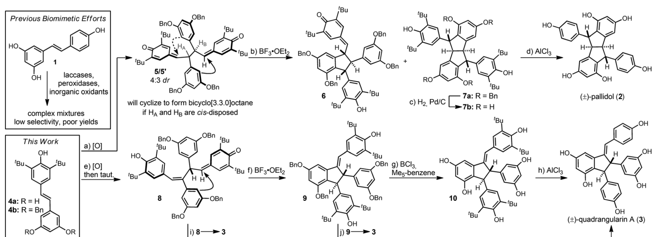
Scheme 1. The total synthesis of pallidol ( 2 ) and quadrangularin A ( 3 ): a) KHMDS (1.05 equiv), [\text{FeCp}_2]\text{PF}_6 (1.05 equiv), THF, 0 °C, 30 min, 95%; b) \text{BF}_3 \cdot \text{OEt}_2 (2 equiv), \text{CH}_2\text{Cl}_2 , -78 °C, 40 min, 88%, 6/7a ca. 1:1; c) Pd/C (30 wt%), \text{H}_2 (1 atm), 3:2 EtOAc/MeOH, RT, 12 h, 95%; d) \text{AlCl}_3 (12 equiv, 2.25 M in \text{CH}_3\text{NO}_2 ), toluene, 60 °C, 30 min, 80%; e) KHMDS (1.25 equiv), 15 min; f) \text{BF}_3 \cdot \text{OEt}_2 (2 equiv), \text{CH}_2\text{Cl}_2 , -78 °C, 5 min, 90% over 3 steps; g) \text{BCl}_3 (12 equiv), \text{Me}_5 -benzene (20 equiv), \text{CH}_2\text{Cl}_2 , -78 °C, 2 h, 82%; h) \text{AlCl}_3 (12 equiv, 2.25 M in \text{CH}_3\text{NO}_2 ), toluene, 60 °C, 30 min, 80%; i) \text{Me}_5 -benzene (40 equiv), \text{AlCl}_3 (25 equiv, 0.6 M in \text{CH}_3\text{NO}_2 ) slow addition, \text{CH}_2\text{Cl}_2 , 0 °C, then 60 °C, 15 min, 51%; j) \text{Me}_5 -benzene (40 equiv), \text{AlCl}_3 (24 equiv, 0.5 M in \text{CH}_3\text{NO}_2 ) slow add'n, \text{CH}_2\text{Cl}_2 , 0 °C, then 60 °C, 1 h, 88%, 5:1 mixture of quadrangularin A ( 3 ) to its internal alkene isomer. Bn = benzyl, t Bu = tert -butyl, taut. = tautomerization, KHMDS = potassium hexamethyldisilazide, [\text{FeCp}_2]\text{PF}_6 = ferrocenium hexafluorophosphate, THF = tetrahydrofuran, \text{Me}_5 -benzene = pentamethylbenzene.
