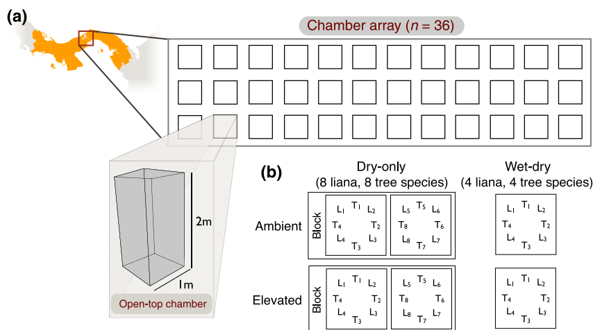
Fig. 1 (a) Open-top chamber array location, layout, and dimensions. (b) experimental design and species distribution among CO 2 treatments and chambers for each experiment. L = liana, T = tree; each subscript number represents a distinct species. Species locations within each chamber for both experiments, and between chambers within block for the dry-only experiment, were randomized before planting.
