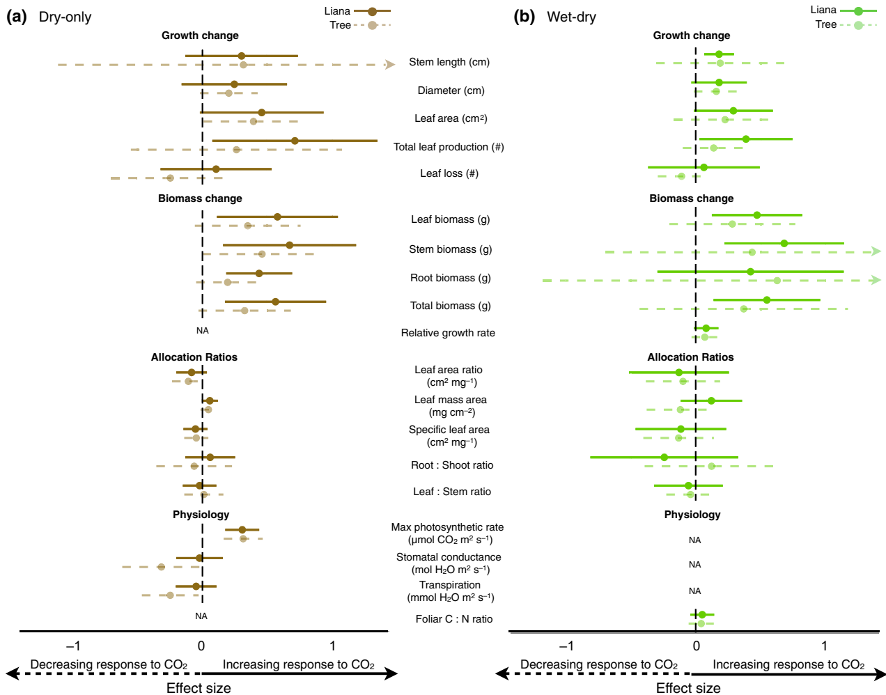
Fig. 2 Effect size response to CO 2 for growth variables, biomass variables, allocation ratios, and physiological variables in the (a) dry-only and (b) wet-dry experiments. Due to the large effect of seasonality on gas-exchange measurements, the wet-dry physiology is presented in Fig 3. Positive/negative effect sizes indicate an increased/decreased response to CO 2 . Points represent the mean effect size; lines represent the 95% confidence interval. Arrows denote confidence intervals that extend beyond the boundaries of the figure.
