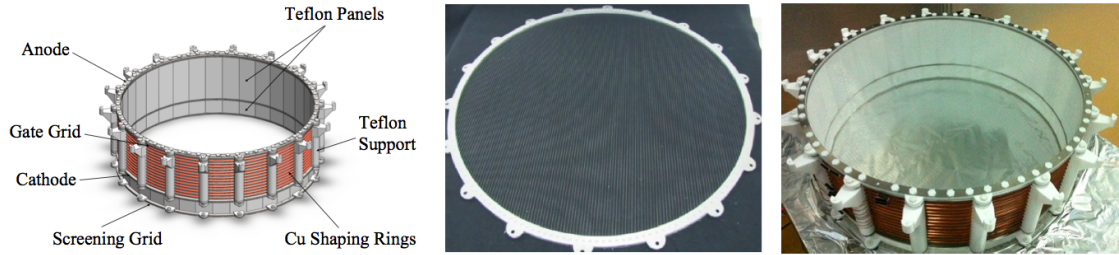
Figure 5.6.3: Left: Schematic of field shaping cage and electrodes. A grounded anode caps the top of the high electric field region, the gate voltage sets the extraction field, and the cathode voltage sets the drift field. A set of 14 field shaping rings sets the voltage boundary conditions to maintain a uniform field in the TPC. Center: Photograph of a gate, cathode, and screening electrode unit formed of parallel 200 \mu\text{m} wires at 5 \text{ mm} pitch. Right: Photograph of assembled electrodes and field cage with cylindrical reflector. Figure from [84].
