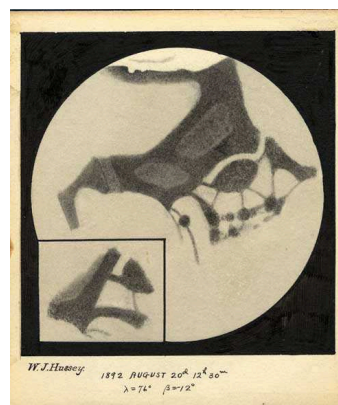
W.J. Hussey's drawing of Mars, 1892. From UM Observatory papers, Box 12.
