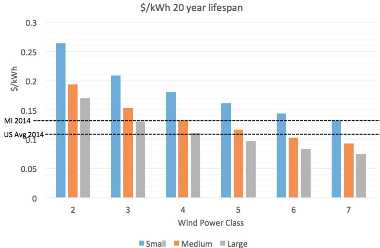
Figure 7: The cost of energy production for turbine use for 20 years, for three sizes of wind turbines. Horizontal dashed lines indicate the average electricity price in Michigan and in the United States. Bars beneath the dashed lines indicate that wind turbines are economically viable with perfect net metering. See Table 4 for Wind Power Class to wind velocity (m/s) conversion.
