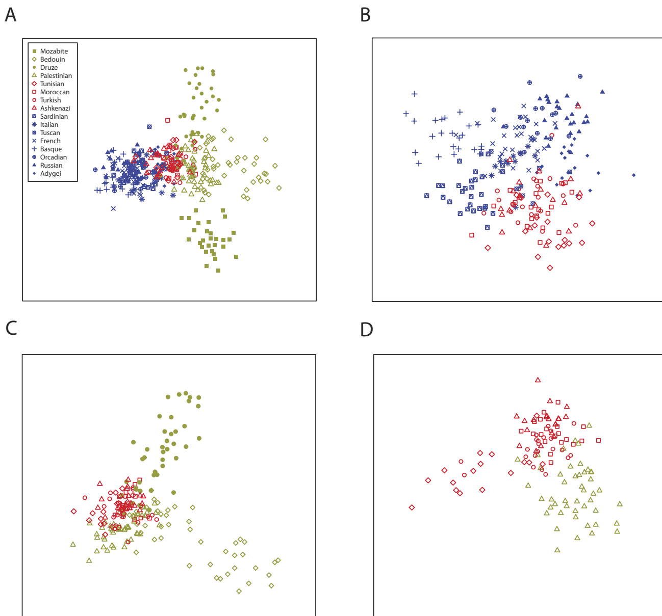
Figure 5 Multidimensional scaling (MDS) analysis of population structure. (a) MDS for European, Jewish, and Middle Eastern individuals. (b) MDS for European and Jewish individuals. (c) MDS for Jewish and Middle Eastern individuals, excluding Mozabites. (d) MDS for Palestinian and Jewish individuals.
