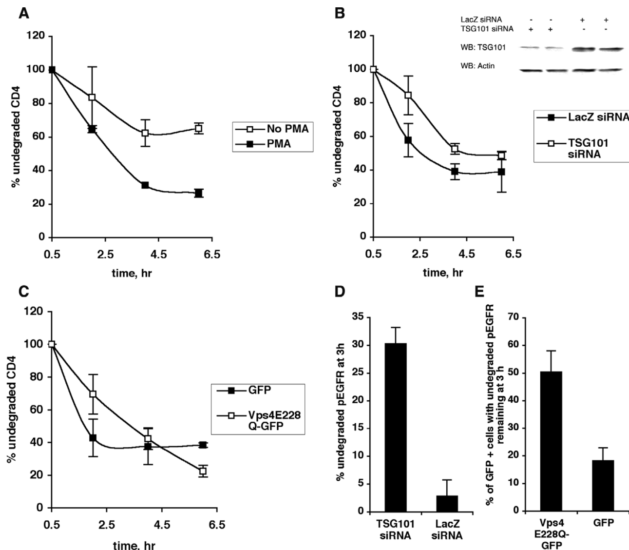
Figure 4 PMA-induced CD4 downregulation is TSG101 and Vps4 independent. (A) COS-1 cells transfected with CD4 were labeled with trans- 35 S-label for 10 minutes, then chased in non-radioactive medium in the presence or absence of 50 ng/ml PMA for the indicated times. At each time point, cells were lysed and radioactive CD4 was analyzed by immunoprecipitation, SDS-PAGE and phosphorimaging. The amount of CD4 remaining at each time point was determined as a percent of the amount of CD4 at the first chase time point, ie 0.5 hours. Data from one representative experiment (out of three) is shown. Error bars represent standard deviation between duplicates for each condition at each time point. (B) COS-1 cells co-transfected with CD4 and siRNA against TSG101 or LacZ were treated as described in (A). Data from one representative experiment (out of four) is shown. Also shown is an immunoblot of TSG101 and actin levels in COS-1 cells co-transfected with CD4 and siRNA directed against either TSG101 or LacZ. (C) COS-1 cells co-expressing CD4 and either GFP or Vps4E228Q-GFP were treated as described in (A). Data from one representative experiment (out of three) is shown. (D) COS-1 cells were transfected with siRNA directed against either TSG101 or LacZ, serum-starved, and treated with 50 ng/ml EGF for 10 min. The cells were then washed, reincubated with fresh media for 0 or 3 hours, lysed and analysed by SDS-PAGE and Western blotting with an anti-pEGFR antibody. The percent of undegraded pEGFR remaining at 3 hour was determined for the two conditions. Error bars represent SD between duplicates for each condition. (E) COS-1 cells were transfected with GFP or Vps4E228Q-GFP, serum-starved, and allowed to internalize EGF for 10 min. The cells were then washed, reincubated with fresh media for 3 hours and analysed for GFP fluorescence, or endogenous phosphoEGFR by immunofluorescence. The percentage of GFP positive cells with pEGFR remaining at 3 hours was determined for the two conditions. Error bars represent SD between duplicates for each condition.
