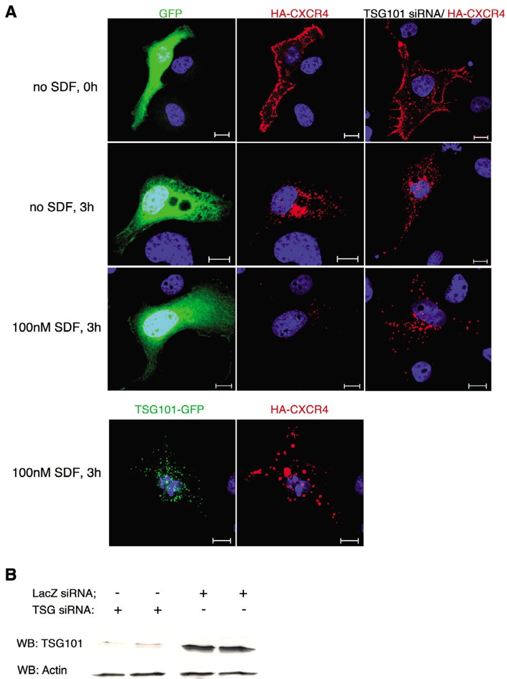
Figure 1 SDF-1 induced CXCR4 downregulation is TSG101-dependent. (A) COS-1 cells co-transfected with HA-tagged CXCR4 and either GFP, TSG101-GFP, or siRNA directed against TSG101, as indicated, were incubated with an anti-HA antibody for 1 hour on ice. Cells were then either fixed and stained with a secondary antibody to detect cell surface CXCR4 (first row), or incubated in DMEM/10% FBS without SDF (second row) or with 100 nM SDF (third and fourth rows) for 3 hours at 37°C prior to fixation, permeabilization and secondary-antibody staining. The cells were then analysed for GFP fluorescence (green), or CXCR4 expression (red). Blue represents nuclear staining. Scale bars = 10 µm. (B) Immunoblot of COS-1 cells co-transfected with HA-tagged CXCR4 and siRNA directed against either TSG101 or LacZ. Top panel, TSG101 Western blot; bottom panel, actin Western blot.
