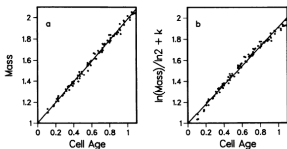
Figure 5 Reanalysis of the data of Kubitschek [16]. At the left is the original data of Kubitschek and at the right is a replotting on logarithmic coordinates. The details are presented in the text.
