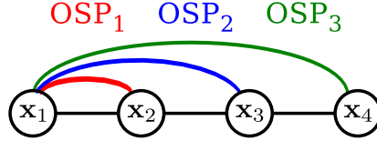
Figure 2.5 Pose-graph over server TOL poses. The OSM algorithm allows the client to reconstruct the underlying server pose-graph (horizontal lines) from the set of received OSPs (colored arcs). Each OSP encodes the transition from \mathbf{x}_1 , which represents the origin state.
