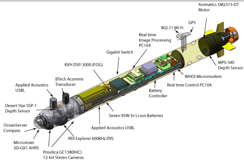
Figure C.1 Schematic Iver2 configuration.
