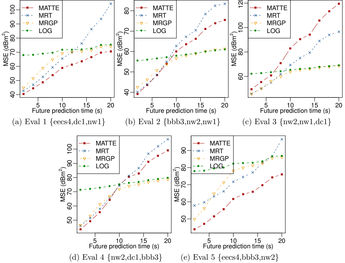
Figure 3.4: Evaluation of signal-strength prediction accuracy. MSE is shown for each method on one of the five testing datasets. Error bars are bounded by 0.8 \text{ dBm}^2 and are omitted for clarity. Our proposed method, MATTE, is compared to extensions of previous methods MRGP and MRT. Our method generally performs better for near-term predictions where the robots’ sensor data provides an informative prior. Poor performance of MATTE in evaluation 3 is attributable to the randomly generated training set which contains only indoor datasets, while the testing set contains both indoor and outdoor sets.
