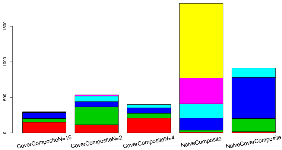
Figure 2.5: Phase 2 cumulative runtimes. Color bands indicate the portion of rasterizations that finished in <1.0s, <2.0s, <3.0s, <4.0s, <5.0s and \geq 5.0 s for colors of red, green, blue, cyan, magenta and yellow, respectively.
