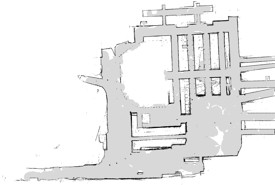
Figure 2.4: Phase 2 occupancy grid. This grid map includes data from 15 robots collected over the course of 72 minutes. Size: 220 x 160 m @ 0.1m resolution.
