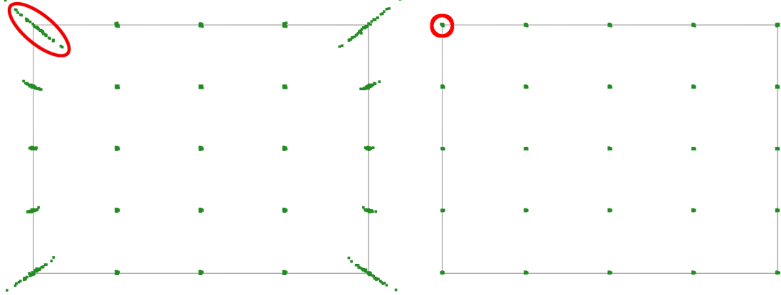
Figure 5.2: Max Expected Reprojection Error. The ERE for several test points is computed by sampling from the estimated model parameter distribution, and reprojecting world points to derive pixel-based error measurements. The resulting pixel error distributions are shown after 3 and 5 images have been taken by the user. The set of samples with the Max ERE are circled in red. Our sampling-based error metric can be used with any intrinsics model and allows us to automatically ensure the calibration is well constrained everywhere without requiring the user to collect a test set.
