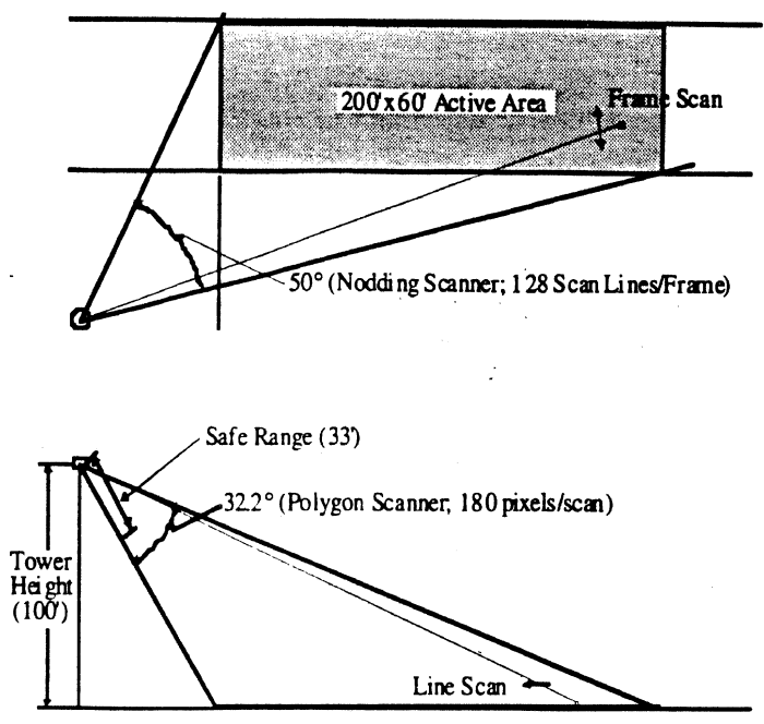
Figure 4-2. Viewing Geometry of the VME-MS
