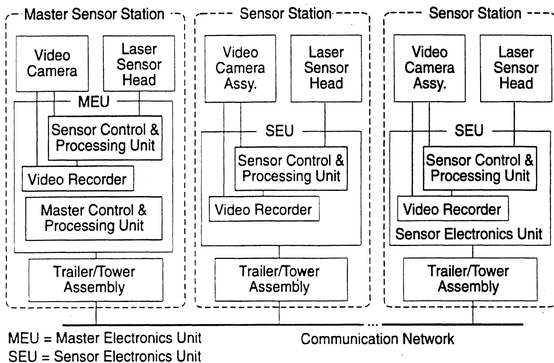
Figure 4-4. VME-MS Architecture
