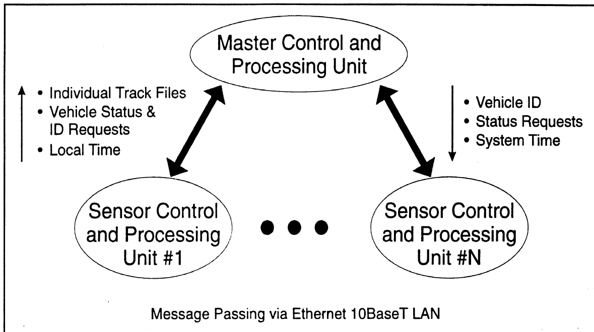
Figure 7-4. System Functionality.
