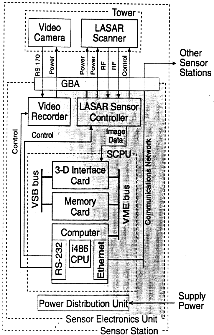
Figure 4-12. Sensor Station
