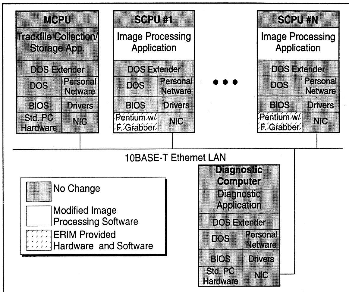
Figure 7-3. Video-based VME-MS System Configuration.
