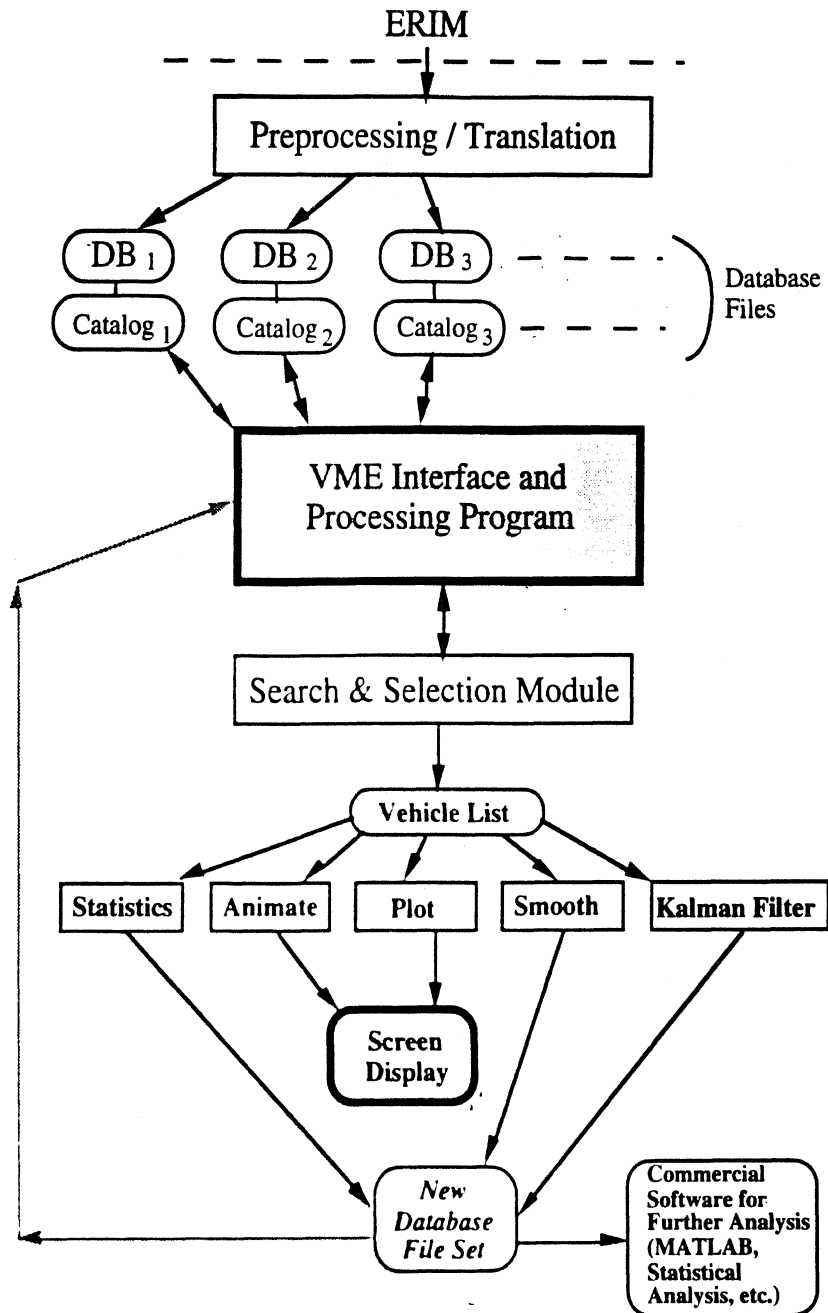
Figure 4-19. Basic Concept of VME Software & Processing Flow.
