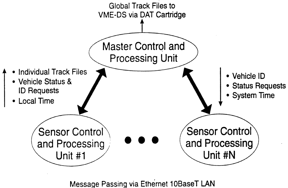
Figure 4-5. SCPU <-> MCPU Communications
