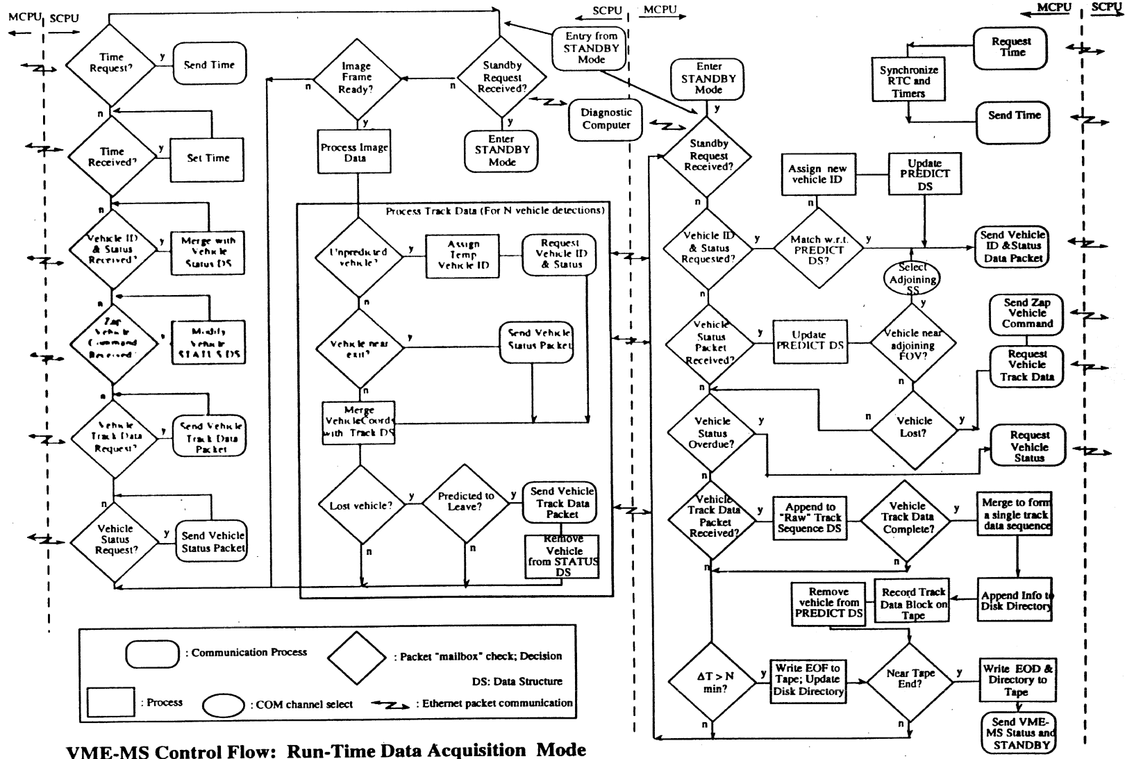
Figure 4-17. Control Flow in Run-Time Data Acquisition Mode.
