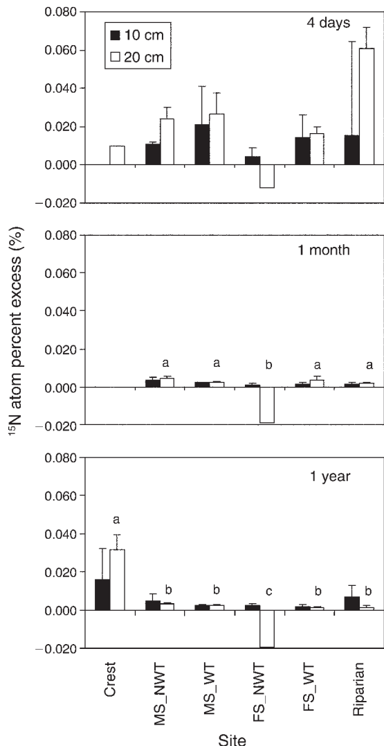
FIG. 3. 15 N atom percent excess (the excess percentage of 15 N atom percent relative to the reference level) in soil pore water collected by micro-lysimeters during the first year. Data for samples collected at 4 days, 1 month, and 1 year are shown; error bars indicate +SE ( n = 2). Lysimeters were installed at 10 and 20 cm depths. Different lowercase letters indicate significant difference by one-way ANOVA ( P < 0.05) across sites within the same depth (differences were significant only for 20-cm samples). Abbreviations are as follows: MS, Midslope; FS, Footslope; NWT, non-water tracks; WT, water tracks.
