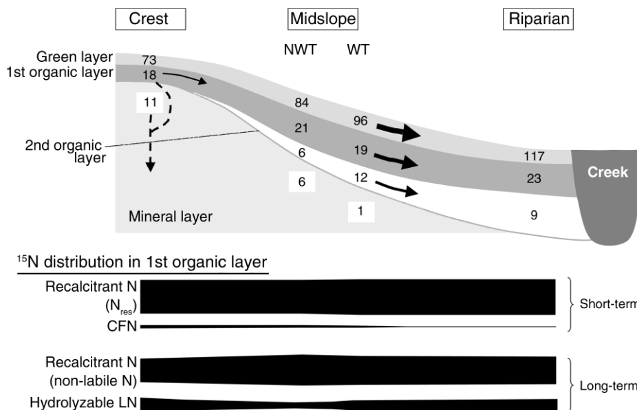
FIG. 9. Conceptual models of initial ^{15}\text{N} retention and subsequent movement along the hillslope of Innavait Creek watershed along with short- and long-term ^{15}\text{N} distribution in soil. The values indicate average short-term recovery of ^{15}\text{N} (percentage of added) within each green or soil layer. Footslope sites were omitted for simplicity. The solid arrows indicate subsequent movement of ^{15}\text{N} via water flowing downslope, and the dashed arrows show possible pathways of ^{15}\text{N} leaching. The width of arrows indicates relative magnitude of ^{15}\text{N} movement. The bars at the bottom show short- and long-term ^{15}\text{N} distribution within the first organic layer among various N pools across the sites along the hillslope. The width of the bars indicates the contribution of each pool to ^{15}\text{N} retention relative to other pools. N_{res} is residual N after chloroform-fumigation extraction; CFN is chloroform-fumigation extractable N; hydrolyzable LN is total hydrolyzable labile N (hydrolyzable \text{NH}_4^+ , amino acids, and amino sugars); non-labile N is total ^{15}\text{N} recovered in the first organic layer (100%) – total hydrolyzable LN.
