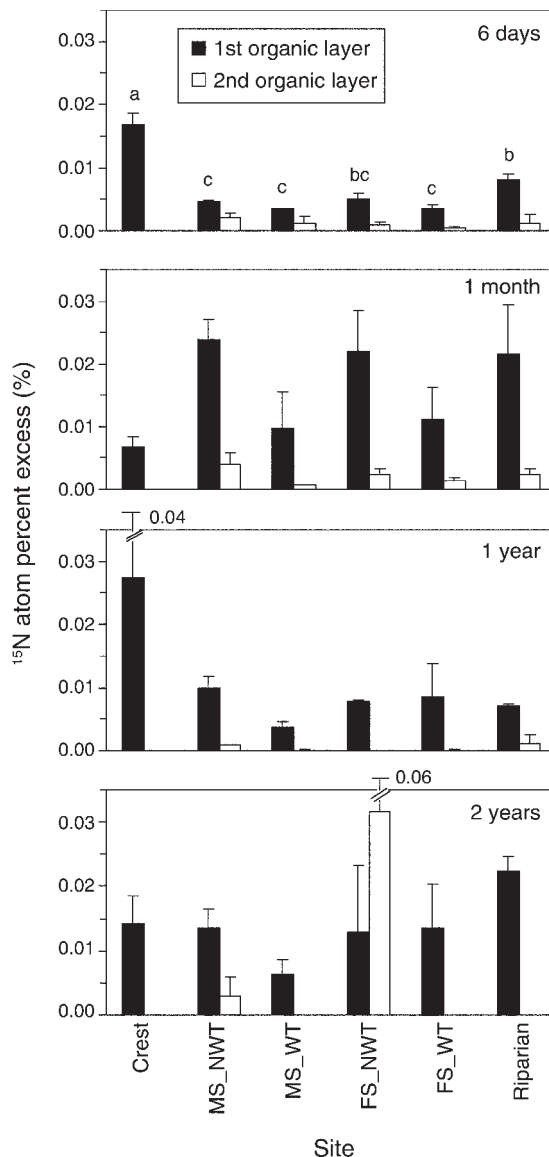
FIG. 4. 15 N atom percent excess in water-extractable dissolved-N pool during the first two years. Data shown are soil extracts for 6 days, 1 month, 1 year, and 2 years; error bars indicate +SE ( n = 2). The first and second organic layers are those shown in Fig. 2. Note that all extraction was done at a soil : water ratio of 1:10, except for the second organic layer collected at 6 days and 1 month, for which a soil : water ratio of 1:5 was used. Abbreviations are as follows: MS, Midslope; FS, Foothlope; NWT, non-water tracks; WT, water tracks.
