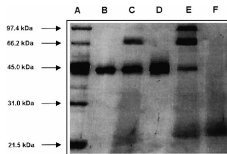
Fig. 1. Silver-stained SDS-PAGE of wild-type TGT and TGT(S103A) in the absence or presence of tRNA Tyr -(G 34 ). Lane A, molecular mass standards; lane B, TGT (wt); lane C, TGT (wt)+tRNA; lane D, TGT(S103A); lane E, TGT(S103A)+tRNA; lane F, tRNA.
