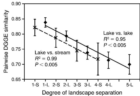
FIG. 5. Mean pairwise similarity values for DGGE banding patterns plotted against the degree of landscape separation. This separation is a categorical variable representing the number of upstream lakes or inlets separating two sites; x-axis values of 1-L mean that comparisons are made between a lake and its closest upstream lake, and 1-S compares a lake and its closest inlet stream; x-axis values of 2 represent a separation of two upstream lakes or two lake inlets. Error bars indicate \pm SE of all possible combinations within a category.
