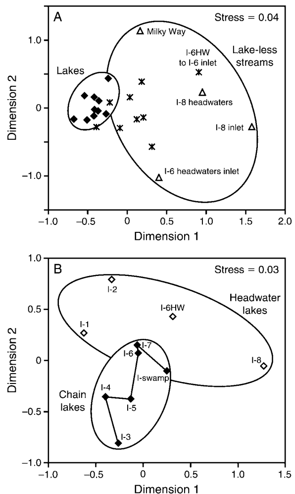
FIG. 3. Multidimensional scaling ordinations (with values of normalized stress) of pairwise estimates of similarity (Dice) calculated from DGGE banding patterns of DNA samples collected 6–7 August 2002. (A) Comparisons among all samples. Symbols indicate lakes (solid diamonds), connecting streams (stars), and lake-less streams (open triangles). (B) Comparisons among lakes only. Symbols indicate flow-through chain lakes (solid diamonds) and headwater lakes (open diamonds). Chain lakes are connected with a line.
