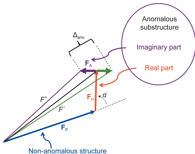
Figure 1 Diagram of the relationships between structure factors and anomalous differences. Structure factors corresponding to an acentric reflection with indices (h, k, l) and to its Bijvoet mate with indices (-h, -k, -l) are given. The structure factors for the Bijvoet mate are reflected across the x axis for clarity in presentation. The structure factor for the non-anomalous atoms in the structure is designated as F_P . The part of the structure factor originating from the real part of the form factor for the atoms in the anomalous substructure ( f^{\circ} + f' ) is shown as F_H and the part of this structure factor coming from the imaginary part of the form factor ( if'' ) is shown as F_A .
