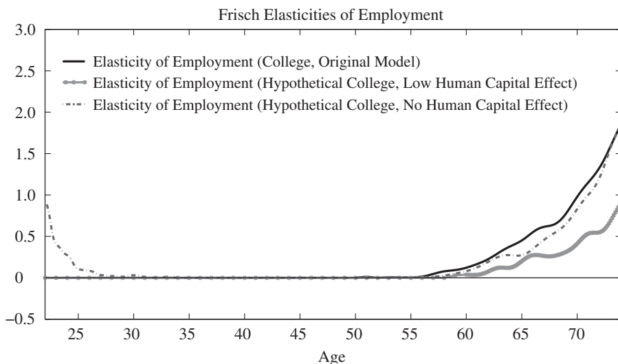
Fig. 19. Effect of Human Capital – Frisch Elasticity – Extensive Margin
