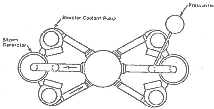
Figure 6-10: Various types of PWR NSSSs from U.S. Reactor Vendors
