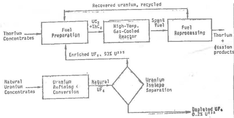
High-Temperature Gas-Cooled Reactor
