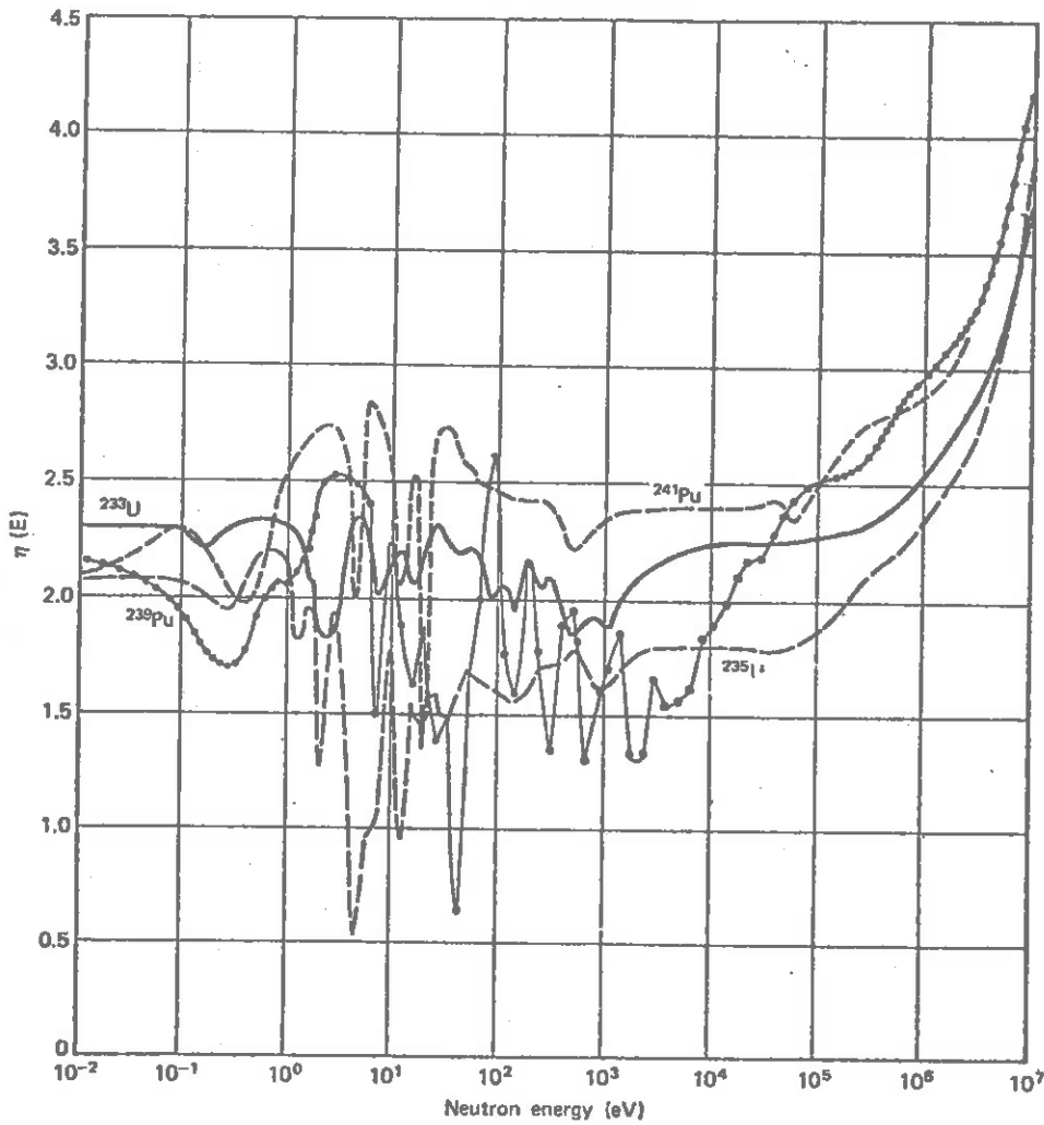
Variation of \eta with energy for ^{233}\text{U} , ^{235}\text{U} , ^{239}\text{Pu} and ^{241}\text{Pu} .
