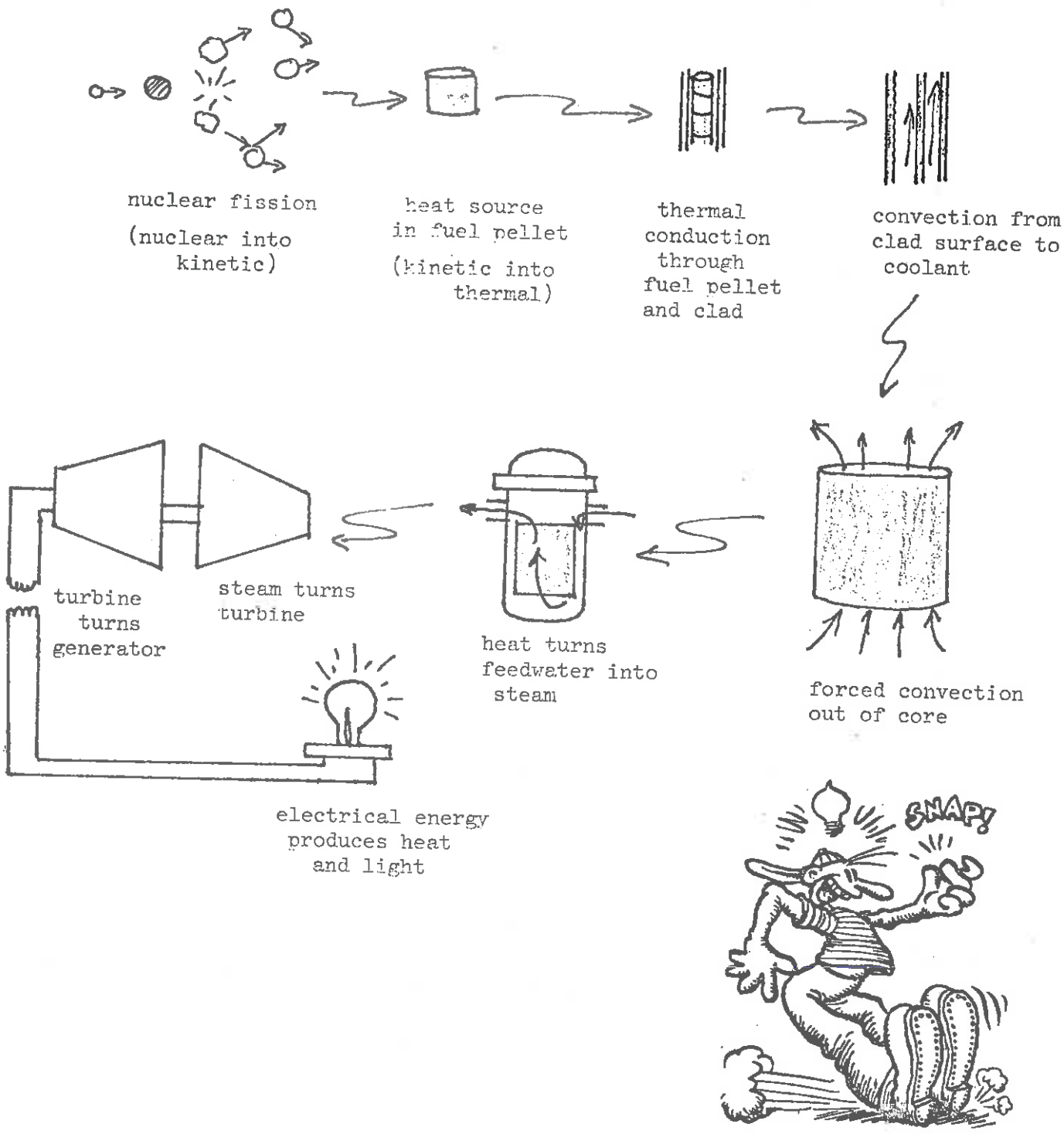
Figure 3-1: The Energy Transformations Involved in Nuclear Power
