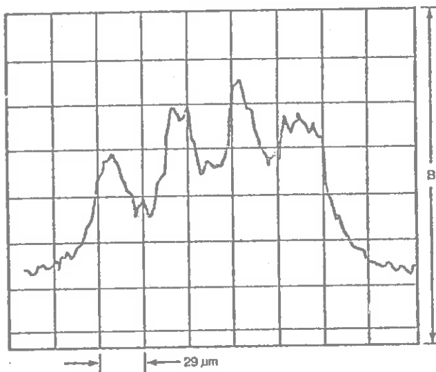
Fig. 5. Image-intensified x-ray pinhole photographs, shown with corresponding diametric microdensitometer traces, were obtained during compression of (top) unfilled spherical glass shell with outside diameter of 120 micrometres, wall thickness 1 micrometre, and (below) DT-filled (30 atm) spherical glass shell with 117-micrometre outside diameter, 0.7-micrometre wall.
