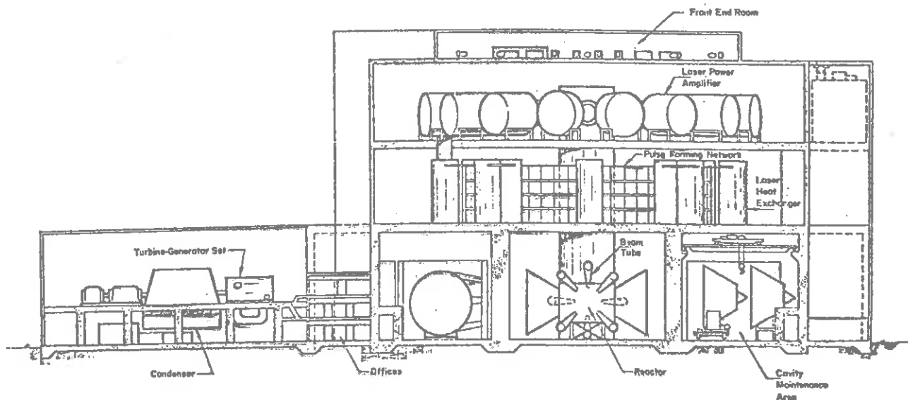
Electric generating station utilizing magnetically protected laser-fusion reactors and CO 2 laser technology
