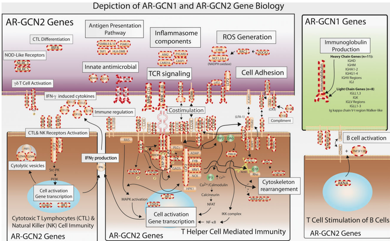
Figure 4: Biological functions of clinical acute rejection–gene coexpression network 1 (AR-GCN1) and AR-GCN2 genes. The figure illustrates the biological functions of 107 (56%) of the AR-GCN2 (immune response/inflammation) genes and all 31 of the AR-GCN1 (B cell/immunoglobulin production) genes. The genes in the illustration with dashed red border are present in the GCNs. It is important to note that these genes are essentially the same in IFTA-GCN2.
