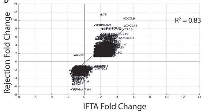
Figure 2: Differentially expressed genes shared between IFTA and AR. (A) Venn diagram showing differentially expressed genes (DEGs) shared between interstitial fibrosis and tubular atrophy (IFTA) without inflammation and clinical acute rejection (AR). (B) Plots the differential fold changes in gene expression (DEGs) comparing IFTA without inflammation versus AR. A linear regression line and R 2 statistic demonstrates a highly concordant direction of gene expression between phenotypes; (C) and (D) repeat and validate the analysis using an independent, external dataset. Note 1: Differentially expressed genes and fold changes are calculated in relation to normal transplants (TX) defined by stable function and light histology. Note 2: The subphenotypes of IFTA with and without inflammation were not available for the external data set.
