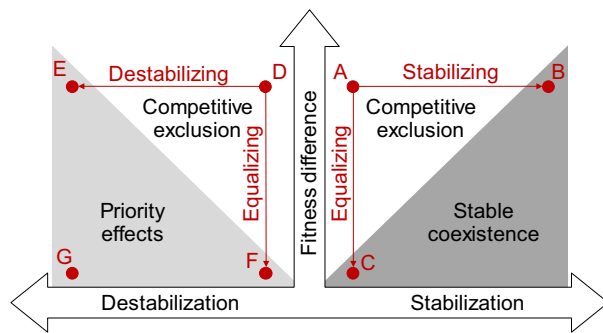
Fig. 1. Theoretical framework describing mechanisms of stable coexistence and priority effects. The x-axis quantifies the strength of stabilization or destabilization. In stabilization, a species' per capita growth rate is negatively related to its abundance relative to the other species. In destabilization, it is positively related. The y-axis quantifies fitness difference between species. Each dot marked with a letter represents a hypothetical pair of species interacting with each other at a local site (see text for detail). Modified from Mordecai (2011).
