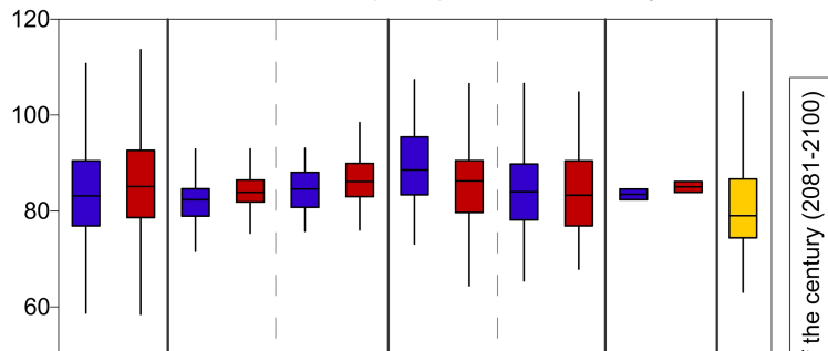
Extreme 24 h precipitation, RP=10 years
