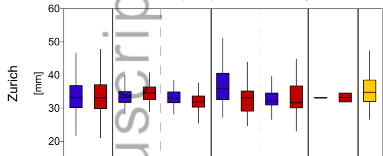
Extreme 1 h precipitation, RP=10 years
