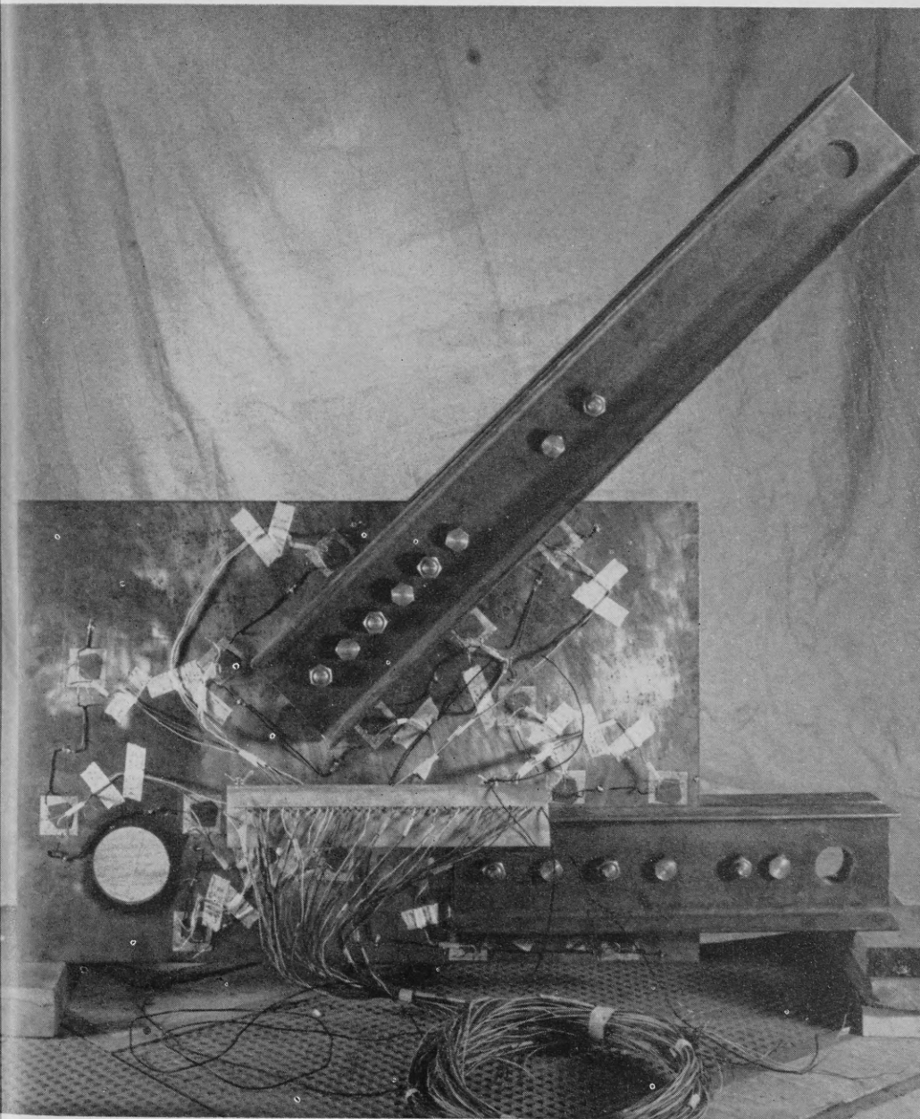
Electric strain gages measuring stresses in connection plate of steel truss, Civil Engineering
