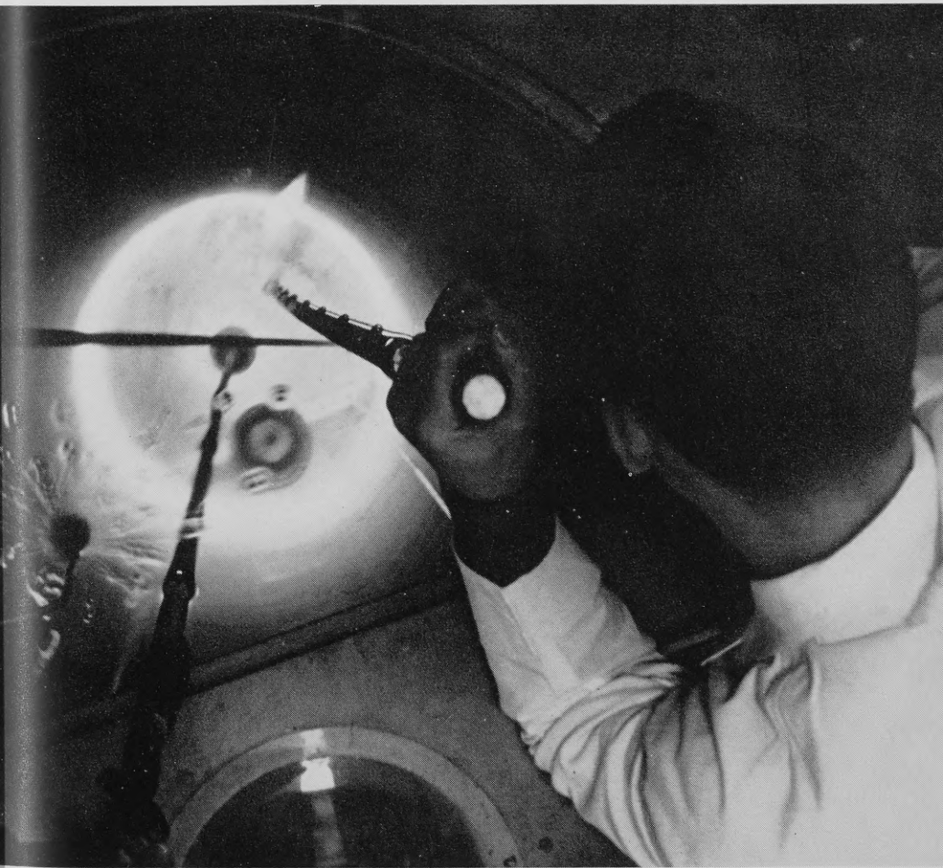
Loading cobalt-60 rods in gamma radiation source at the bottom of a 16-foot well
