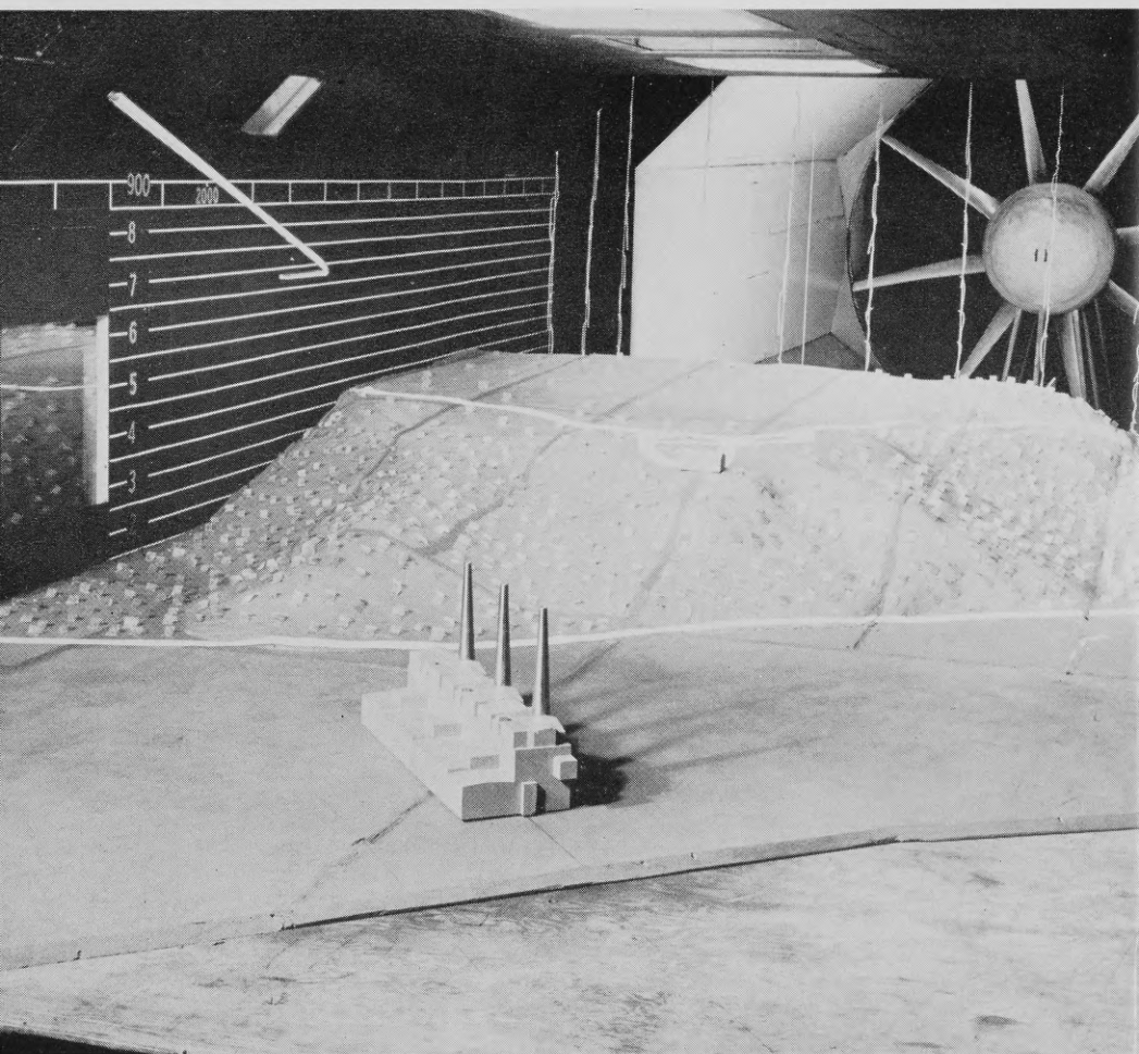
Air-pollution studies in a wind tunnel
