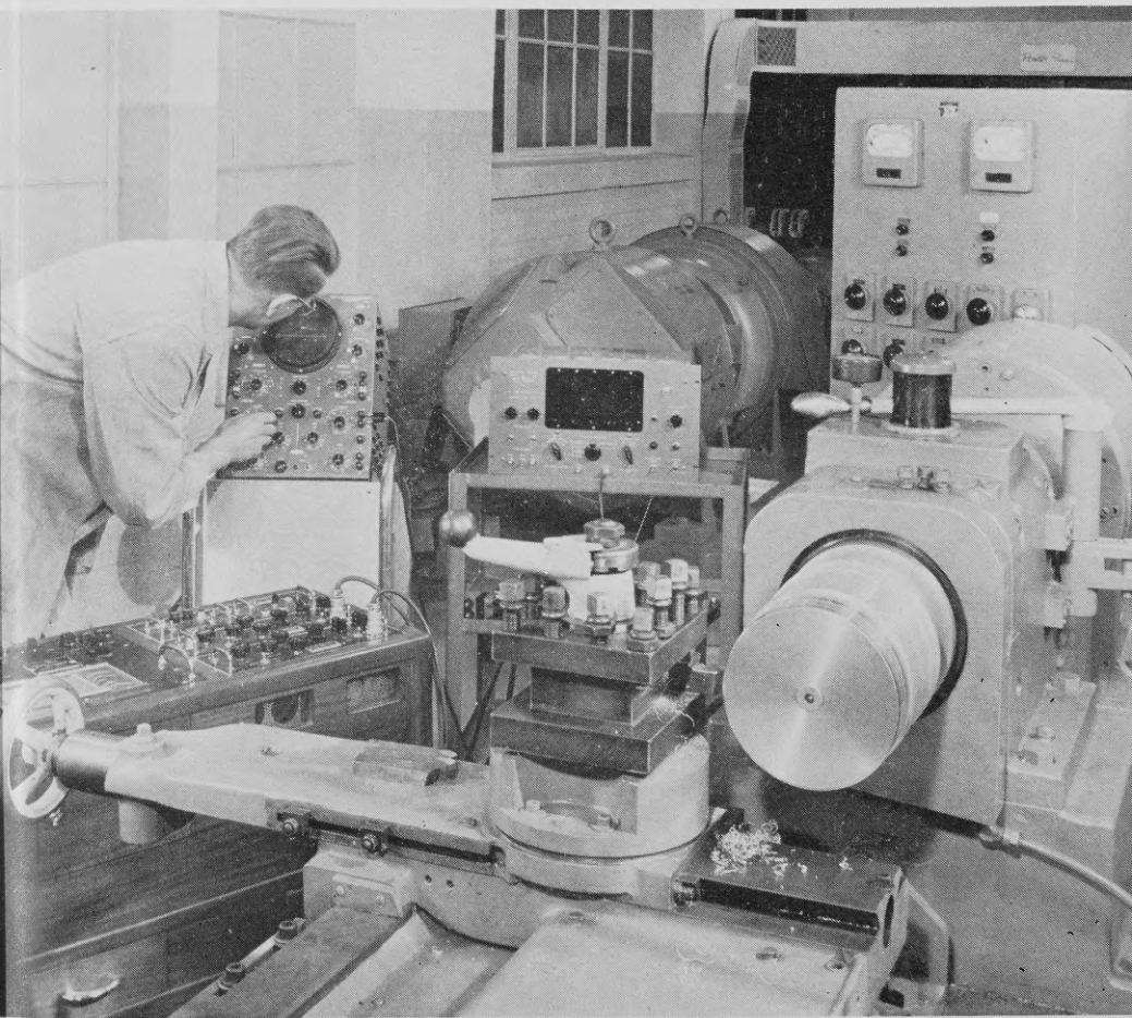
A 300-horsepower lathe which operates at speeds up to 10,000 revolutions a minute
