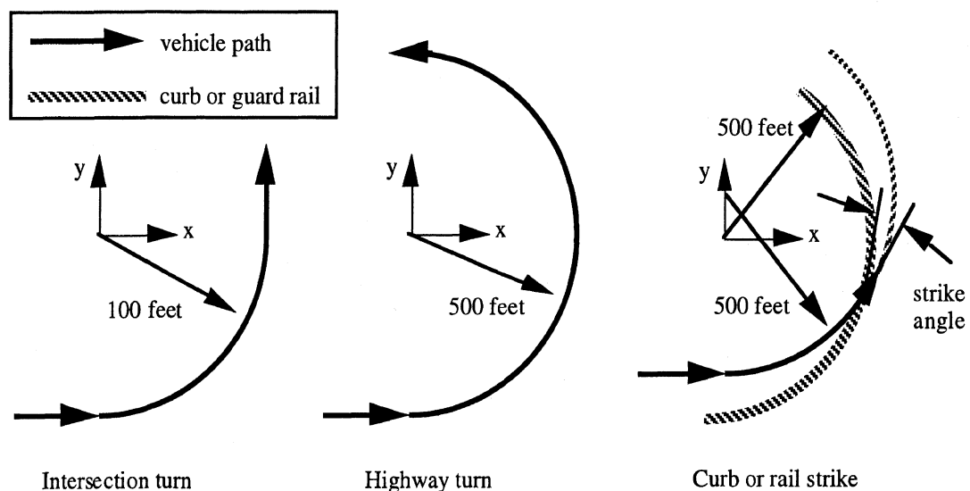
Figure 7. Closed-loop simulated maneuvers
