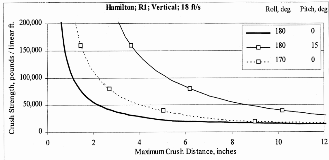
Figure C-11. Vertical results for Hamilton with flat rails and flat end dams only.
