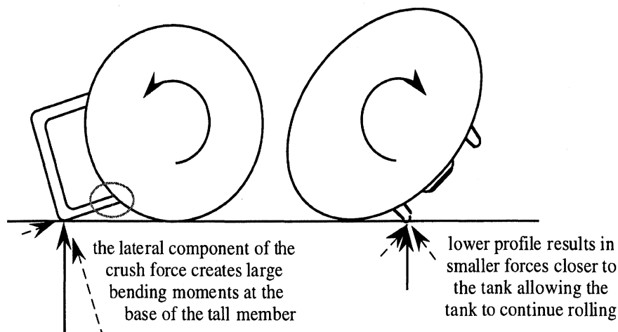
Figure 37. Forces on the protectors during rolling impact
