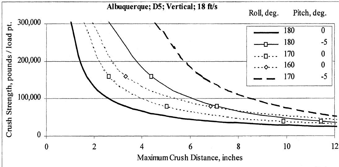
Figure C-6. Vertical results for Albuquerque with staples every 4 ft.
