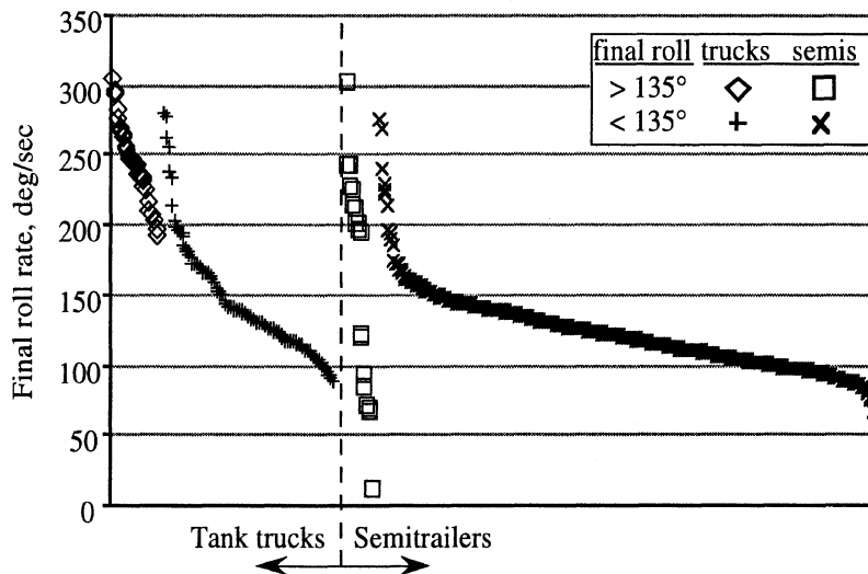
Figure 24. Final roll rates of the tank units
