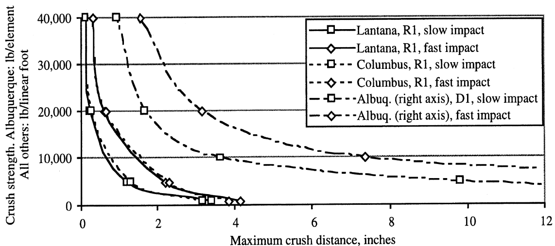
Figure 36. Rolling-impact results for the semitrailers in their as-designed configurations
