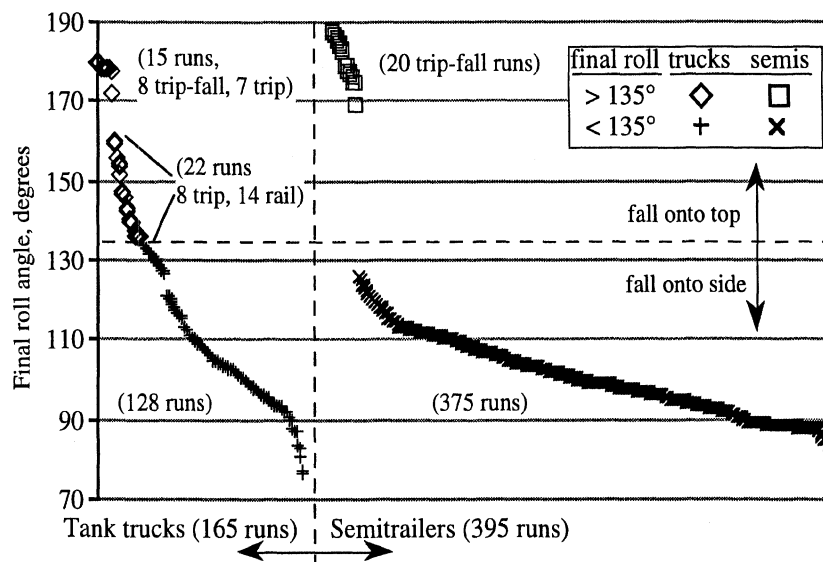
Figure 20. The final roll angle for all successful simulated test runs
