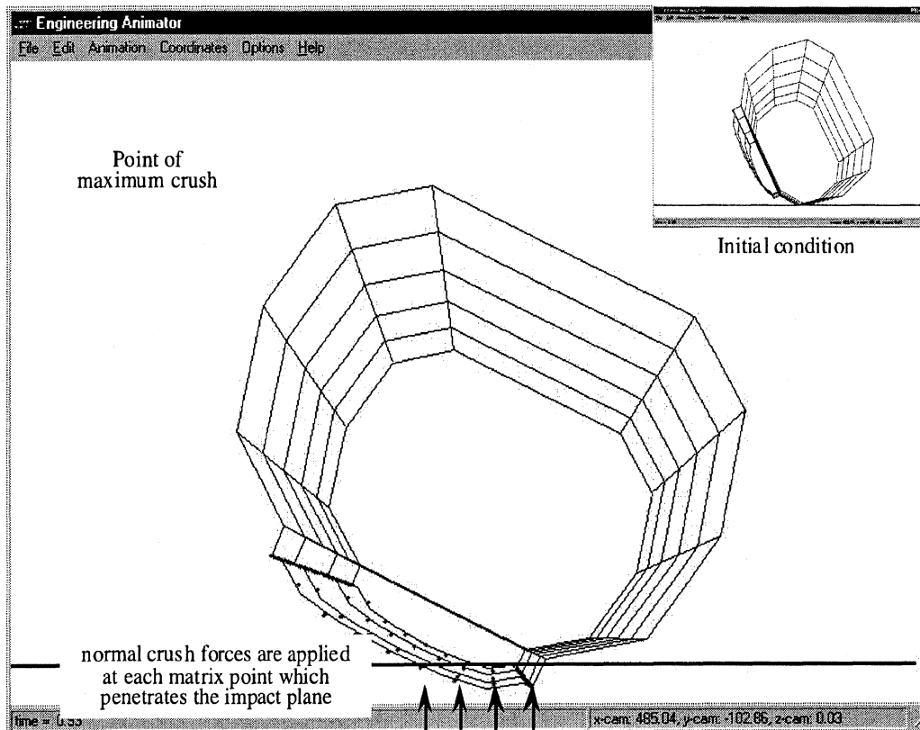
Figure 31. Animation frames from a simple run of the rolling-impact model
