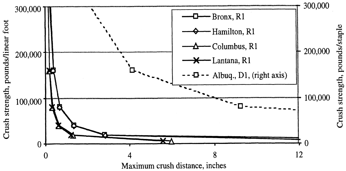
Figure 42. Comparison of results from the as-design vehicles in 12-ft/sec impacts, flat against the top
