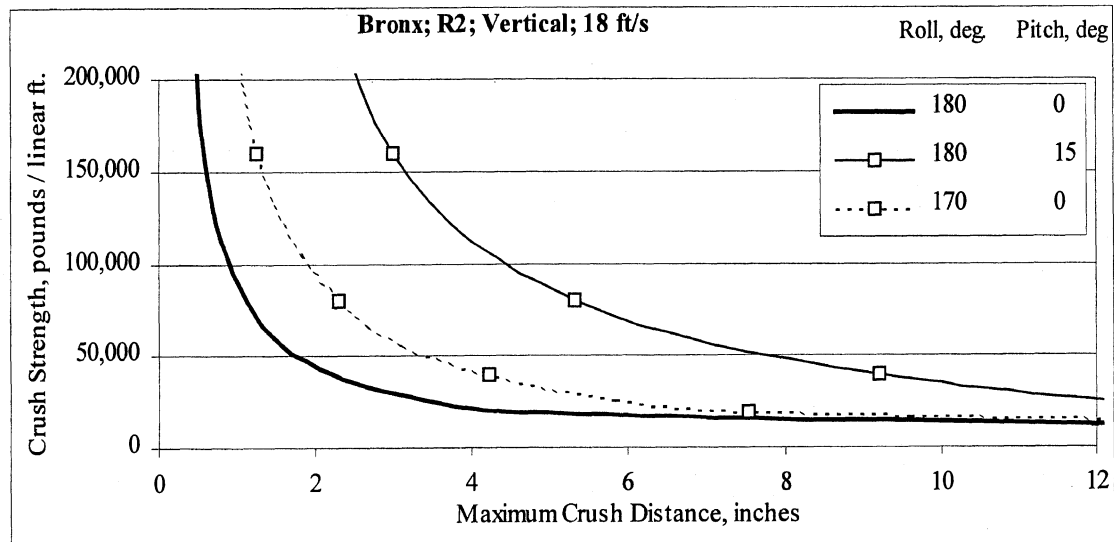
Figure C-9. Vertical results for Bronx with flat rails and flat dams every 6 ft
