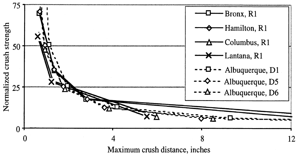
Figure 44. The impact data of figure 43 presented in normalized form
