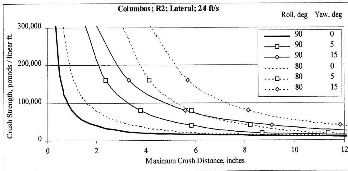
Figure C-30. Lateral results for Columbus with flat rails and flat end dams every 6 ft.
