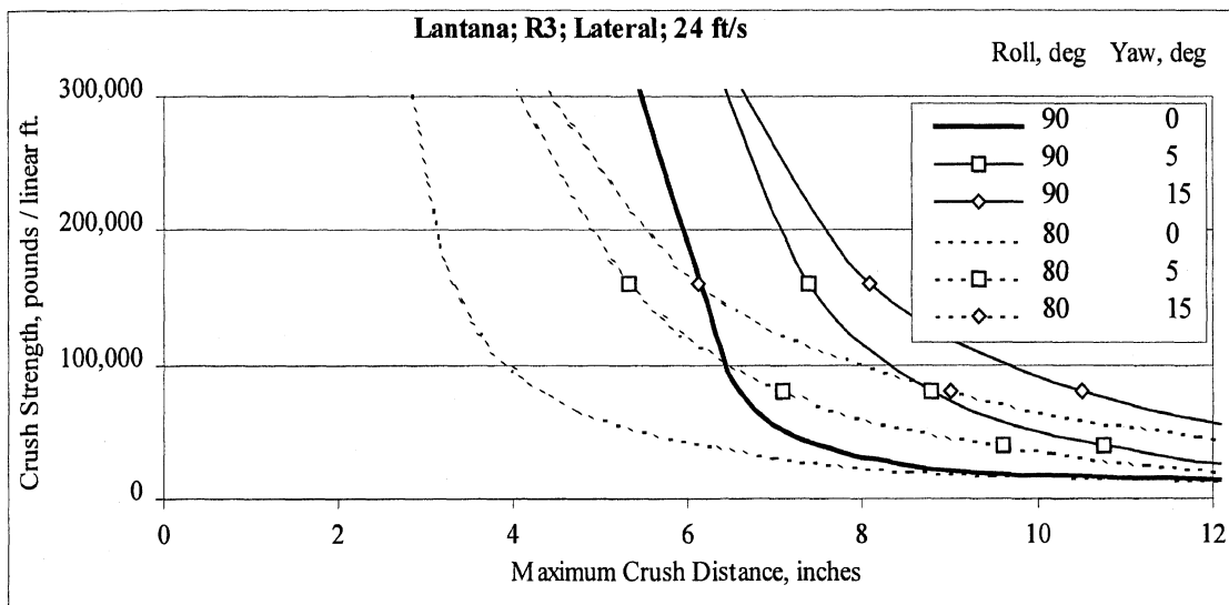
Figure C-34. Lateral results for Lantana with flat rails and crowned dams every 6 ft.
