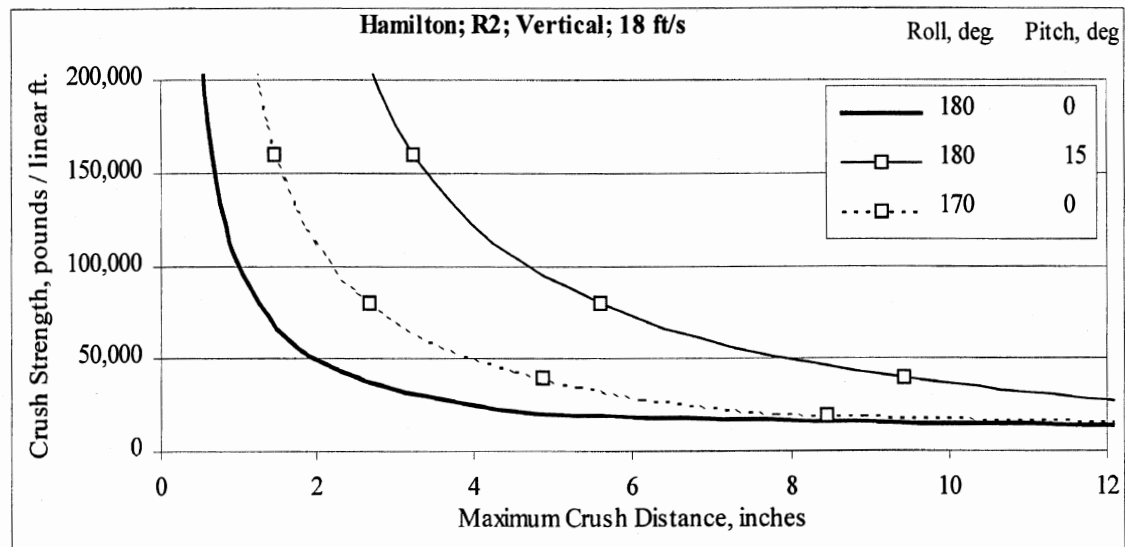
Figure C-12. Vertical results for Hamilton with flat rails and flat dams every 6 ft.
