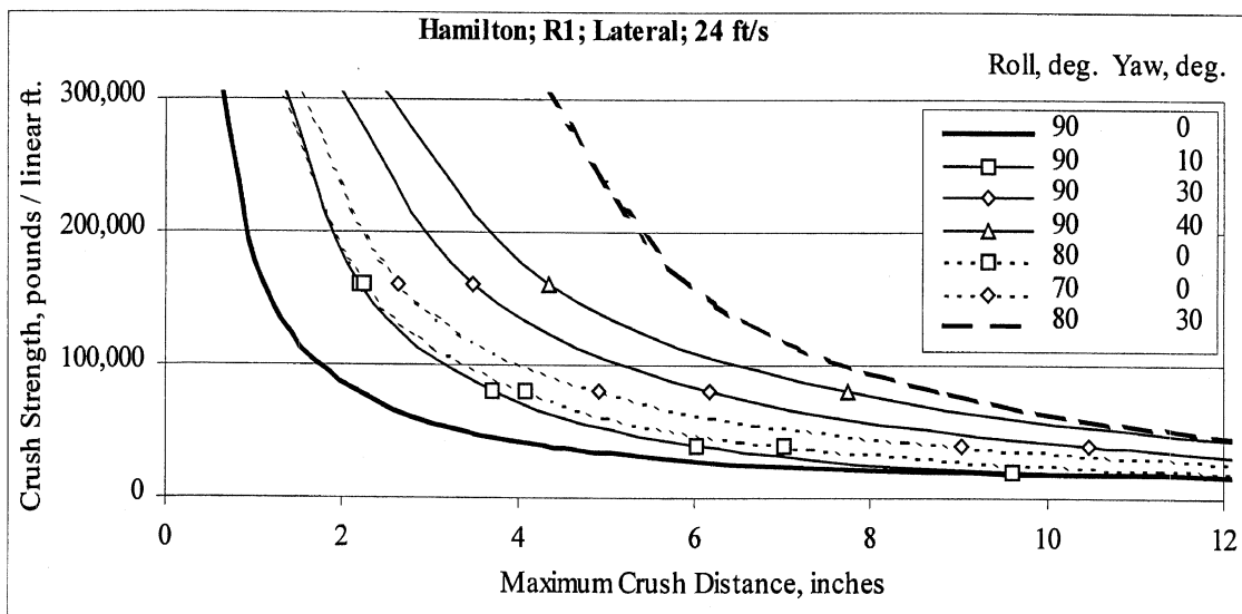
Figure C-26. Lateral results for Hamilton with flat rails and flat end dams only.
