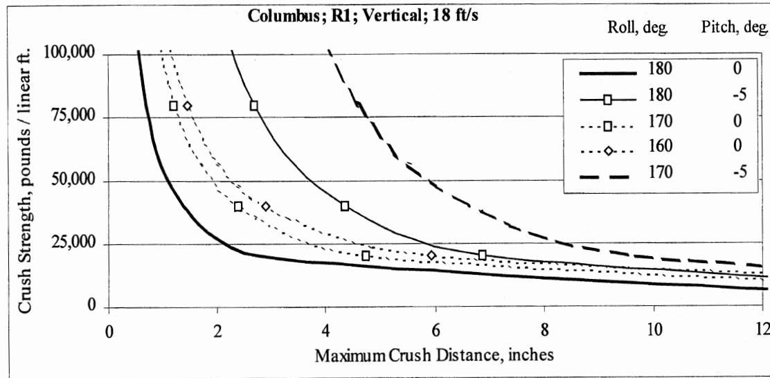
Figure C-14. Vertical results for Columbus with flat rails and flat end dams.
