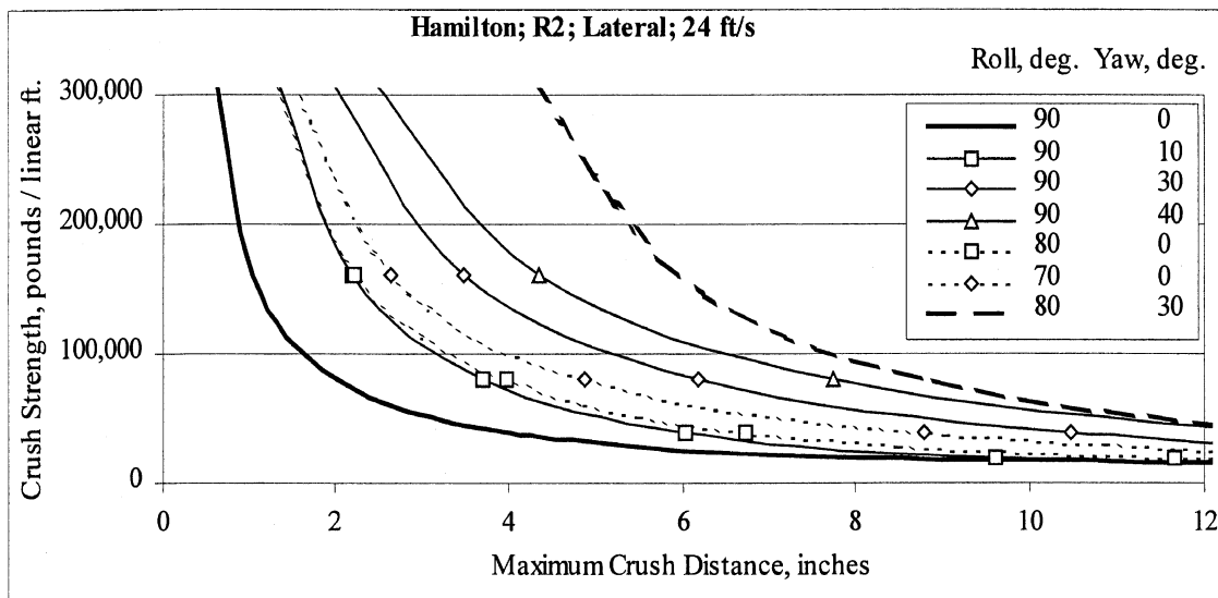
Figure C-27. Lateral results for Hamilton with flat rails and dams every 6 ft.
