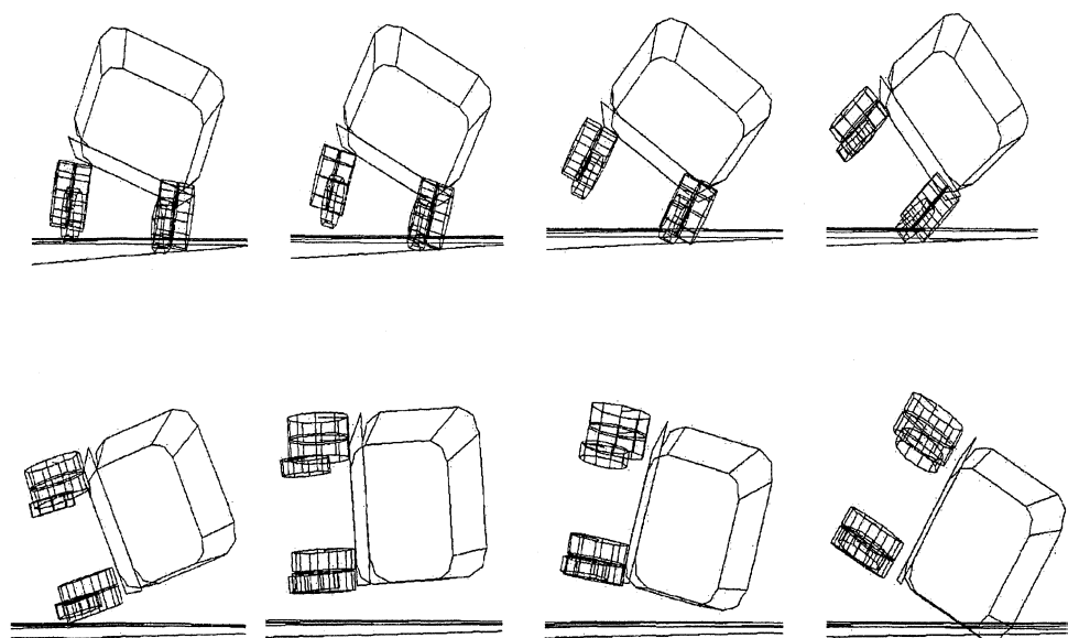
Figure 12. The Hamilton vehicle in a rapid, flat-surface rollover (run #63, \Delta t=0.1 sec)
