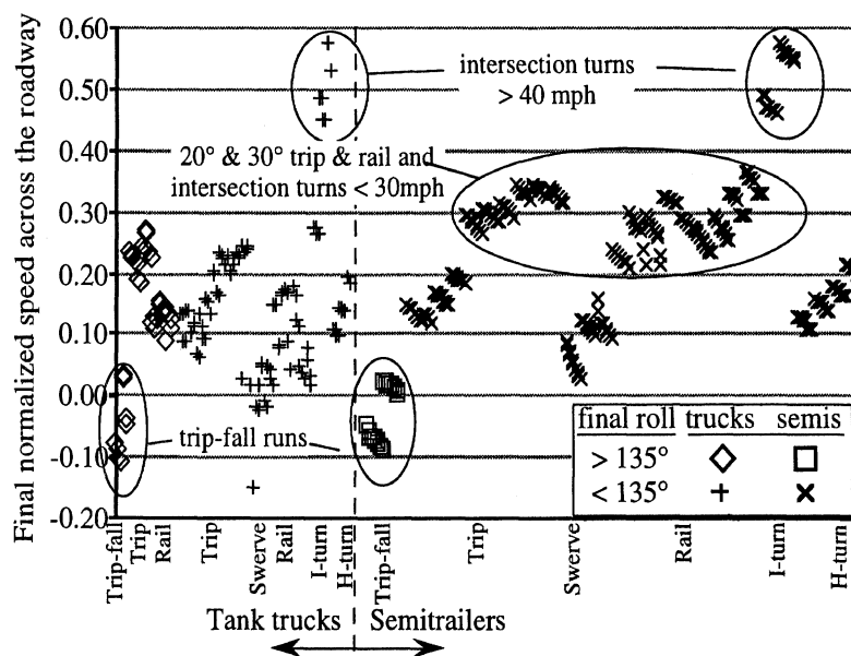
Figure 26. Final speed of the tank units across the roadway grouped by maneuver
