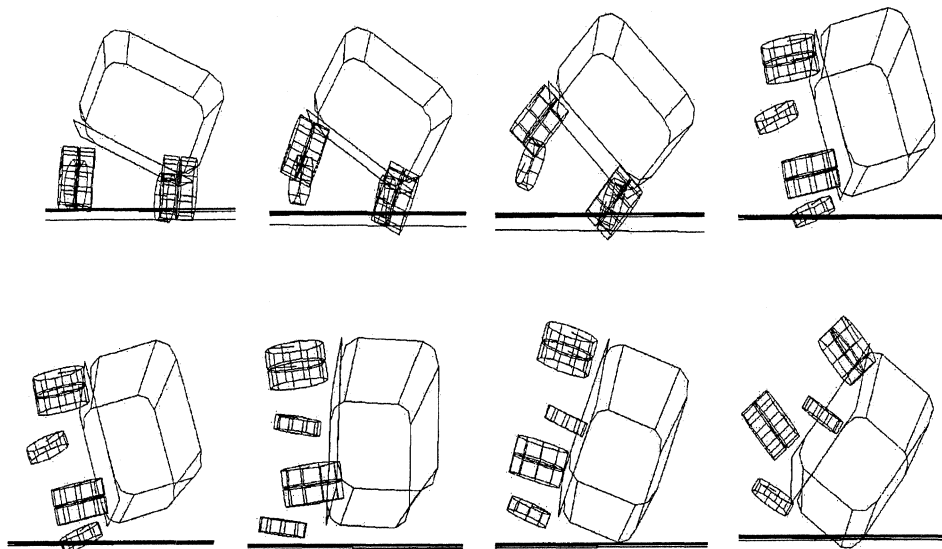
Figure 16. The Hamilton vehicle rolling over after striking a rail(run #52, \Delta t=0.1 sec)
