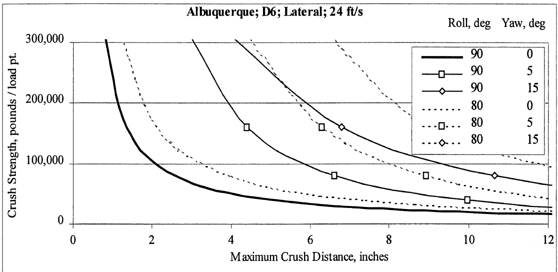
Figure C-22. Lateral results for Albuquerque with staples every 2 ft.
