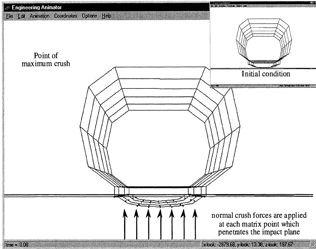
Figure 30. Animation frames from a simple run of the normal-impact model
