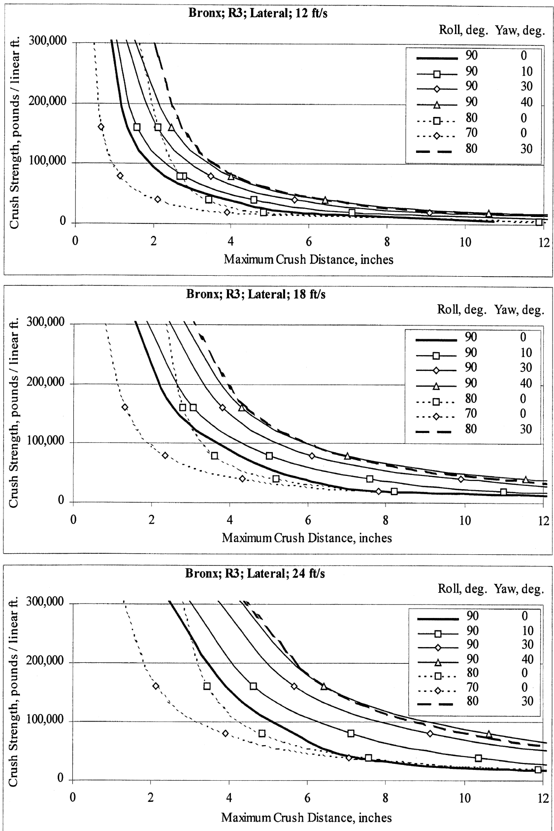
Figure C-25. Lateral results for Bronx with flat rails and crowned dams every 6 ft.
