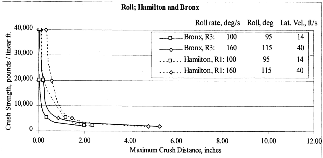
Figure C-3. Roll results for Bronx and Hamilton simulation.
