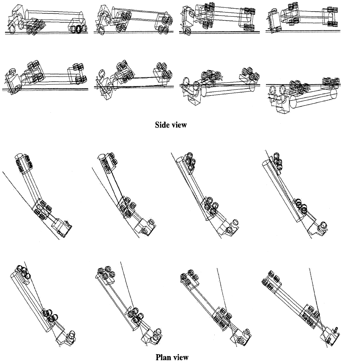
Figure 18. The Albuquerque vehicle rolling over and falling after striking a curb at 20 degrees and 45 mph (run #124)
