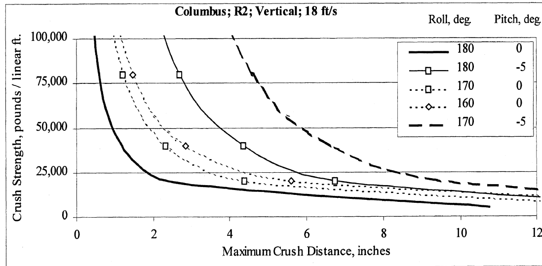
Figure C-15. Vertical results for Columbus with flat rails and flat dams every 6 ft.
