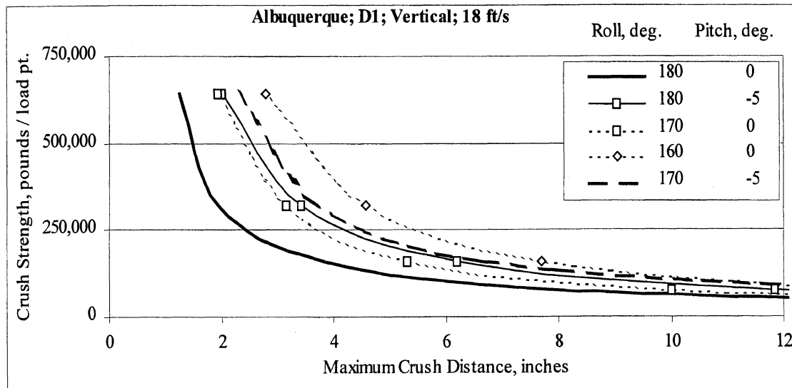
Figure C-5. Vertical results for Albuquerque as designed
