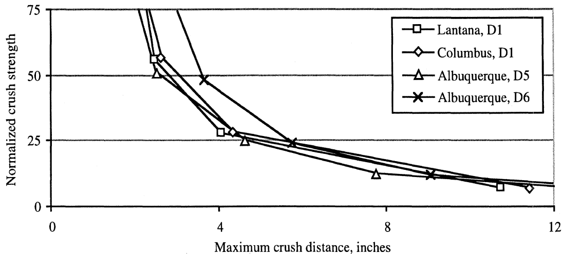
Figure 45. Results from impacts at 12 ft/sec and -5 degrees of pitch presented in normalized form
