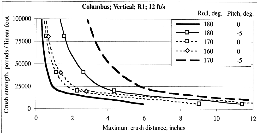
Figure 34. Example results from the impact simulation study
