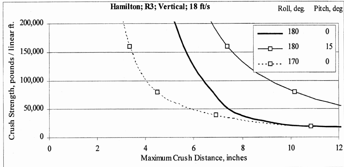
Figure C-13. Vertical results for Hamilton with flat rails and crowned dams.
