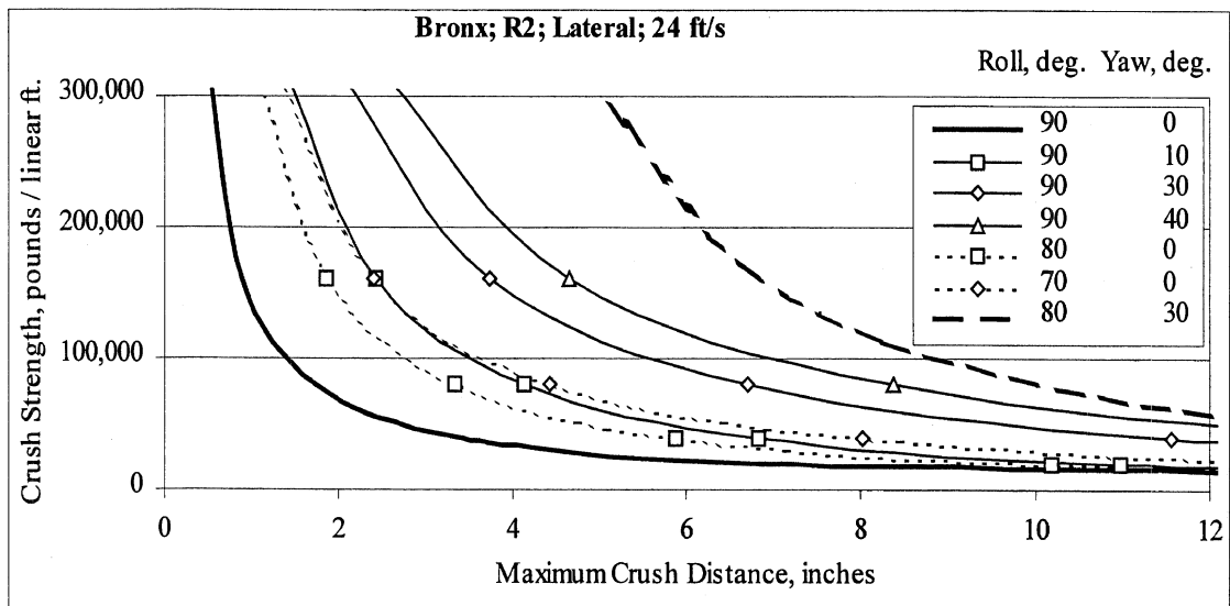
Figure C-24. Lateral results for Bronx with flat rails and flat dams every 6 ft.
