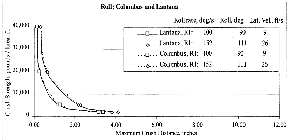
Figure C-4. Roll results for Columbus and Lantana simulation
