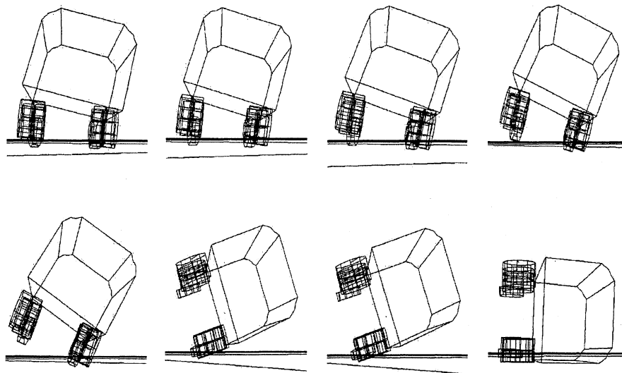
Figure 10. The Bronx vehicle in a minimal rollover (run #116, \Delta t = 0.25 sec)
