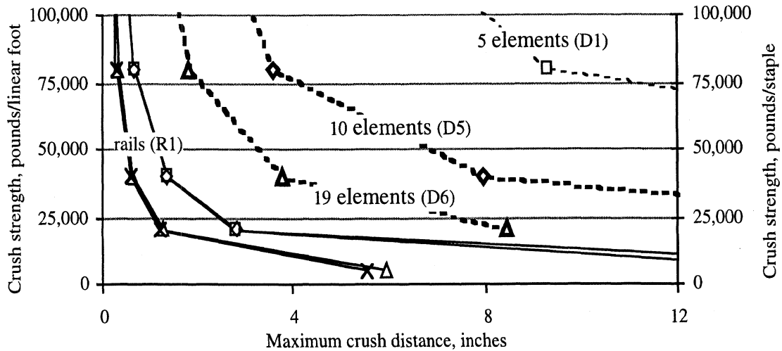
Figure 43. The performance of discrete elements approaches that of rails as their numbers increase
