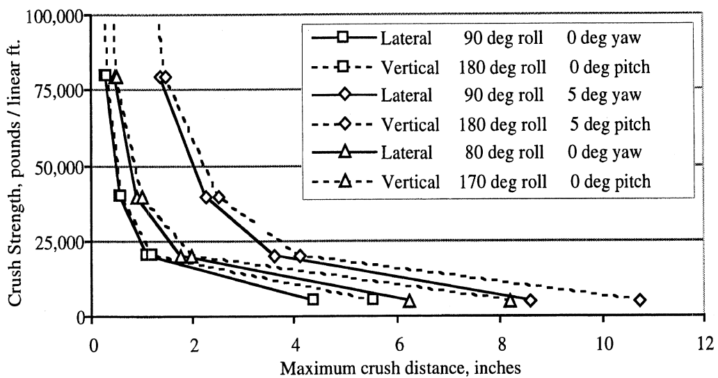
Figure 40. Comparison of results from similar vertical and lateral impacts of the Lantana semitrailer (all at 12 ft/sec)
