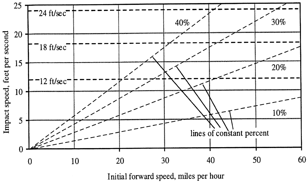
Figure 39. The relationship between percent of initial forward speed in miles per hour and impact speed in ft/sec
