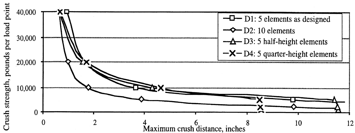
Figure 38. The influence of variations of discrete-element design on the rolling-impact results for the Albuquerque vehicle
