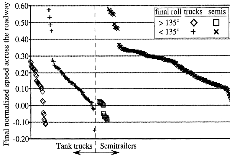
Figure 25. Final speed of the tank units across the roadway
