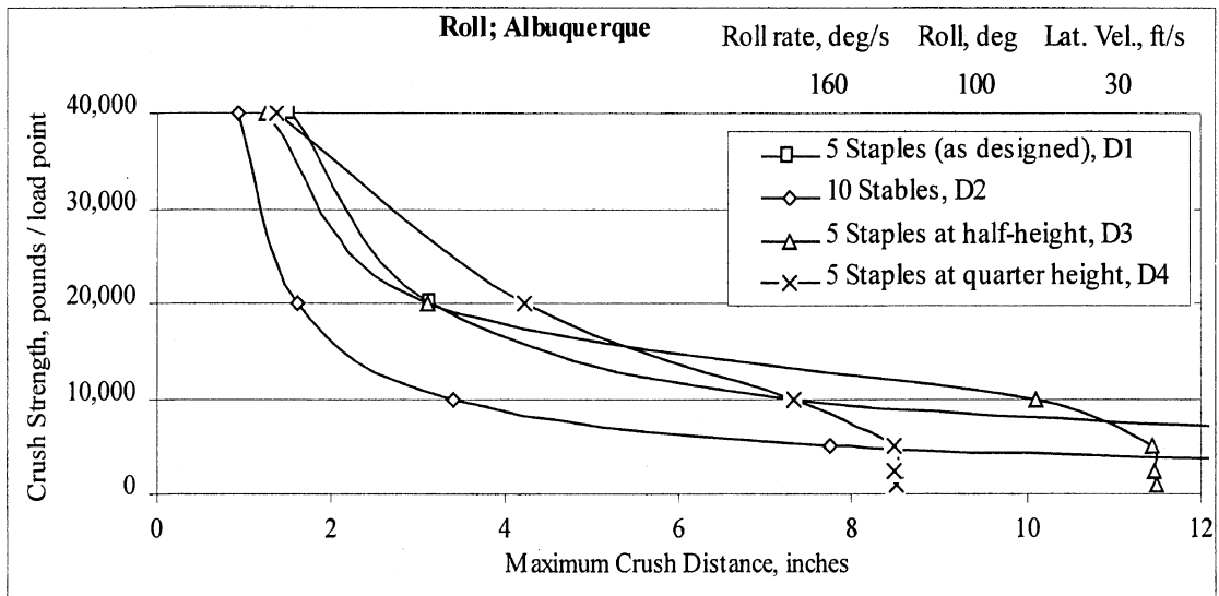
Figure C-2. Roll results for Albuquerque for the “fast” roll simulation
