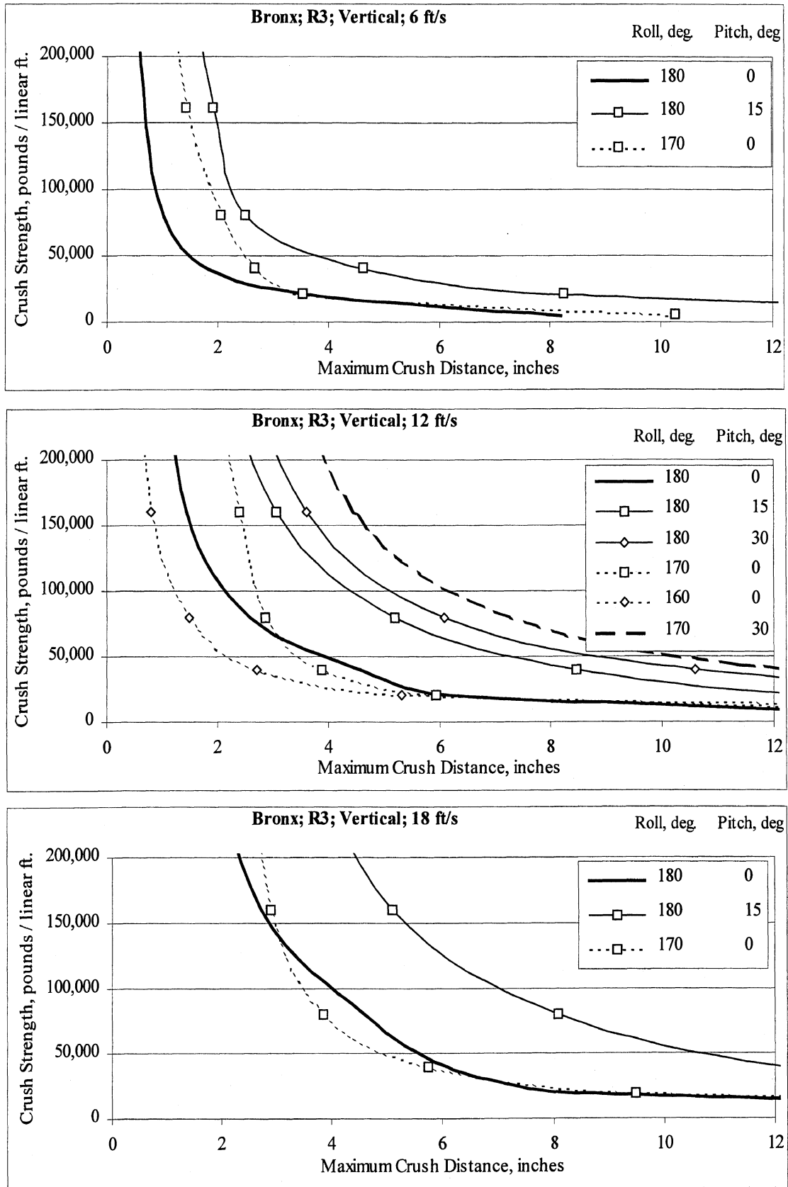
Figure C-10. Vertical results for Bronx with flat rails and crowned dams as designed.
