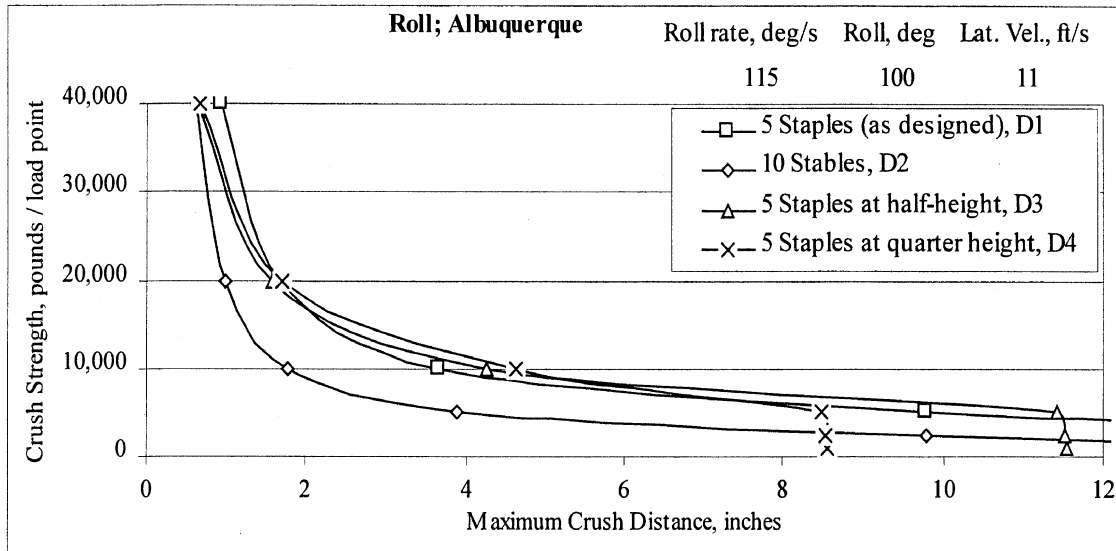
Figure C-1. Roll results for Albuquerque for the “slow” roll simulation
