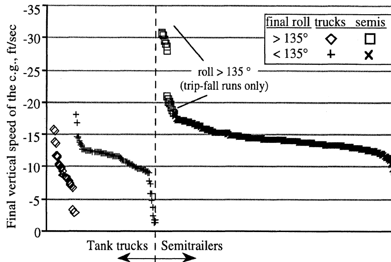
Figure 21. Final vertical speeds of the centers of gravity of the tank units
