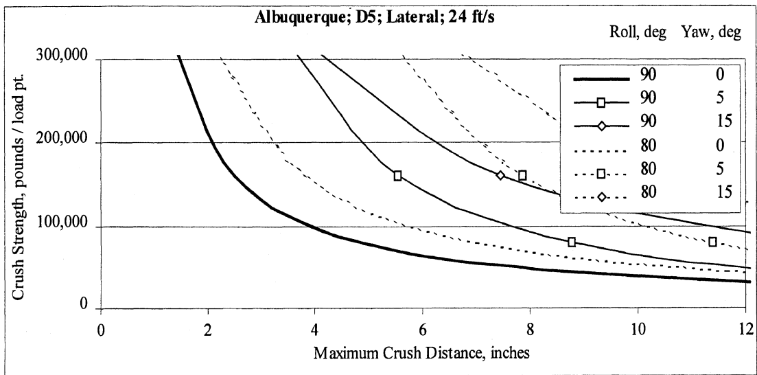
Figure C-21. Lateral results for Albuquerque with staples every 4 ft.
