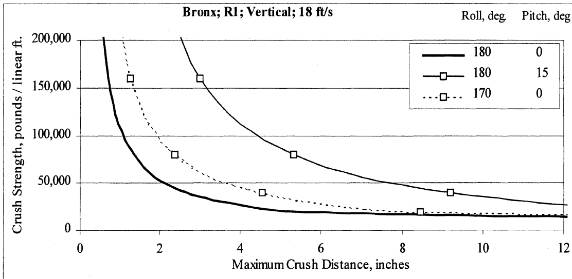
Figure C-8. Vertical results for Bronx with flat rails and flat end dams only.
