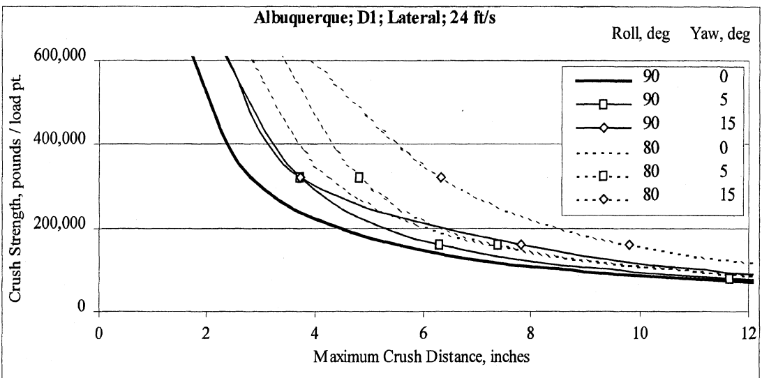
Figure C-20. Lateral results for Albuquerque as designed
