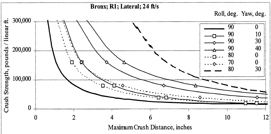
Figure C-23. Lateral results for Bronx with flat rails and flat end dams only.
