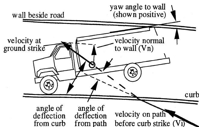
Figure 9. Plan-view of a vehicle rolled onto its side at the completion of a simulation run
