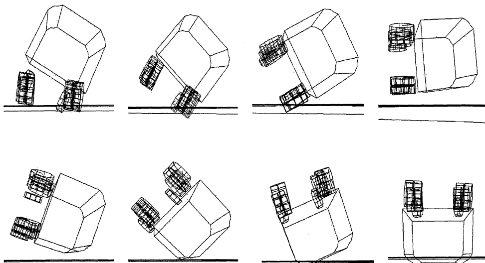
Figure 14. The Bronx vehicle rolling over after striking a curb (run #28, \Delta t=0.1 sec)
