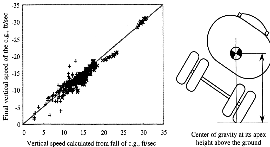
Figure 22. Comparison of final vertical speeds from the simulation and from the simple calculation based on the center of gravity falling from its apex height
