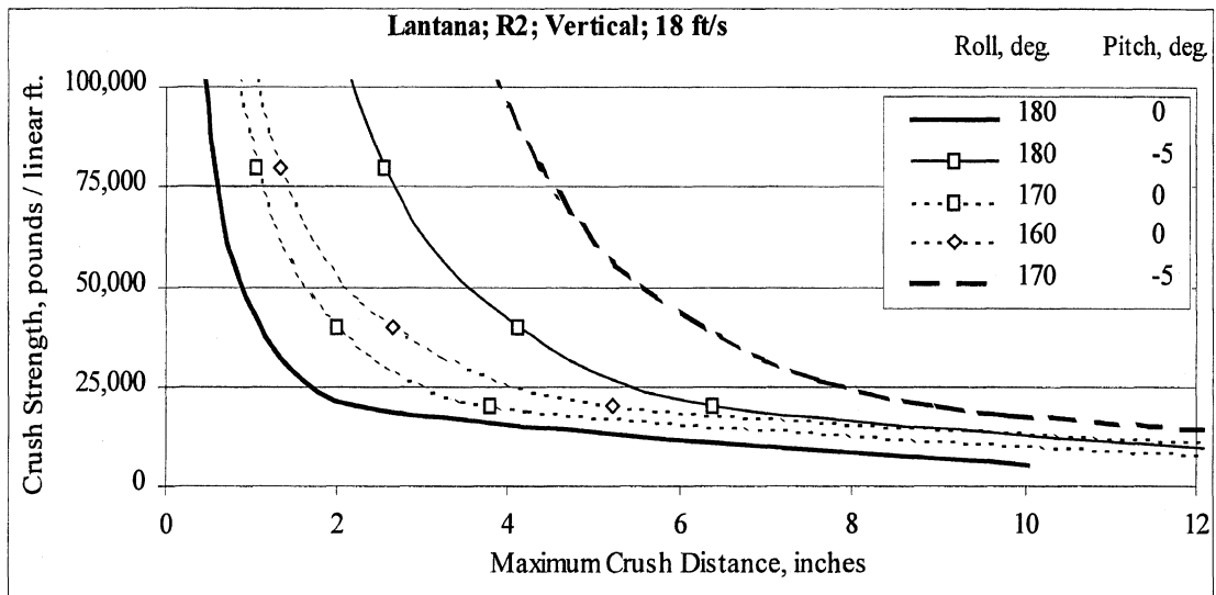
Figure C-18. Vertical results for Lantana with flat rails and flat dams every 6 ft.
