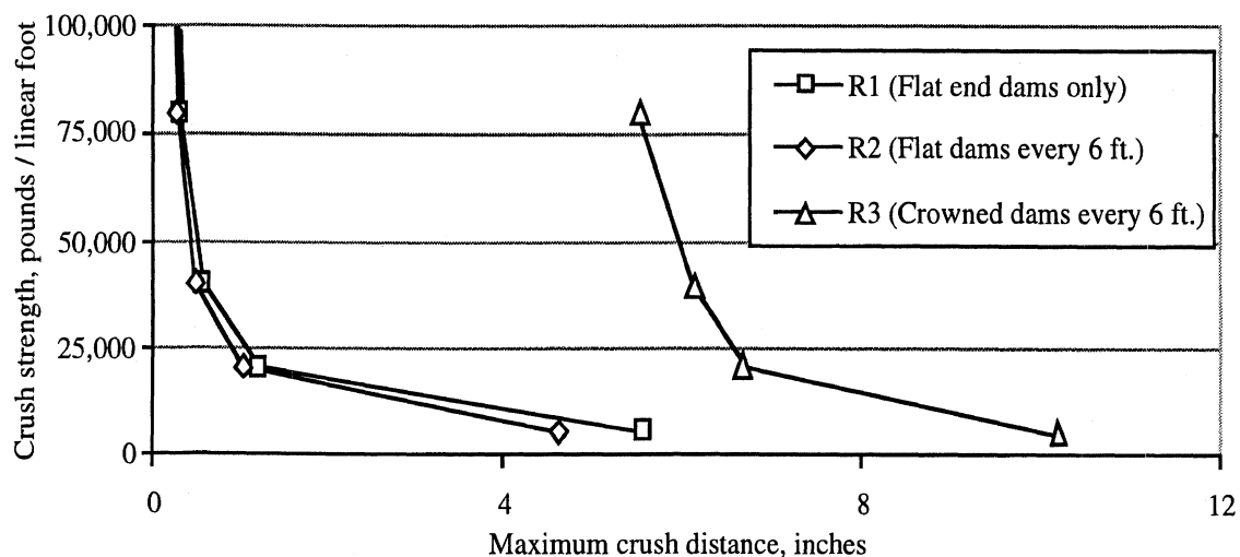
Figure 47. Comparison of results for various protector configurations
