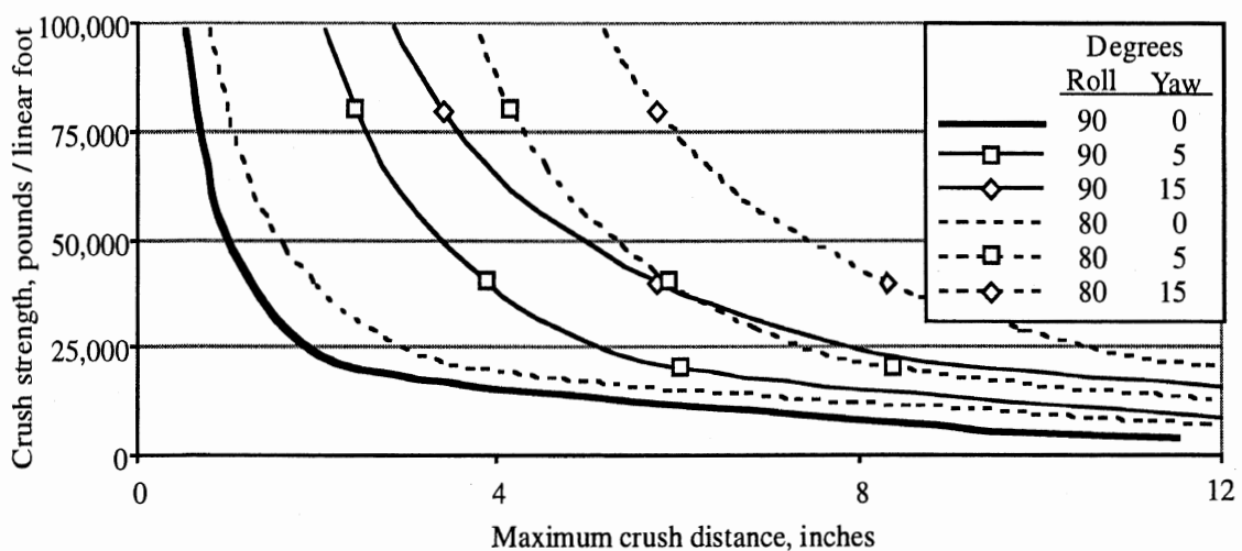
Figure 46. Results from lateral impacts of the Lantana semitrailer (R1) at 18 ft/sec and at various roll and yaw angles
