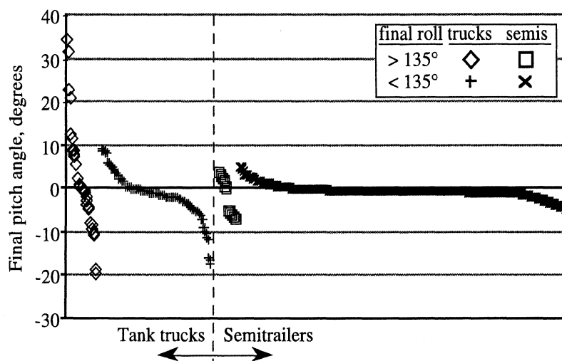
Figure 23. Final pitch angles of the tank units
