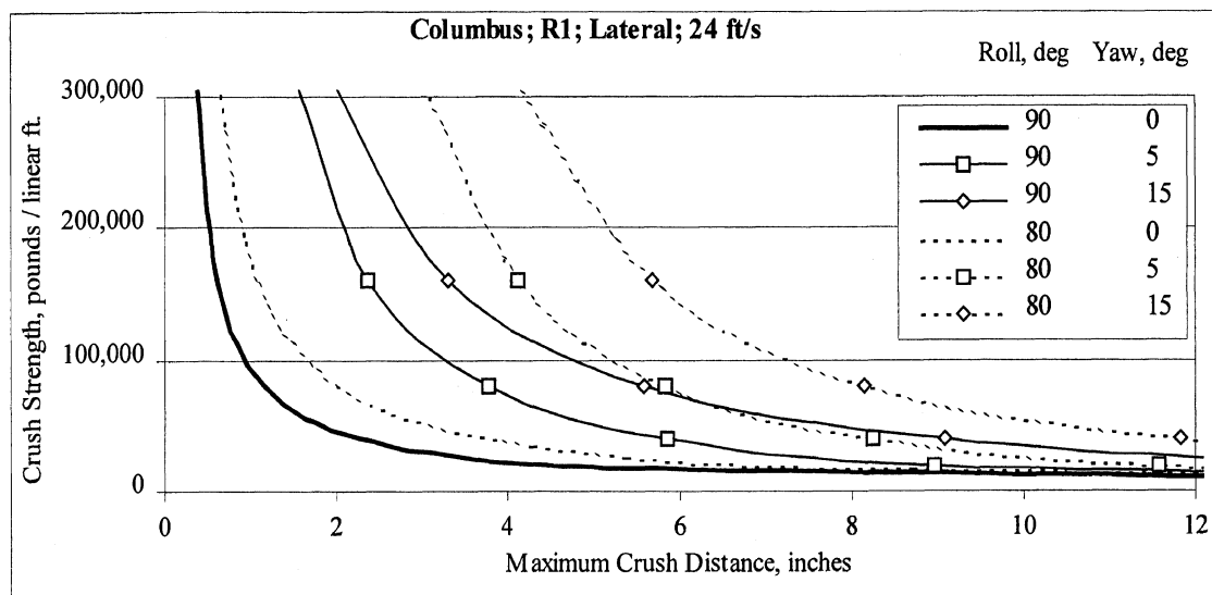
Figure C-29. Lateral results for Columbus with flat rails and flat end dams only.
