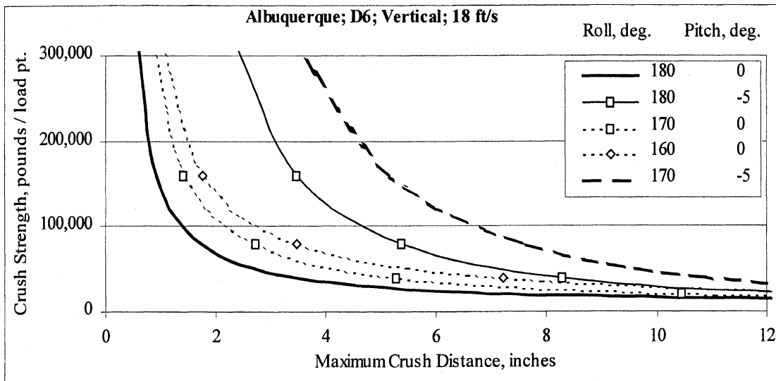
Figure C-7. Vertical results for Albuquerque with staples every 2 ft.
