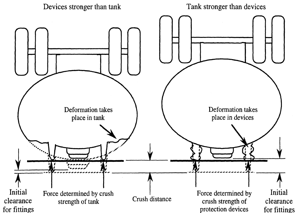
Figure 28. Impact deformation may take place in the tank or in the rollover-protection devices
