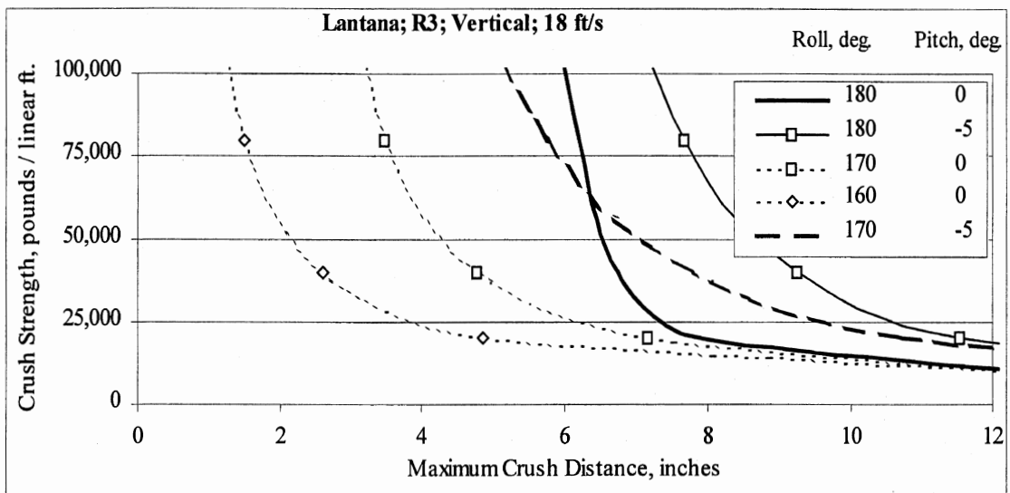
Figure C-19. Vertical results for Lantana with flat rails and crowned dams.
