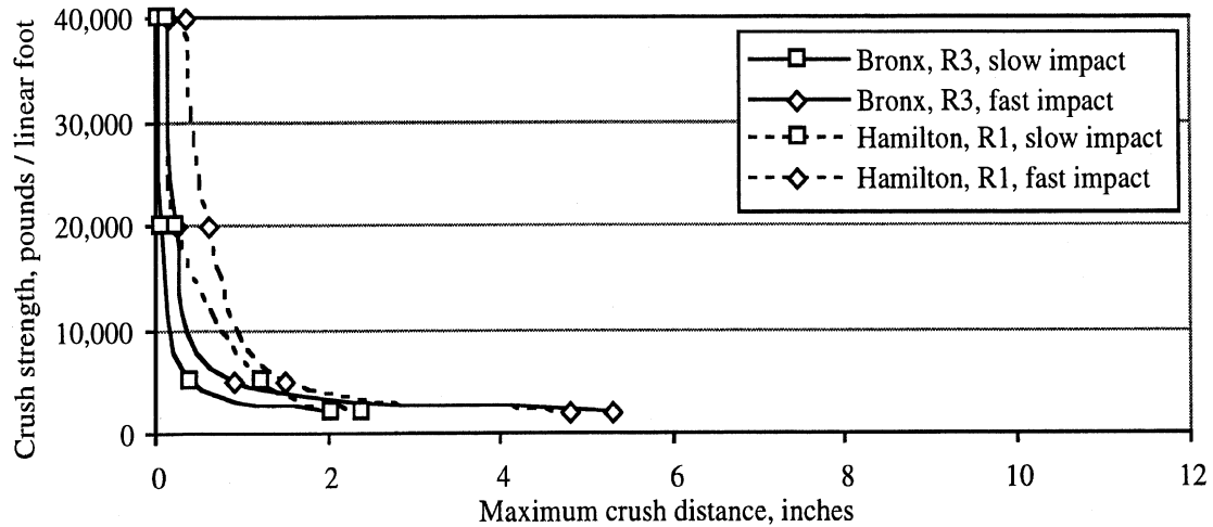
Figure 35. Rolling-impact results for the trucks in their as-designed configurations
