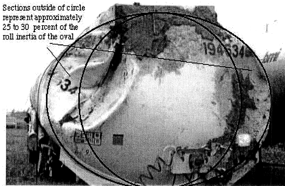
Figure 6. Estimating the roll moment of inertia of the liquid load
