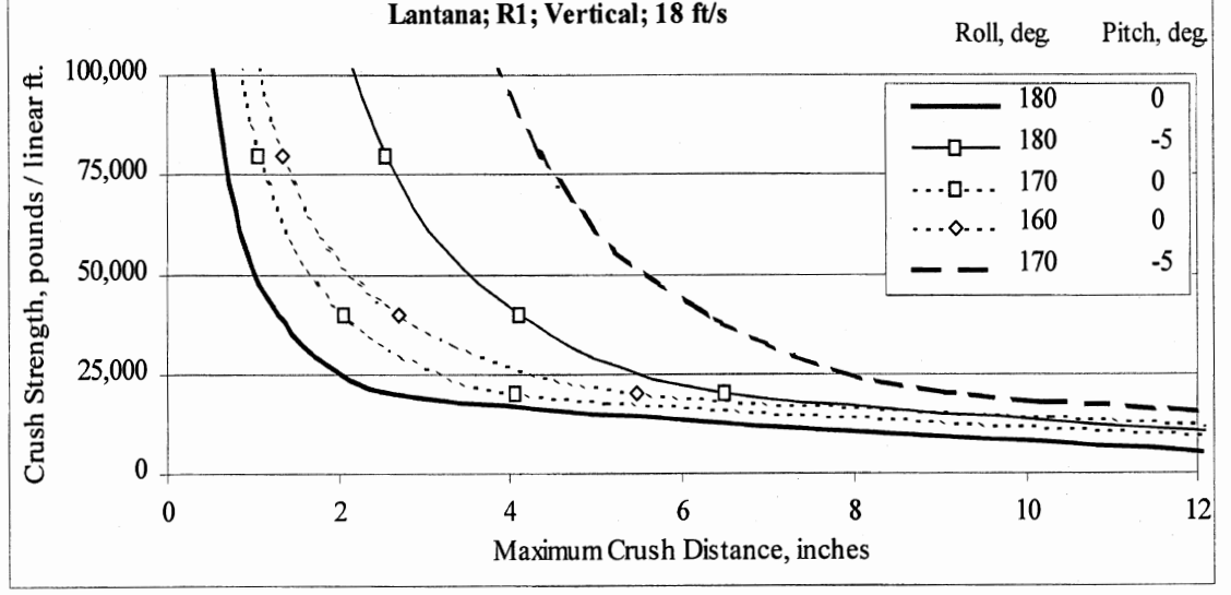
Figure C-17. Vertical results for Lantana with flat rails and flat end dams only.
