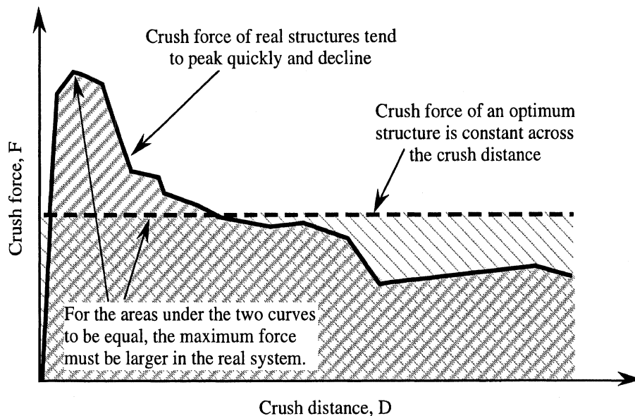
Figure 29. Comparison of the energy dissipation performance of idealized and realistic structures
