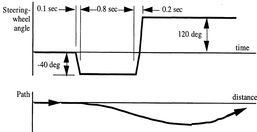
Figure 8. The open-loop high-speed avoidance maneuver
