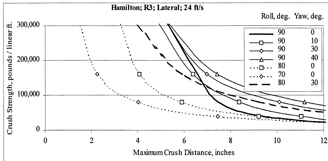
Figure C-28. Lateral results for Hamilton with flat rails and crowned dams every 6 ft.
