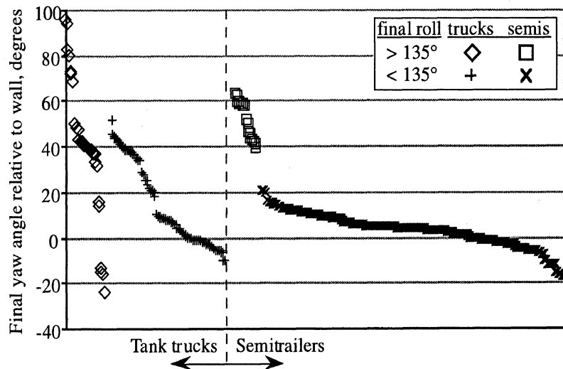
Figure 27. Final yaw angle of the tank units relative to a vertical surface parallel to the road
