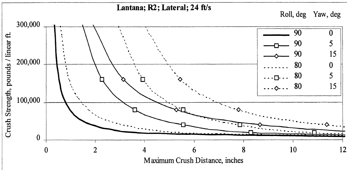
Figure C-33. Lateral results for Lantana with flat rails and flat dams every 6 ft.
