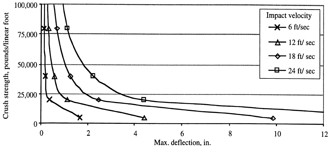
Figure 41. The influence of velocity on the results from simulations of the Lantana semitrailer in flat-on-the-top impacts
