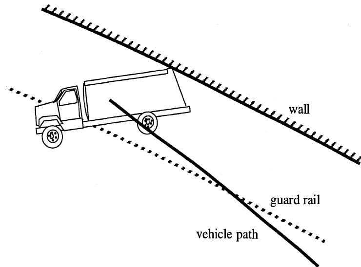
Figure 17. Plan-view sketch of the Hamilton vehicle at the end of run #52
