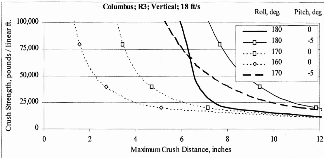
Figure C-16. Vertical results for Columbus with flat rails and crowned dams.
