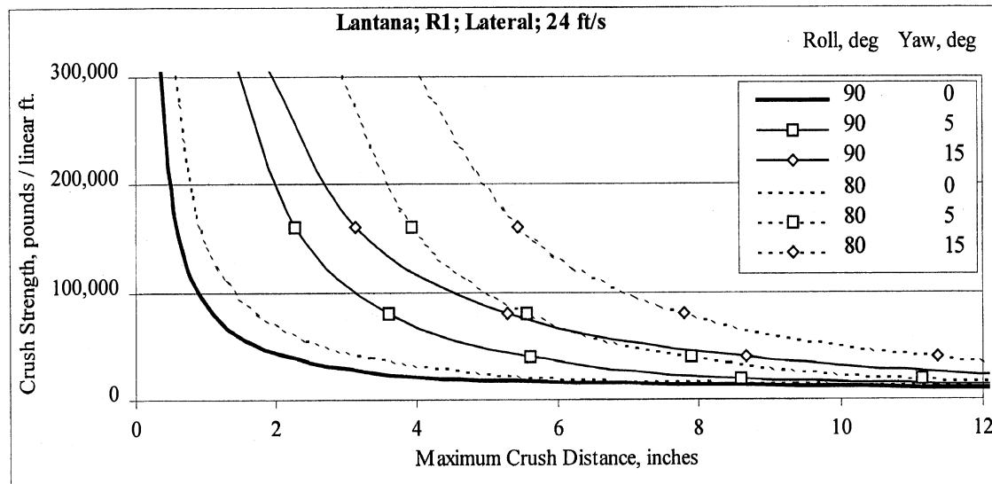
Figure C-32. Lateral results for Lantana with flat rails and flat end dams only.
