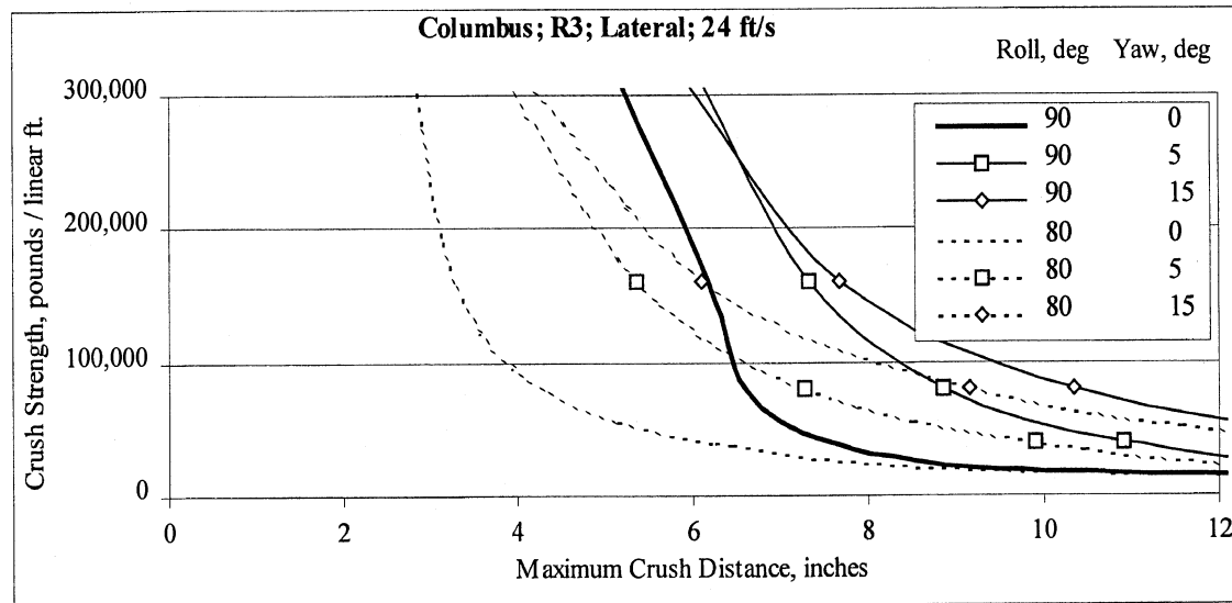
Figure C-31. Lateral results for Columbus with flat rails and crowned end dams every 6 ft.
