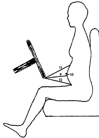
Figure A.4. Measurements from bottom of steering-wheel rim to abdomen.
