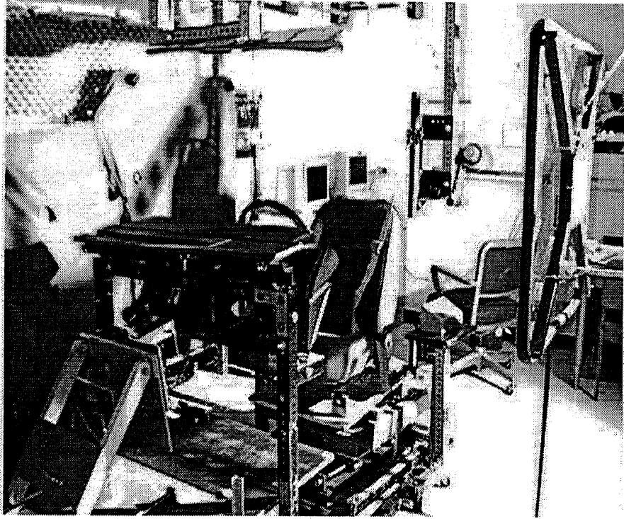
Figure 3. Adjustable laboratory seating buck.
