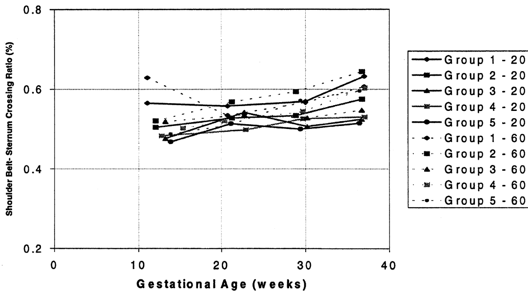
Figure 51. Ratio of shoulder-belt crossing on sternum by gestational age for 360-mm seat-height configurations. Dashed lines correspond to the 60° nominal shoulder-belt angle, while solid lines designate the 20° shoulder-belt angle.
