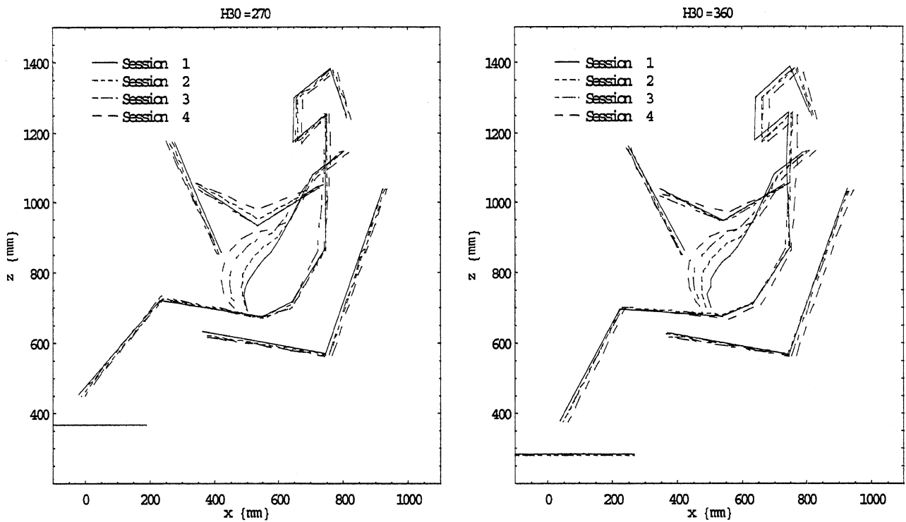
Figure G.2. Average postures and abdomen contours of Group-2 subjects for each gestational age and seat height.
