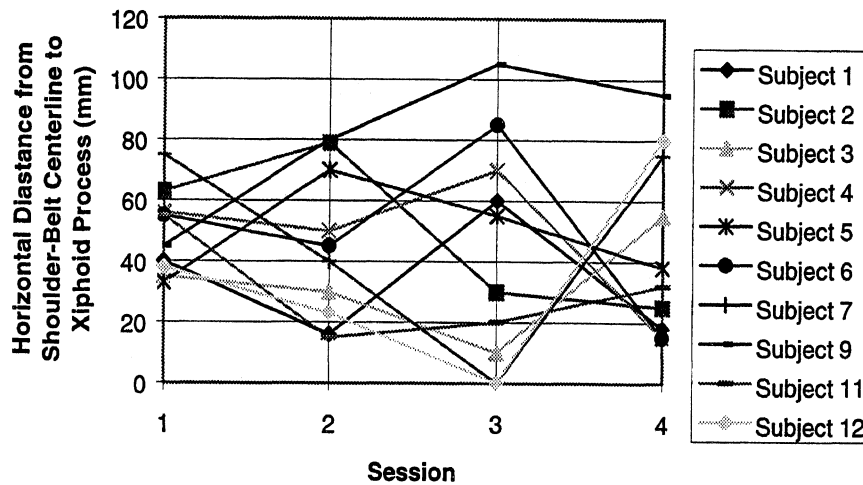
Figure A.25. Horizontal distance from the shoulder-belt centerline to the xiphoid process (measurement B in Figure A.23).
