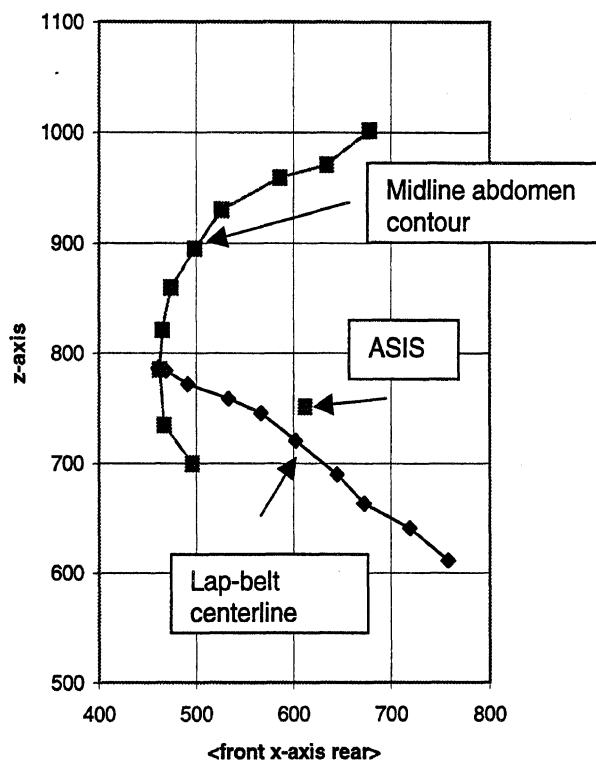
Figure 73. Relationship between lap-belt routing, ASIS, and abdomen contour in later months of pregnancy.
