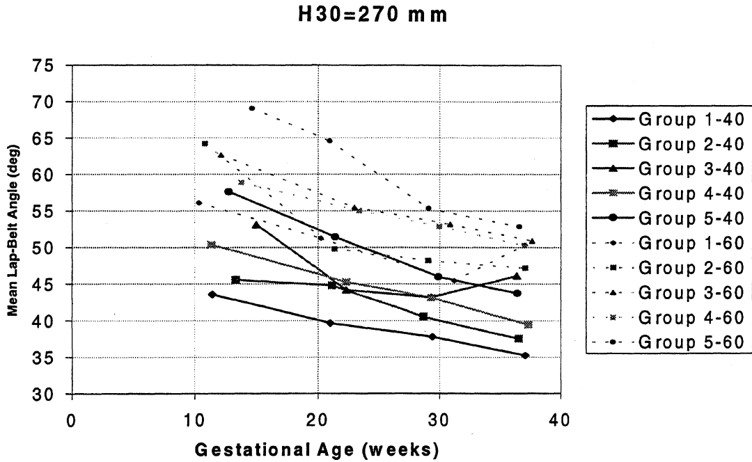
Figure 41. Mean actual lap-belt angles by gestational age for each stature group and nominal belt-angle condition for the 270-mm seat-height configurations. Dashed lines correspond to the 60^\circ nominal lap-belt angle, while solid lines designate the 40^\circ lap-belt angle.
