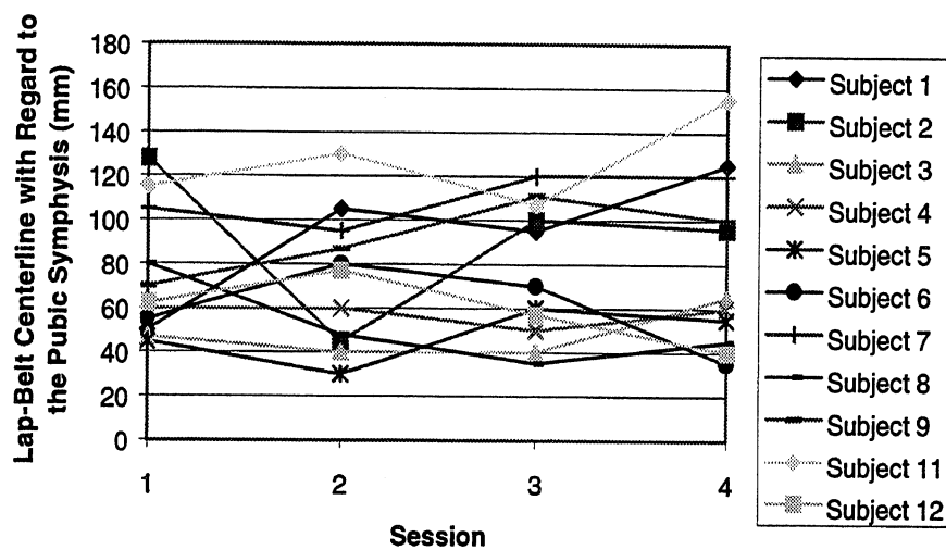
Figure A.22. Vertical location of the lap-belt centerline relative to the pubic symphysis.
