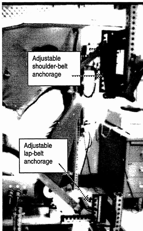
Figure 5. Side-view of test buck showing fixtures for adjusting seat-belt anchor points.
