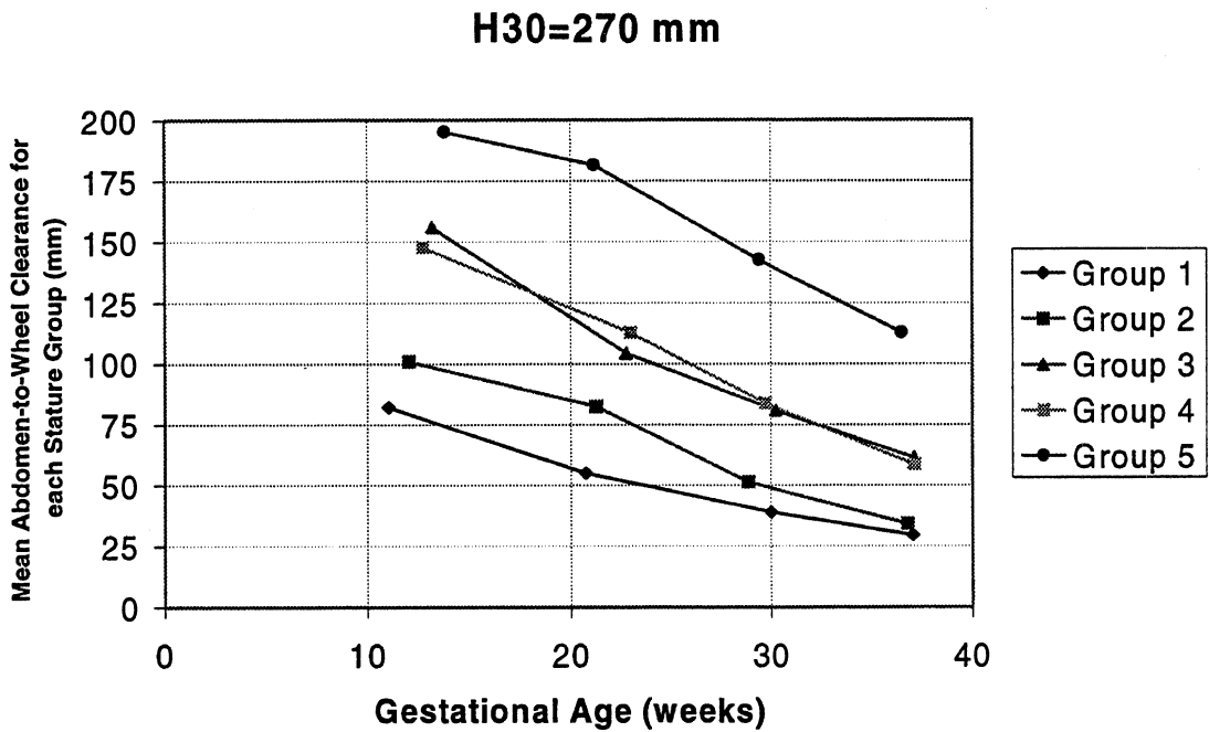
Figure 27. Mean abdomen-to-wheel clearance by gestational age for each stature group for 270-mm seat-height configurations.
