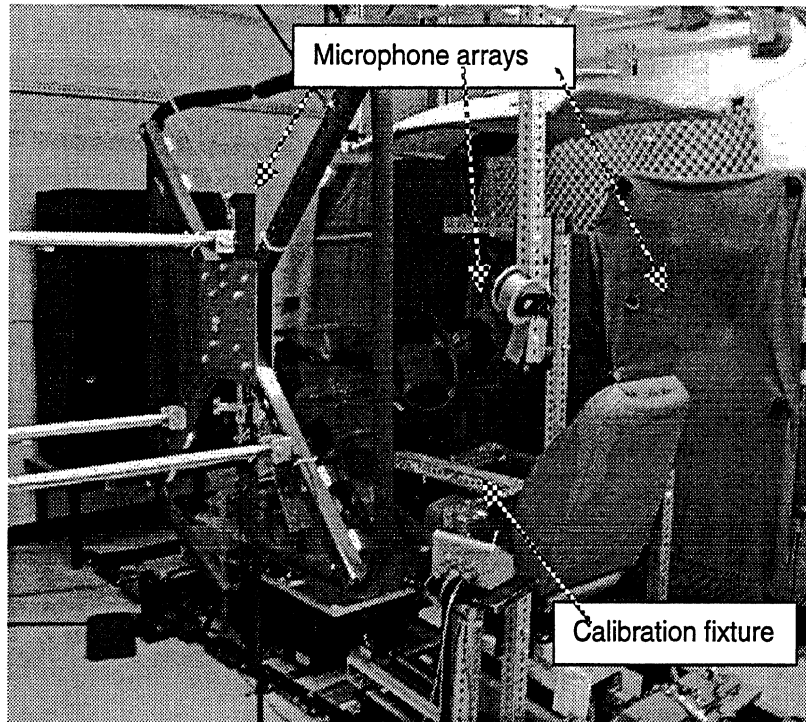
Figure 8. Seating buck with three microphone arrays and calibration fixture in place.
