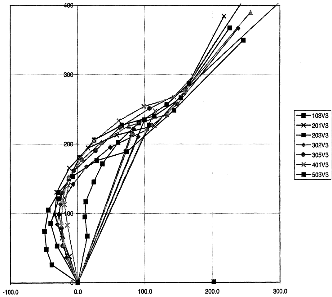
Figure 36. Abdomen contours for third test session of subjects with abdomen depths close to the mean for all subjects.
