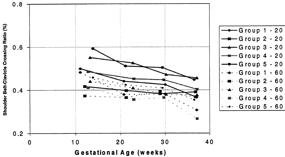
Figure 53. Ratio of shoulder-belt crossing on clavicle by gestational age for 270-mm seat-height configurations. Dashed lines correspond to the 60° nominal shoulder-belt angle, while solid lines designate the 20° shoulder-belt angle.
