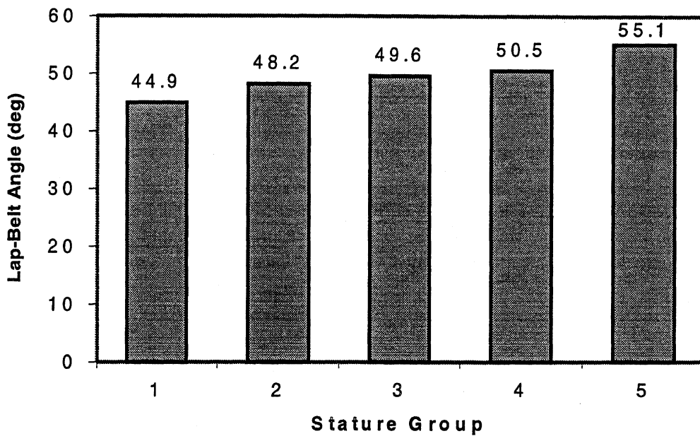
Figure 44. Mean lap-belt angles by stature group.
