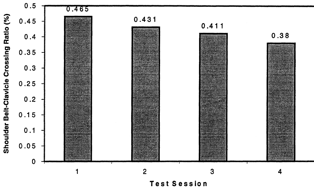
Figure 55. Ratio of shoulder-belt crossing on clavicle by test session for all stature groups and test configurations.
