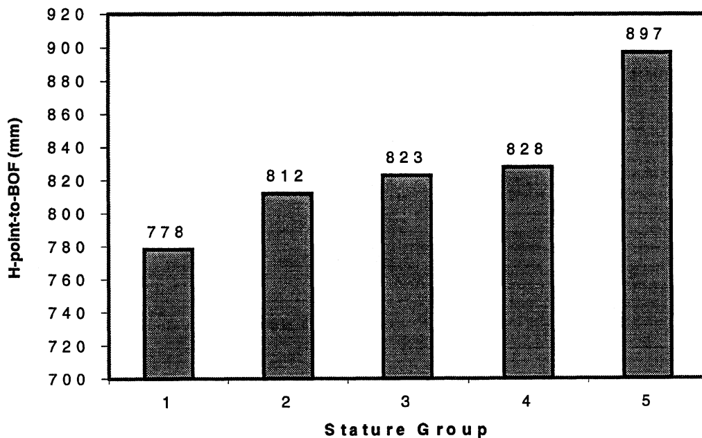
Figure 25. H-point-to-BOF distance by stature group for all test sessions and configurations.
