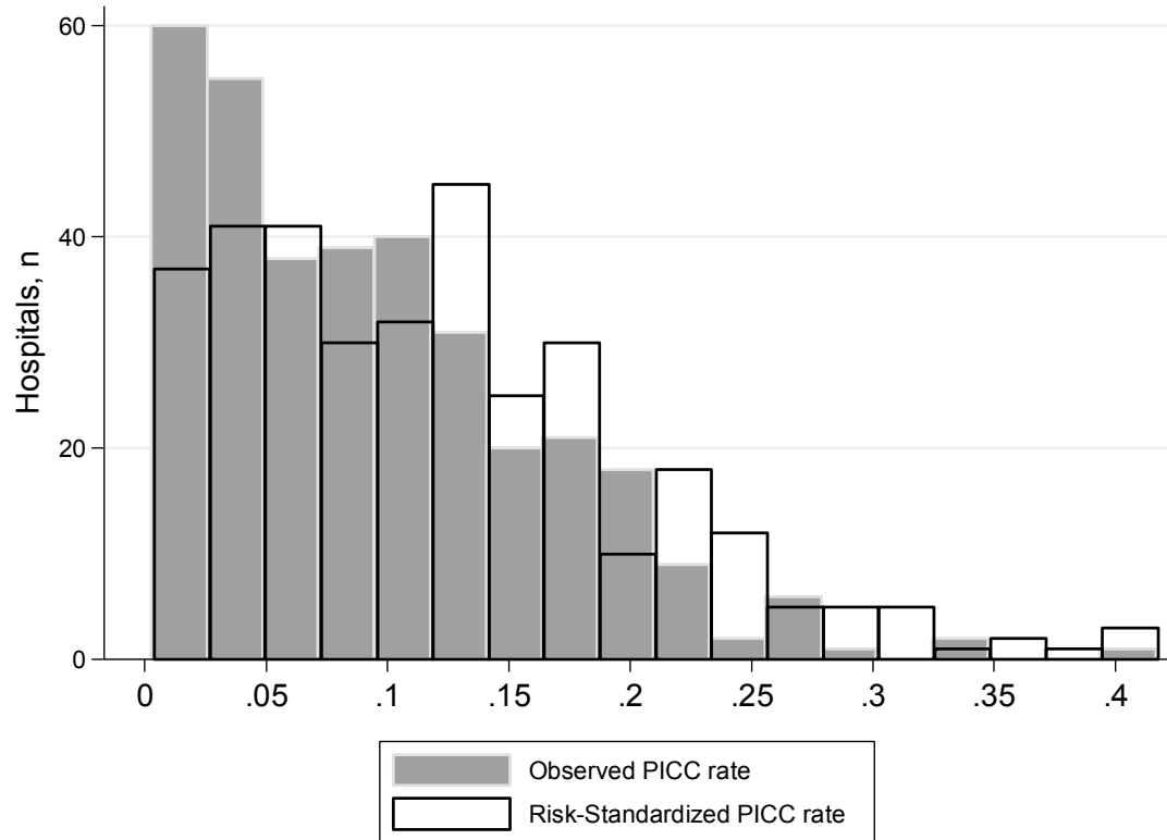
FIGURE 2: OBSERVED VS. RISK-STANDARDIZED RATE OF PICC USE ACROSS 343 US HOSPITALS (RESTRICTED TO SITES WHERE > 5 PATIENTS RECEIVED PICCS)
