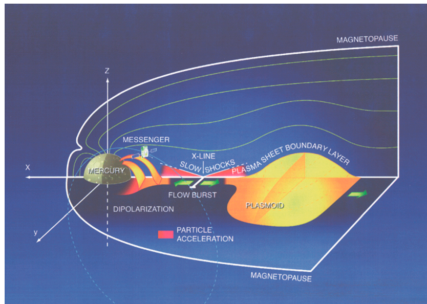
Figure 10. Schematic diagram of Mercury's magnetosphere showing substorm phenomenology as observed by MESSENGER, including energetic particle acceleration and near-midnight magnetic field reconfigurations [Slavin et al. , 2007].
