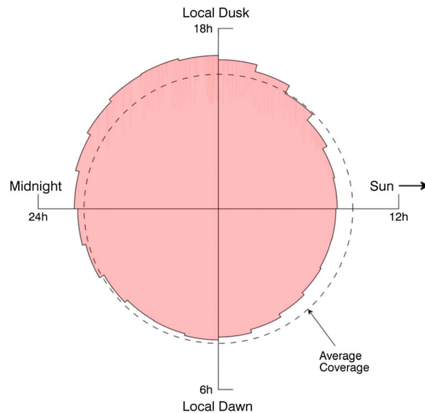
Figure 1. MESSENGER coverage in local time (LT) over the period of study, grouped into 1-h bins. The radius of each bin denotes its relative coverage, and the dashed circle marks the average coverage. For this study, “average” coverage constituted 608.4 h of data accumulation. The minimum coverage (10–11 LT) was 531.2 h, and the maximum coverage (19–20 LT) was 703.7 h. Hence, MESSENGER observations were relatively uniform in local time, with a slight bias toward postdusk/premidnight.
