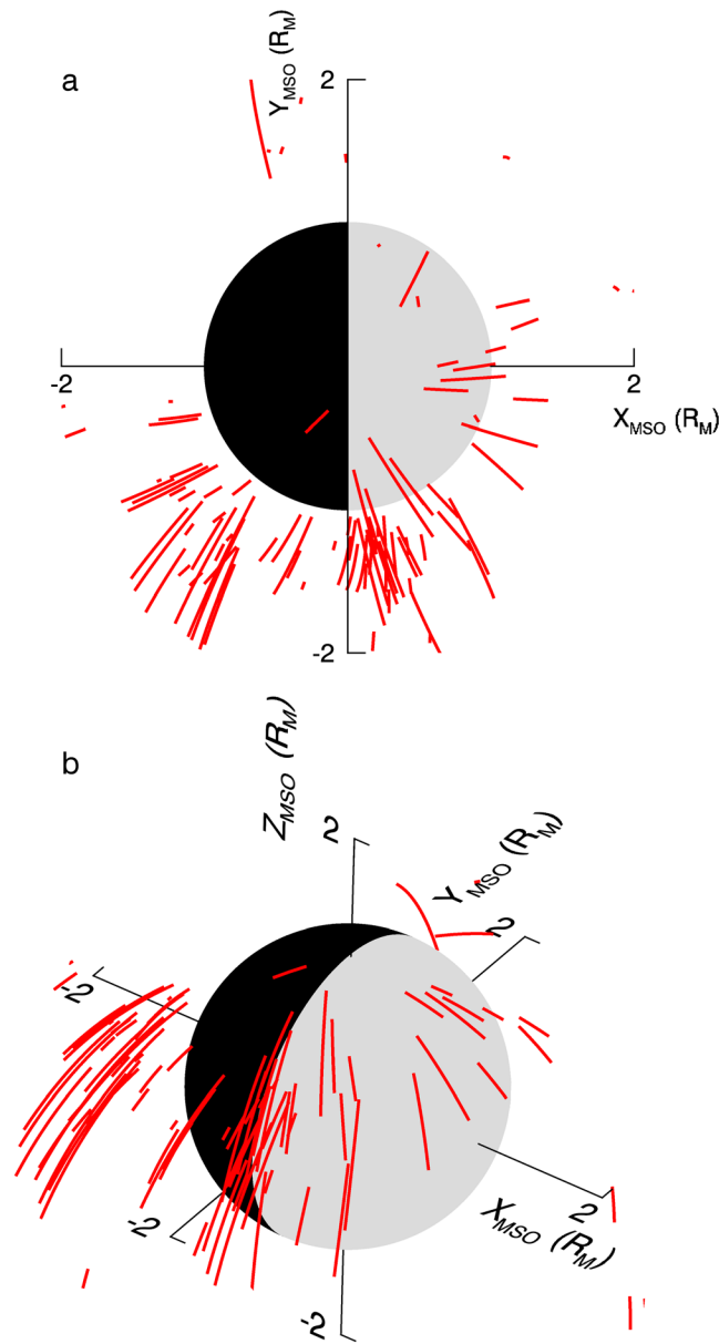
Figure 9. Diagrams showing spatial locations and extents of all energetic electron events in this study. (a) Projection of MESSENGER orbits onto the MSO X-Y plane during times when events were detected. (b) Representation of orbit trajectory segments during electron bursts shown in a three-dimensional projection.
