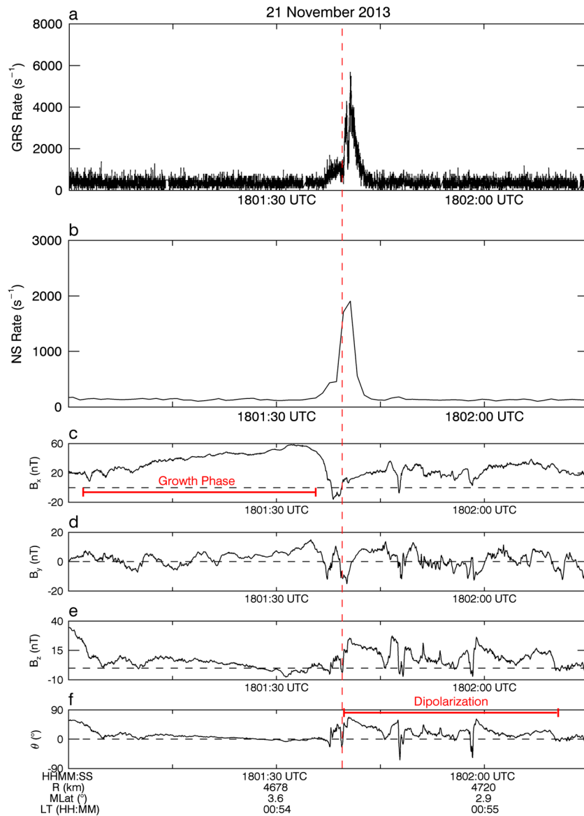
Figure 6. An electron injection event in (a) GRS and (b) NS data near Mercury local midnight on 21 November 2013. The format follows that in Figure 2. (c–f) Magnetic field inclination angle data show substorm-like field changes, as described in the text.
