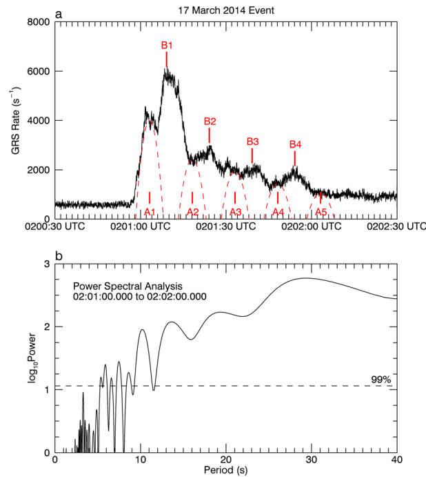
Figure 5. (a) GRS data for 17 March 2014 for the same period as that shown in Figure 3a but with a 10-sample smoothing filter applied. This plot shows the 15-s period “drift echoes” in the data set indicated by the tick marks labeled A1, A2, ... and B1, B2, ..., as described in the text. The red dashed curves indicate the A population. (b) Power spectral analysis for the time series in Figure 5a.
