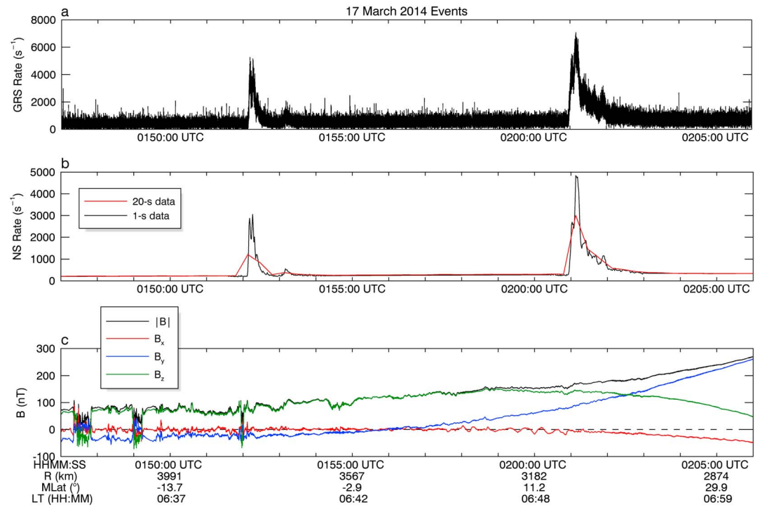
Figure 2. (a) High-time-resolution (10-ms sampling) records from the Gamma-Ray Spectrometer (GRS) anticoincidence shield detector on the MESSENGER spacecraft. Data are shown for the period from 0147 to 0206 UTC on 17 March 2014. (b) Data for the same time interval as in Figure 2a from the MESSENGER Neutron Spectrometer. The black trace shows data at 1-s cadence from NS, and the red curve shows data sampled every 20 s. (c) Magnetic field data from 17 March 2014. Magnetic field components are in the MSO coordinate system.
