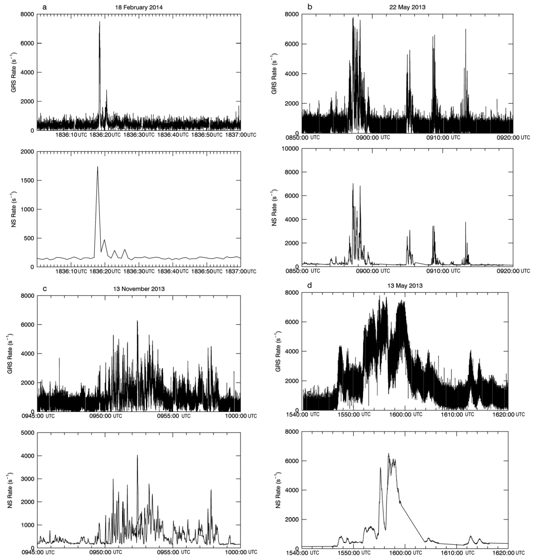
Figure 7. Different types of energetic electron enhancement events analyzed in this study. (a) Another near-midnight injection event. (b) Multievent enhancement. (c) Periodic electron event. (d) Smooth type of energetic electron event.
