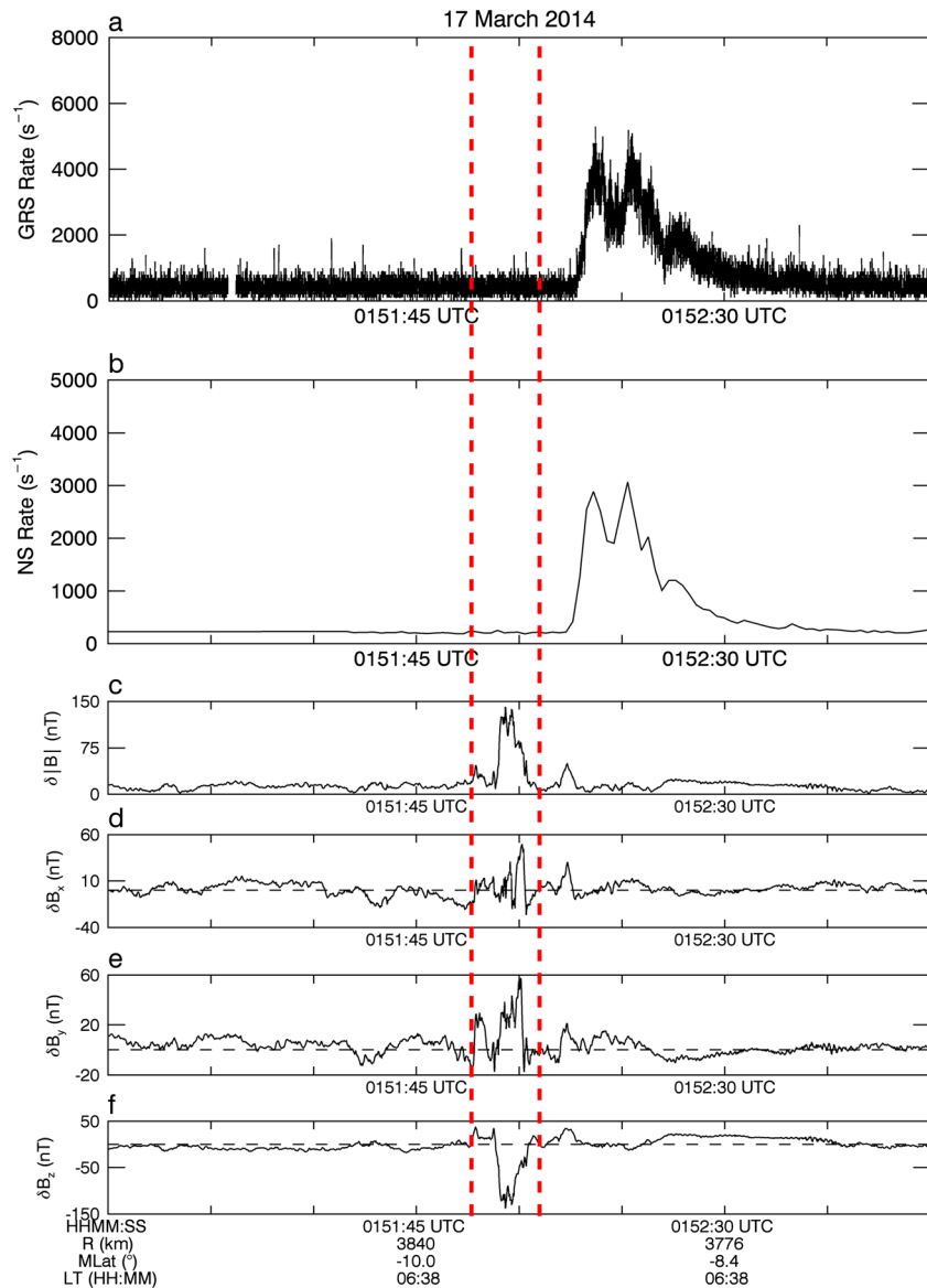
Figure 3. Detailed (a) GRS and (b) NS data for the period from 0151 to 0153 UTC on 17 March 2014. (c-f) Residual magnetic field data from MESSENGER for the same period: \delta B , \delta B_x , \delta B_y , and \delta B_z , respectively. The vertical dashed lines delineate magnetopause crossings by the spacecraft.
