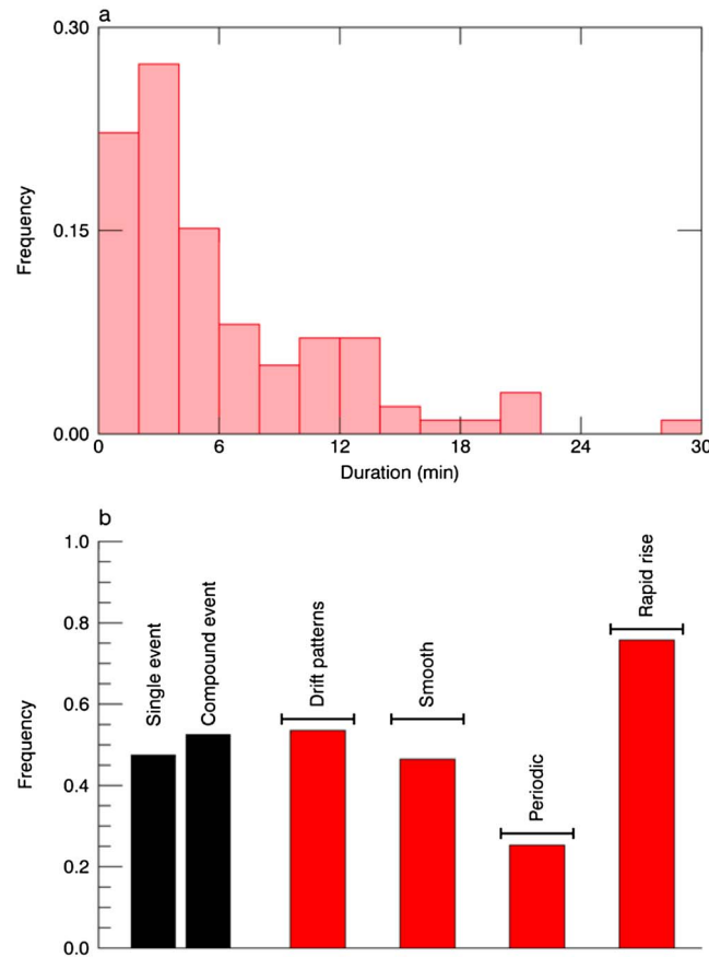
Figure 8. (a) Frequency of occurrence versus duration of events for energetic electron enhancements analyzed in this study. (b) Percentage of different types of electron enhancement events in this study.
