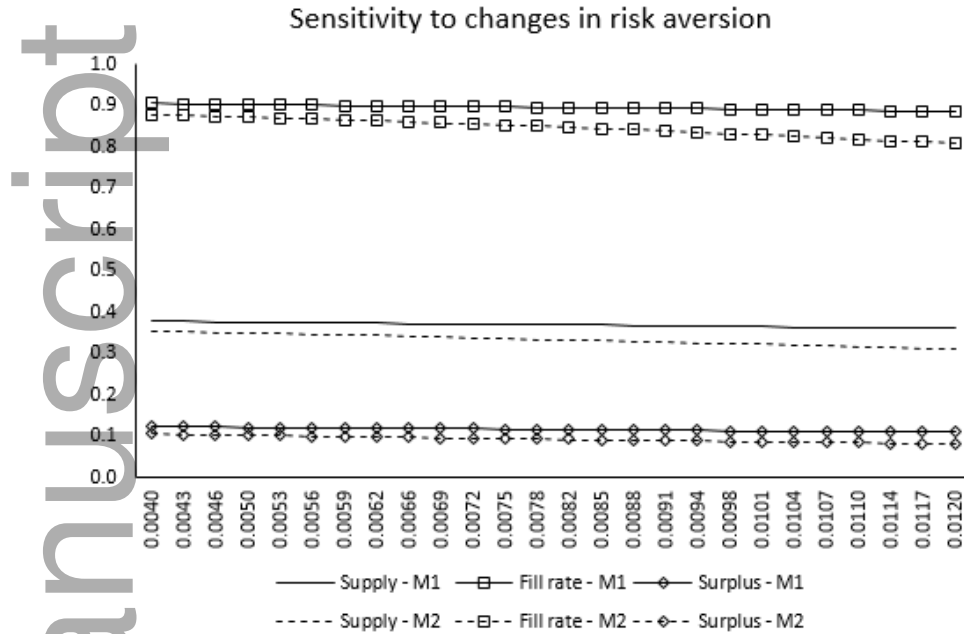
Figure A3: Sensitivity of total supply, fill rate, and supplier surplus to changes in supplier risk aversion ( \gamma ).
