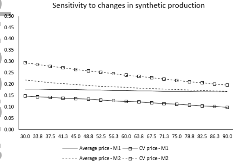
Figure 10: Sensitivity of average price (divided by $2,000) and price coefficient of variation to changes in semi-synthetic production ( s ).
