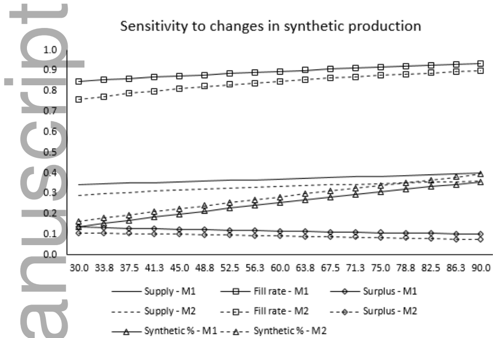
Figure 5: Sensitivity of total supply, fill rate, and supplier surplus to changes in semi-synthetic production ( s ). The figure also includes semi-synthetic production as a fraction of the total ( s/(s + q^*) ).
