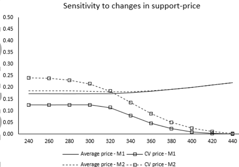
Figure 11: Sensitivity of average price (divided by $2,000) and price coefficient of variation to changes in the support-price ( p_0 ).
