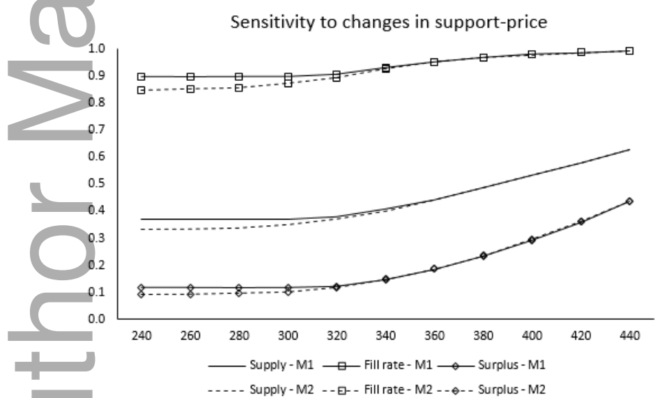
Figure A8: Sensitivity of total supply, fill rate, and supplier surplus to changes in the support-price ( p_0 ). The average total spend ranges for $73m (base-case value) to $105m for M1 and $75m to $175m for M2 as the support-price ranges from $240 to $440.
