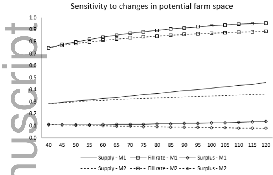
Figure A5: Sensitivity of total supply, fill rate, and supplier surplus to changes in potential farm space (c).
