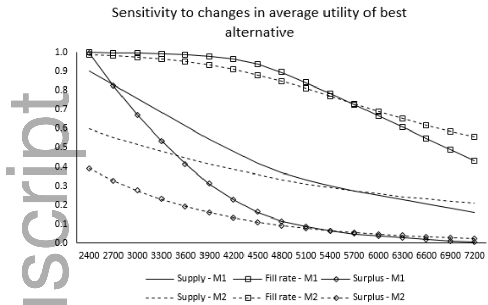
Figure A7: Sensitivity of total supply, fill rate, and supplier surplus to changes in average utility of the best alternative ( \mu_b ).
