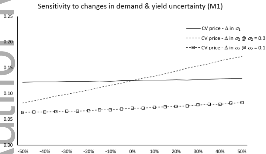
Figure 9: Sensitivity of price coefficient of variation to changes in demand uncertainty ( \sigma_1 ) and yield uncertainty ( \sigma_2 ). The sensitivity to yield uncertainty is illustrated at the base-case value \sigma_2 = 0.3 , and at \sigma_2 = 0.1 = \sigma_1 . Sensitivity results are not reported for demand model M2 because demand uncertainty does not affect the system.
