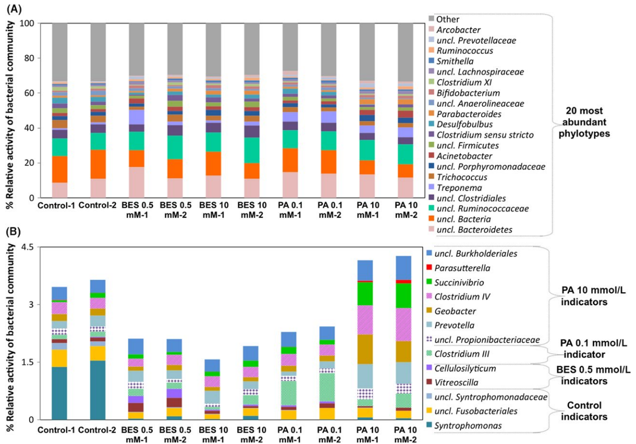
Figure 5. Relative activity based on the 20 most abundant bacterial phylotypes grouped at the genus level (A) and the phylotypes identified as indicator organisms ( P < 0.05 ) (B) in anaerobic mesocosms after 9 days of incubation for each inhibition condition. Duplicates shown represent duplicate biomass samples from the same reactors. No inhibitor was added in control conditions.
