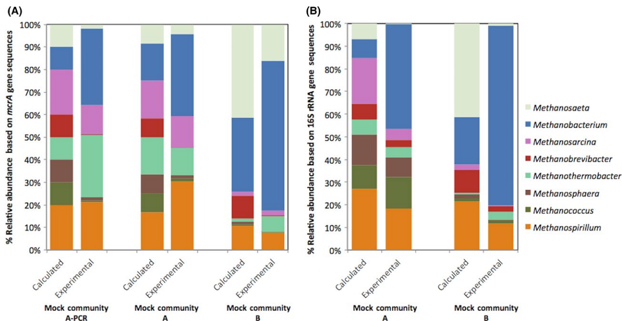
Figure 1. Comparison between the calculated and experimental relative abundance of methanogen mock communities based on the sequencing of the mcrA gene (A) and 16S rRNA gene (B). Mock community A-PCR was created by pooling the PCR products from individually amplified mcrA genes for each methanogen. Mock community A and B were created by pooling DNA extracts before amplification. The expected compositions were calculated based on DNA concentrations of the extracts from 10 strains measured by fluorospectrometry, genome size, and gene copy number, or PCR product quantification by fluorospectrometry (Table S2). Two different strains were included for the genera Methanospirillum and Methanosarcina . All strains included in the mock communities were identified through mcrA gene and 16S rRNA gene sequencing. The mcrA gene-based sequencing results included one sequence each identified as Methanohalophilus and Methanoculleus , which were excluded from the graphs.
