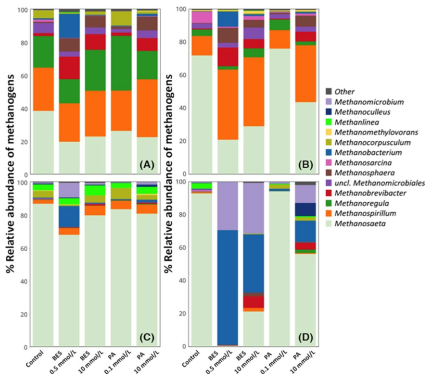
Figure 3. Relative abundance (DNA) and activity (RNA) of methanogens in anaerobic mesocosms after 9 days of incubation based on 16S rRNA genes (A), 16S rRNA cDNA (B), mcrA genes (C), and mcrA transcript cDNA (D), sequencing. Sequences from duplicate samples for each condition are combined (duplicates are shown in Figure S4).
