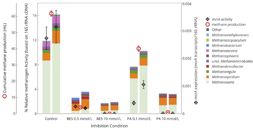
Figure 2. Cumulative methane production and molecular characterization of methanogens in cow dung and anaerobic digester sludge mesocosms after 9 days of incubation. Relative methanogen activity based on methanogen 16S rRNA cDNA as a % of the total community (including Bacteria and Archaea ) (bars), mcrA expression normalized by 16S rRNA cDNA (diamonds) determined with RT-qPCR, and cumulative methane production (circles). Error bars for methane production volume represent the propagated uncertainty in methane concentration measurements. mcrA expression is displayed as the averages and standard deviations of triplicate RT-qPCR reactions. Duplicates shown represent duplicate biomass samples from the same reactors. No inhibitor was added in control conditions.
