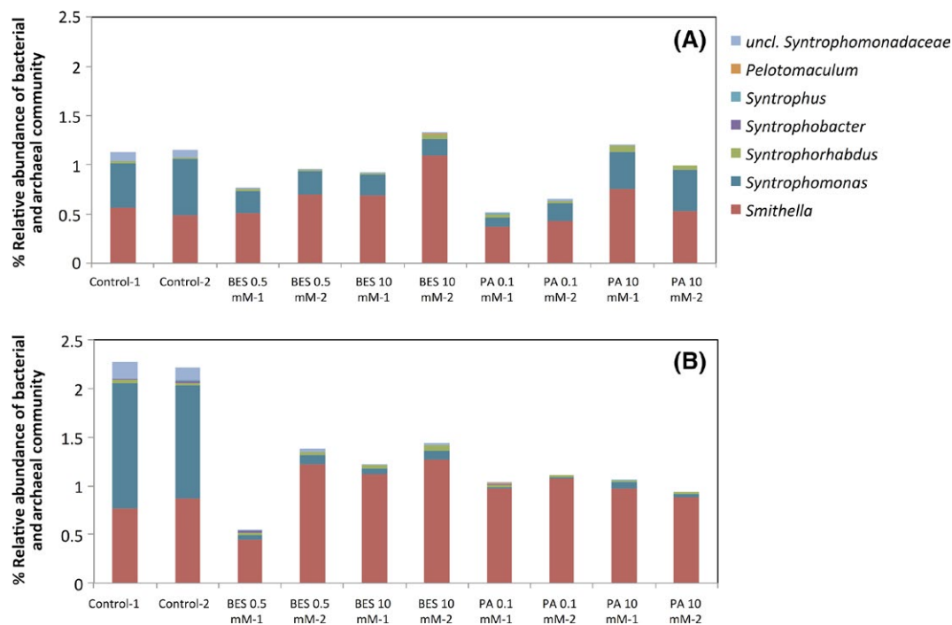
Figure 4. Relative abundance (A) and activity (B) of syntrophic bacteria as a percentage of the total bacterial and archaeal communities based on 16S rRNA gene and 16S rRNA cDNA sequencing in anaerobic mesocosms after 9 days of incubation. Duplicates shown represent duplicate biomass samples from the same reactors.
