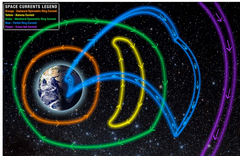
(b) Schematic of near-Earth nightside current systems
