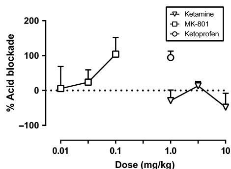
Figure 5 Effects of ketamine, MK-801 and ketoprofen on acid-depressed ICSS expressed as % acid blockade. Abscissa: Drug dose (mg/kg). Ordinate: Per cent blockade of acid-induced depression of ICSS. All data show mean \pm SEM for five, and ED50 values are reported in Table 1.
