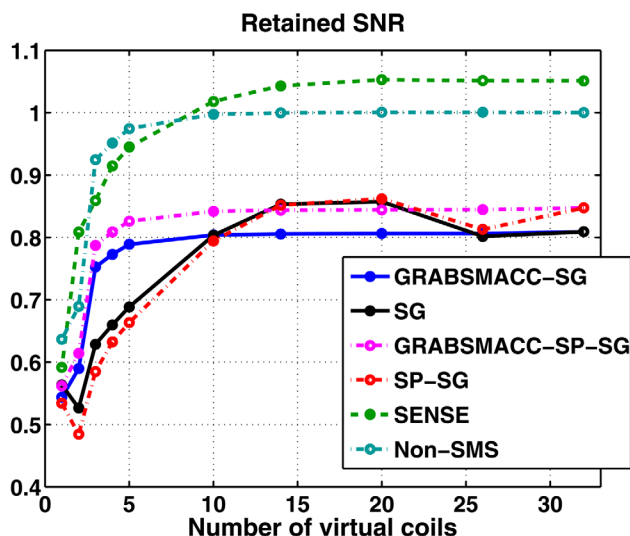
FIG. 7. Average retained SNR, or equivalently, average 1/g -factor within brain voxels.
