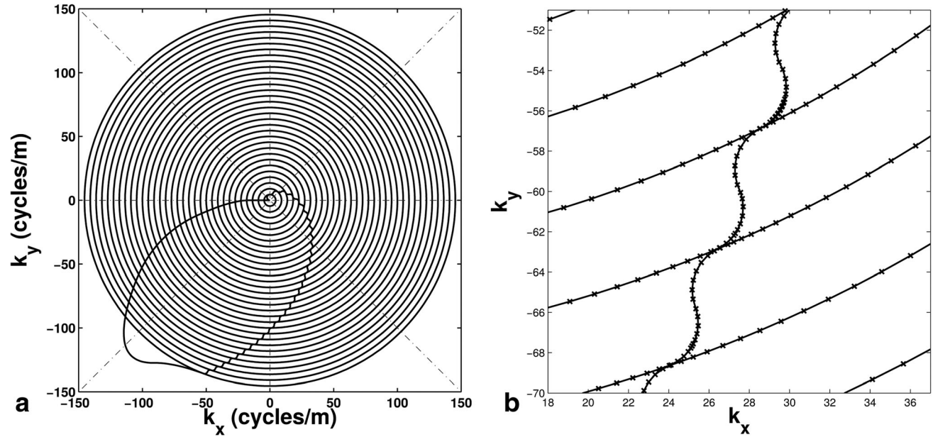
FIG. 1. a: k_x - k_y components of the concentric ring k-space trajectory used in this work. Boundaries of angular sectors for GRAPPA are shown with dash-dotted blue lines. b: Close-up of ring transitions with “x” markers indicating where samples were acquired.
