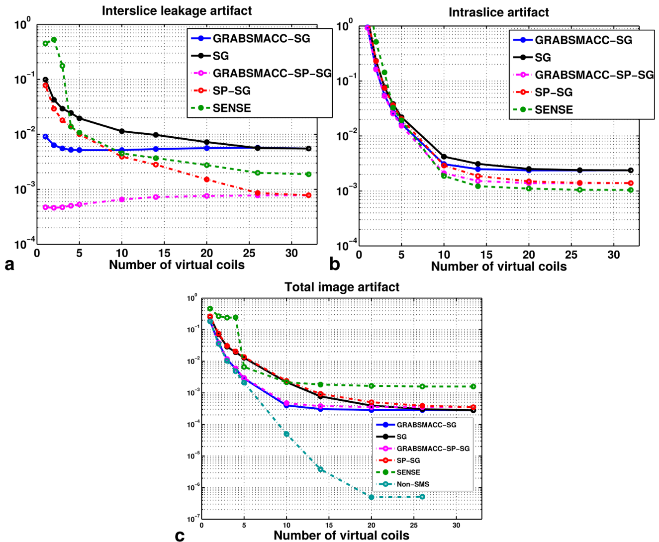
FIG. 5. a : Interslice leakage artifact metric ( L_{2-1} + L_{2-3} ), b : intraslice artifact metric ( l_{2-2} - l_2 ), and c : total image artifact metric ( L_{1-2} + l_{2-2} + L_{3-2} - l_2 ) for the middle slices of a three-simultaneous-slice-acquired volume of 39 total axial slices.
