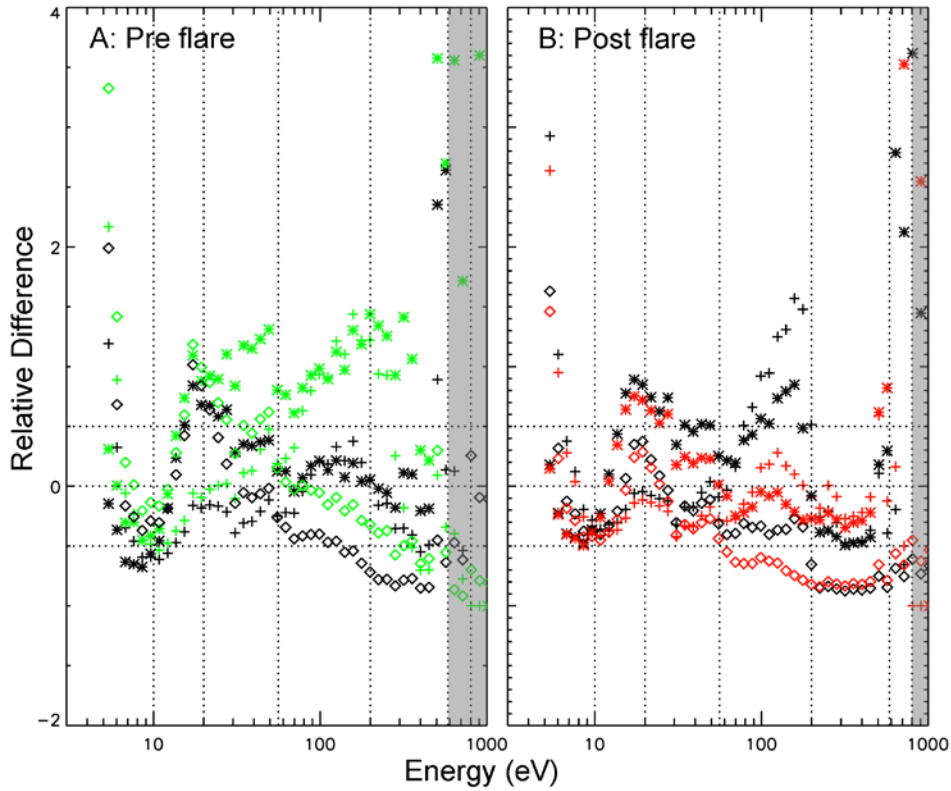
Figure 4. Relative difference between observed and modeled electron flux values as a function of energy shown in Figure 3. Relative difference = (modeled – observed values) / observed values. The colors and symbols are the same as those used in Figure 3. Horizontal dotted lines are shown at -0.5, 0, and +0.5. Vertical dotted lines are shown at 10, 20, 56, 200, 585 and 800 eV. The grey areas indicated where the signal to noise ratio of the observations is less than 3.
