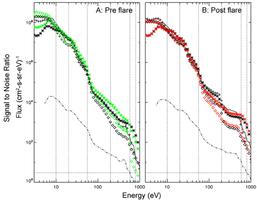
Figure 3: Observed (black lines) and modeled (symbols) electron fluxes for the times given in Table 1. In panel A black symbols show model results using the FISM-M L3D spectrum and green symbols show model results using the HESSR daily irradiance spectrum. In panel B the black symbols are from model runs using the L3F model and the red symbols are the L3FR model.
