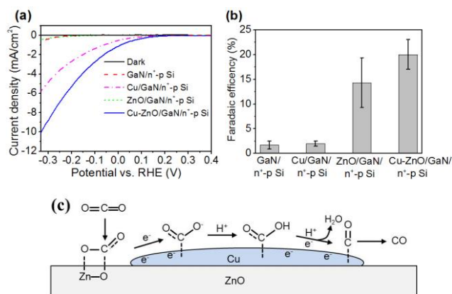
Figure 4. (a) J-V curves. (b) FEs for CO at -0.33 V vs. RHE. (c) Proposed reaction mechanism for the photoreduction of CO 2 to produce CO on Cu-ZnO dual co-catalysts.
