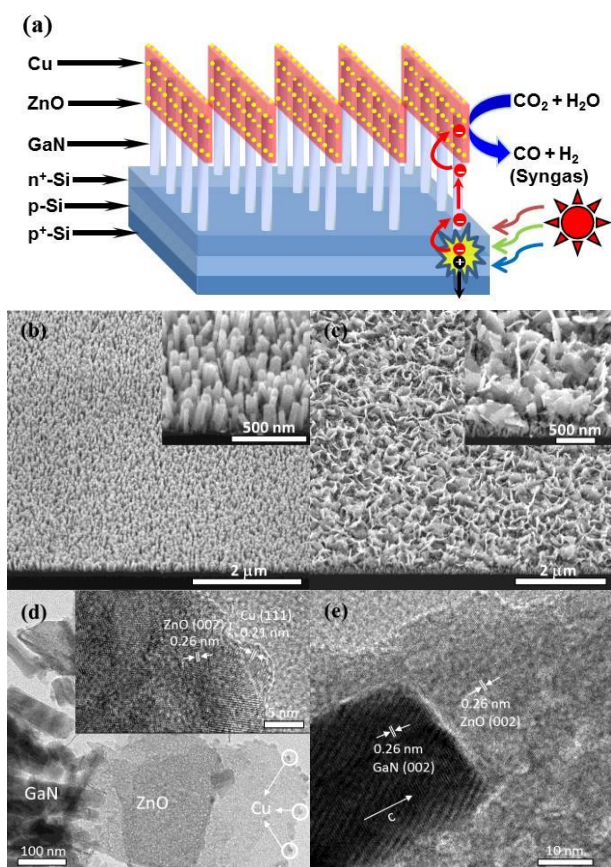
Figure 1. (a) Schematic illustration of Cu-ZnO/GaN/n + -p Si photocathode (not drawn to scale). (b) SEM images of GaN nanowires grown on a p-n junction Si. (c) SEM and (d) TEM images of Cu-ZnO decorated GaN nanowires. Inset of (d), and (e): HRTEM images of the interface between Cu, ZnO and GaN.
