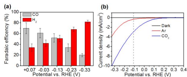
Figure 2. (a) FEs for CO (grey bars) and H 2 (red bars) of Cu-ZnO/GaN/n + -p Si photocathode as a function of potential in CO 2 -saturated 0.5 M KHCO 3 solution (pH 8). (b) J-V curves in Ar and CO 2 -saturated 0.5 M KHCO 3 solution. The dashed line shows the standard potential for CO 2 reduction to CO at pH 8.
