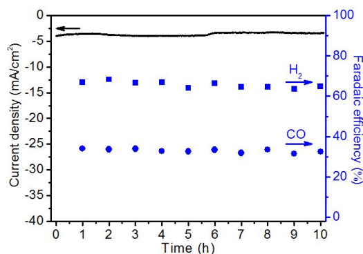
Figure 3. Chronoamperometry data and FEs for CO and H 2 of Cu-ZnO/GaN/n + -p Si photocathode at -0.23 V vs. RHE.
