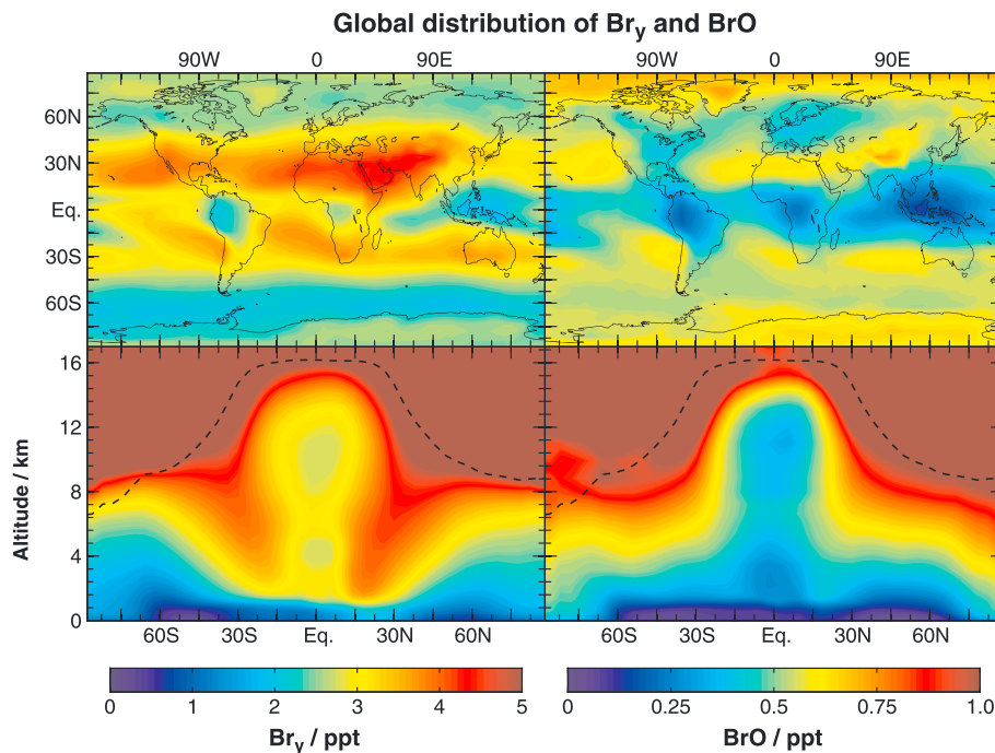
Figure 2. Simulated annual mean global distributions of tropospheric \text{Br}_y and \text{BrO} . Multiply \text{BrO} concentrations by a factor of 2 for daytime values (this approximation is not valid at high latitudes during winter and summer). (top row) Mean tropospheric mixing ratios. (bottom row) Zonal mean mixing ratios as a function of altitude and latitude. The tropopause is shown as dashed line. Results are for the simulation not including dehalogenation of SSA (simulation A).
