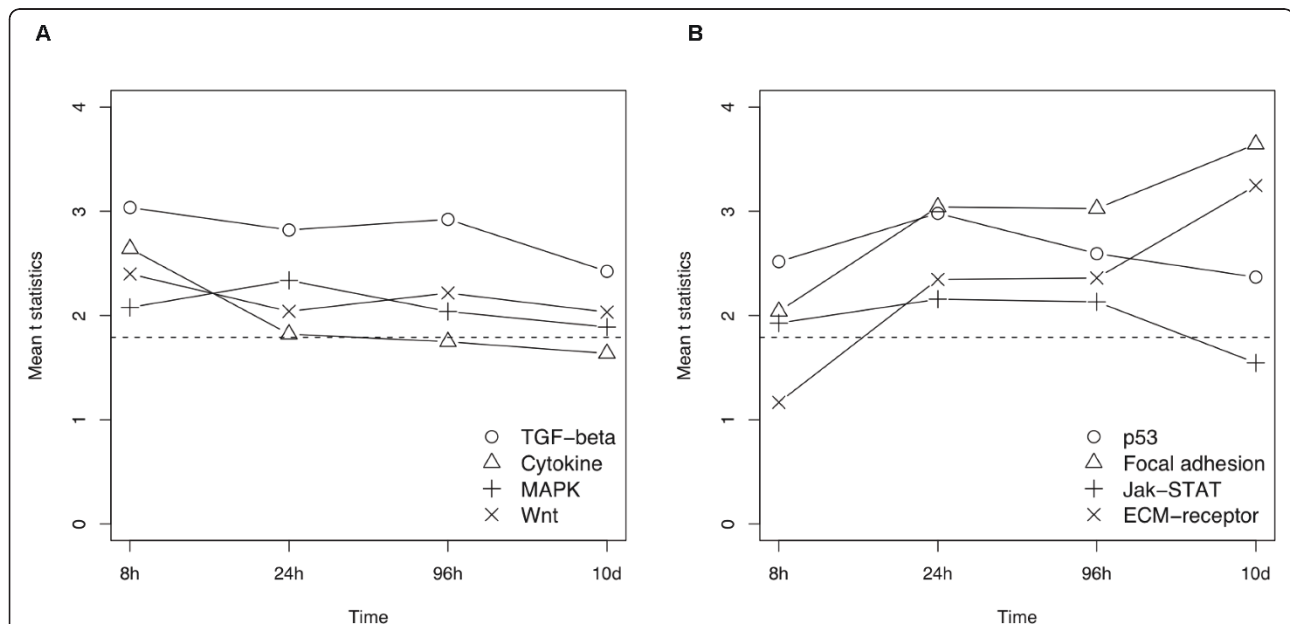
Figure 2 The expression perturbation patterns induced by BMP6 treatment in eight significant KEGG pathways. These pathways are consistently significantly differentially expressed or near so based on GAGE. The mean t-statistics from multiple one-on-one comparisons between the two sample conditions is used as overall perturbation magnitude for each pathway. Perturbation magnitude here is defined as the absolute value of both positive and negative gene expression changes without considering the actual perturbation direction. The dashed line indicates a t-statistic of 1.79, which roughly corresponds to p = 0.01 for 8-96 h or 0.001 for 10 d. Panel (a) and (b) are divided only for visual clarity.
