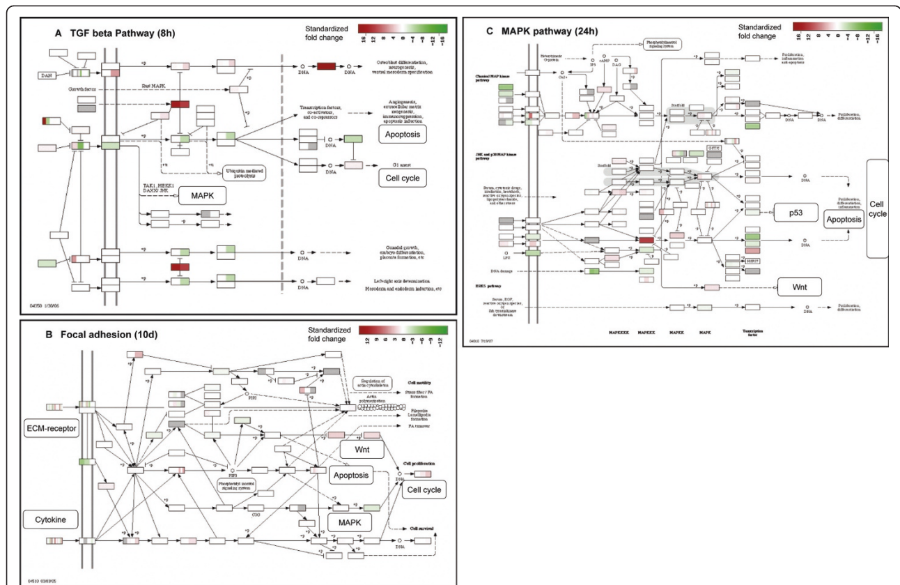
Figure 3 Gene expression fold changes induced by BMP6 in three representative significant KEGG pathways. Each pathway shown is at its most perturbed time point: (a) TGF-beta signaling pathway at 8h; (b) Focal adhesion at 10d; (c) MAPK signaling pathway at 24h. Gene expression level fold changes are standardized over the standard deviation of fold changes for all genes. The standardized fold changes are visualized by using KEGGanim web tool [56]. Note that one KEGG node may correspond to multiple closely related genes with the same function. Relevant other pathways are magnified locally for better view. Gene names are intentionally omitted by KEGGanim for clear view of the gene expression changes in pseudo-color.
