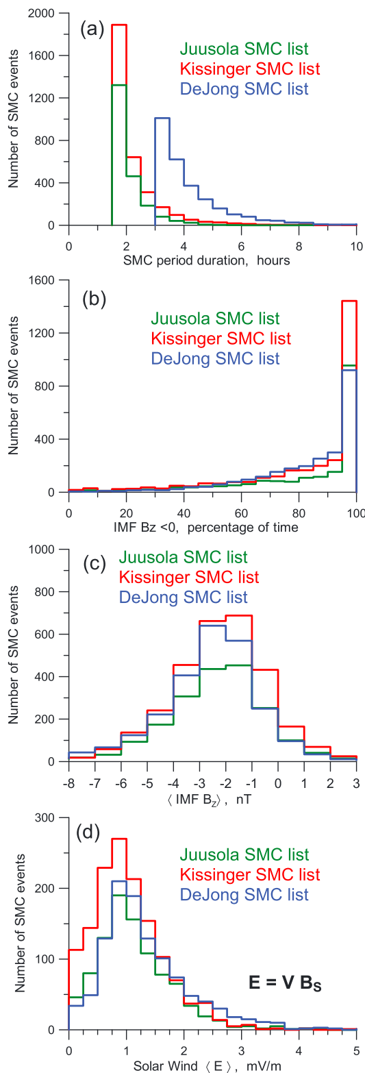
Figure 1. Properties of SMC events for three SMC lists. (a) SMC event duration. (b) Percentage of time when IMF B_z is negative. (c) Mean IMF B_z . (d) Mean solar wind electric field.
