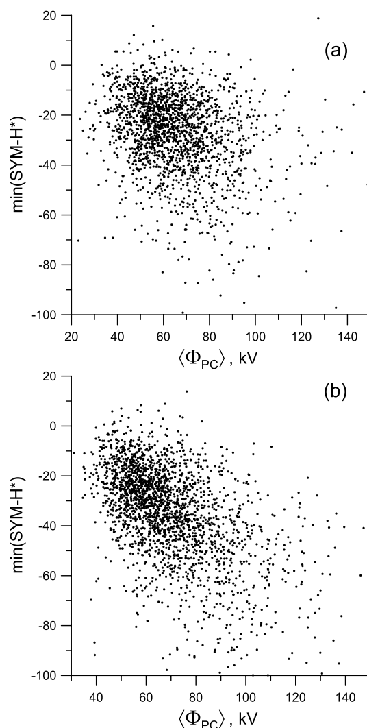
Figure 9. Minimum \text{SYM-H}^* versus mean polar cap potential for the SMC events. (a) Juusola and (b) DeJong lists of events.
