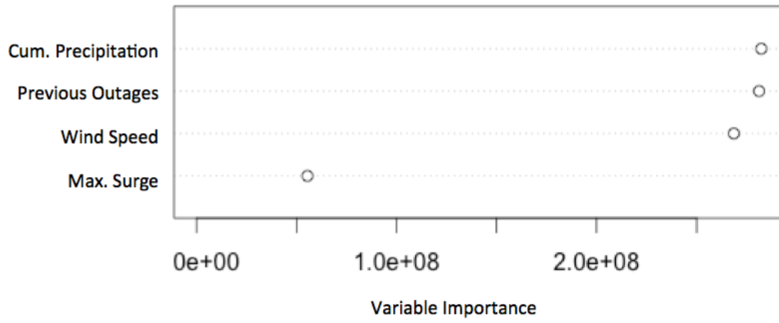
Fig. 4 Variable Importance, reduced covariate set
