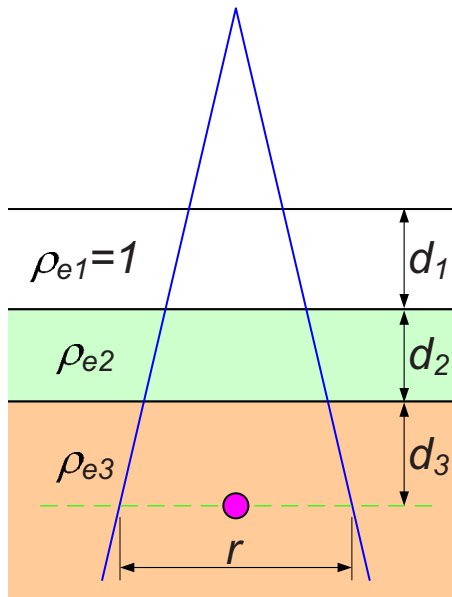
FIG. 2. Photon dose calculation to a point in a heterogeneous phantom. The first layer of material is assumed to be water equivalent.
