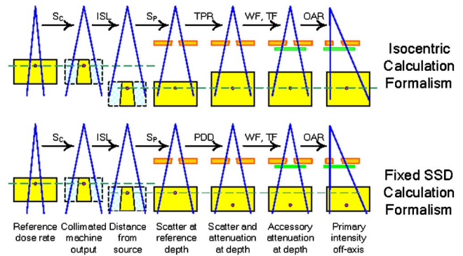
FIG. 1. Development of Eqs. (A2) and (A3) for photon dose calculation to a point in a water equivalent slab phantom. Successive application of factors transforms the dose rate from the reference condition to the conditions of treatment geometry and depth. Steps in the calculation where the phantom scatter differs from the irradiating field size during the application of S_c and ISL factors are indicated by sectioning the phantom, where the portion enclosed by the solid lines signifies the inclusion of reference field size phantom scatter. The solid circle represents the position of the calculation point, while the dashed line crossing several phantoms indicates changes in the point distance from the source.
