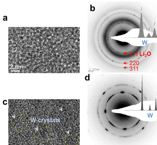
Figure S1 , TEM, high resolution TEM and electron diffraction patterns of fully converted phase (a-b) and beam annealed phase (c-d). Insets in (b) and (d) are simulated diffraction intensity profiles of polycrystalline W. The circles and arrows in (c) indicate the W nanocrystals formed after intense electron beam irradiation.
