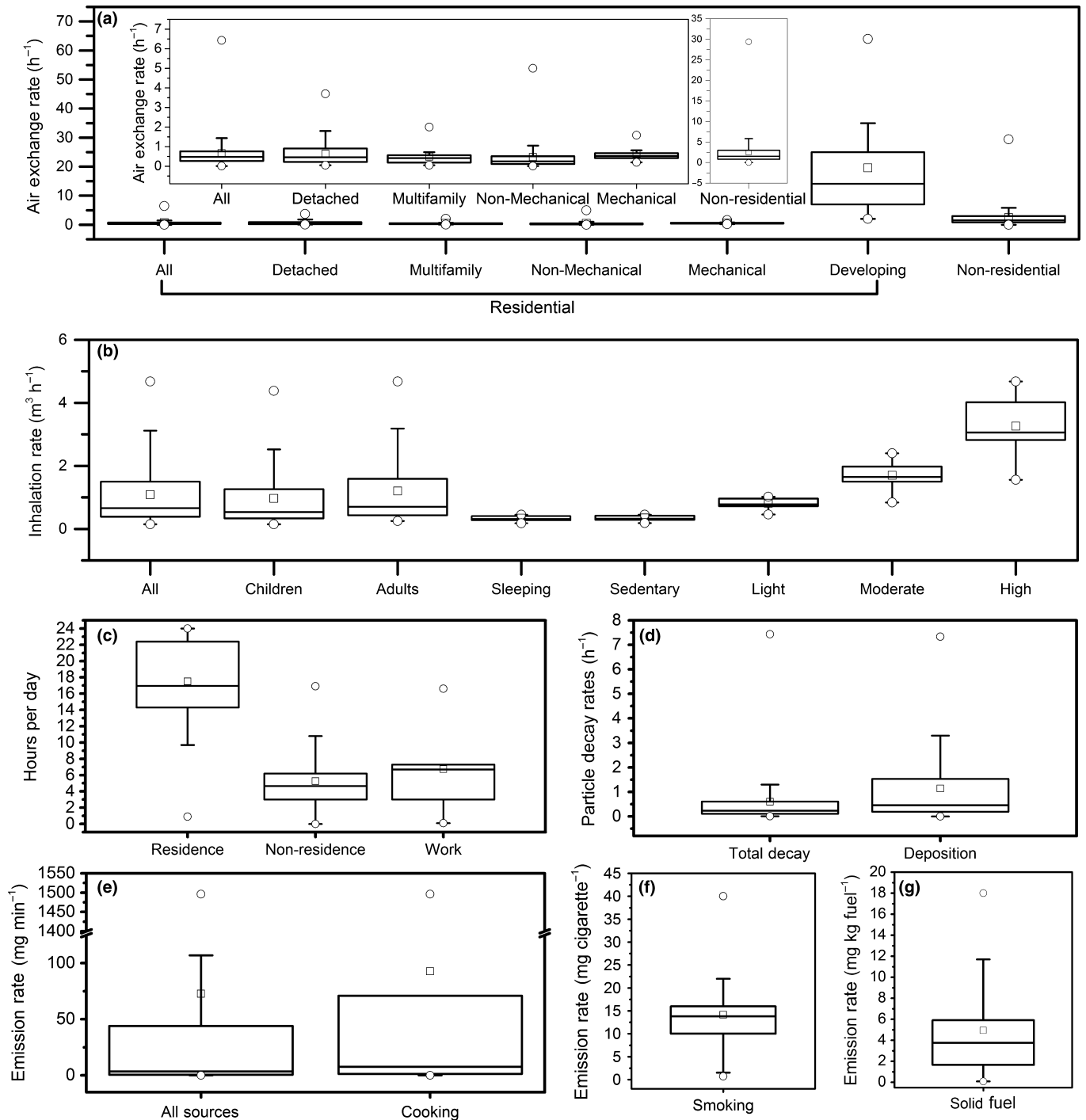
Fig. 2 Summary of measured or modeled values describing the parameter of interest for (a) building air exchange rates, (b) inhalation rates, (c) time-activity factors, (d) particle decay rates, and (e–g) indoor PM 2.5 source strengths reported in the literature. For all plots, the boxes indicate the 25th percentile, median, and 75th percentile. Minimum and maximum values are indicated with circles and mean values are indicated with squares. (a) Air exchange rates shown are for all homes combined (excluding homes in developing nations) ('All') and separately for detached/single-family homes ('Detached'), multifamily homes ('Multifamily'), homes without mechanical ventilation (i.e., infiltration and natural ventilation) ('Non-mechanical'), mechanically ventilated homes ('Mechanical'), homes in developing countries ('Developing'), and non-residential buildings ('Non-residential'). (b) Inhalation rates are for all measurements combined ('All'), and separately for adults (>21 years), children (<=21 years), and activity level (sleeping, sedentary, light, moderate, and high). (c) Time-activity factors include hours per day spent in the residence ('Residence'), in other indoor locations ('Non-residence'), and at work ('Work'). (d) Particle decay rates are given for all particle loss mechanisms combined ('Total Decay') and for losses driven only by deposition. (e) Source emissions are given for common indoor PM 2.5 sources including cooking, cleaning, smoking, and various appliances combined, excluding the combustion of solid fuels ('All Sources'). (e), (f), and (g) Source emissions are also illustrated for cooking, smoking, and solid fuel combustion separately. The total number of observations for each parameter is shown in Figure 1 and all underlying data are provided in the Supporting Information
