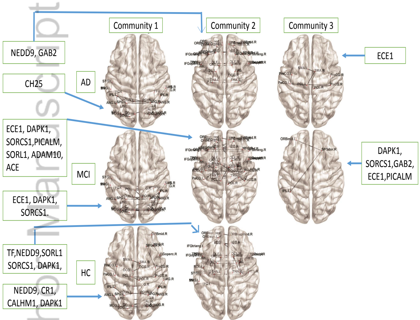
Figure 3. Functional modules or communities for AD, MCI and HC groups, along with important genes. The arrows relate the sub-networks to the significant genes influencing them. Each such gene can influence one or more connections in the functional modules, as well as one or more phenotypes in that module.
