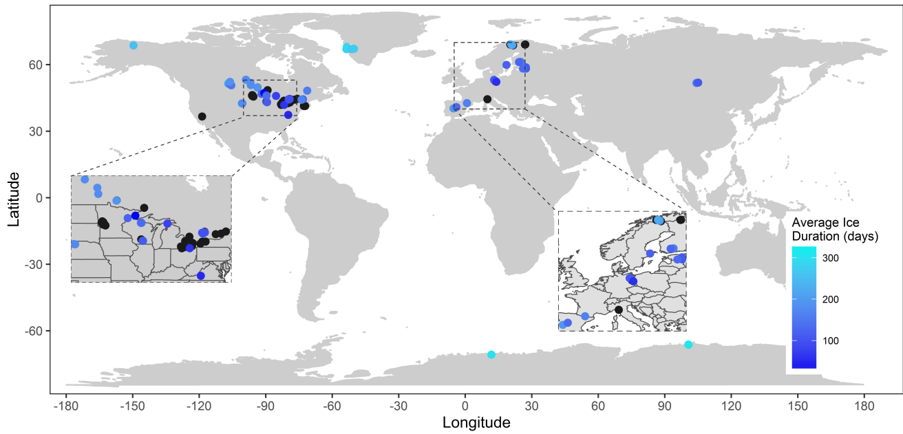
Figure S3. Map of sampling stations in the full synthesis of primary data. Stations are colored by average ice duration (for unique sample stations across all sampled winters); stations with no ice duration information provided are colored black.
