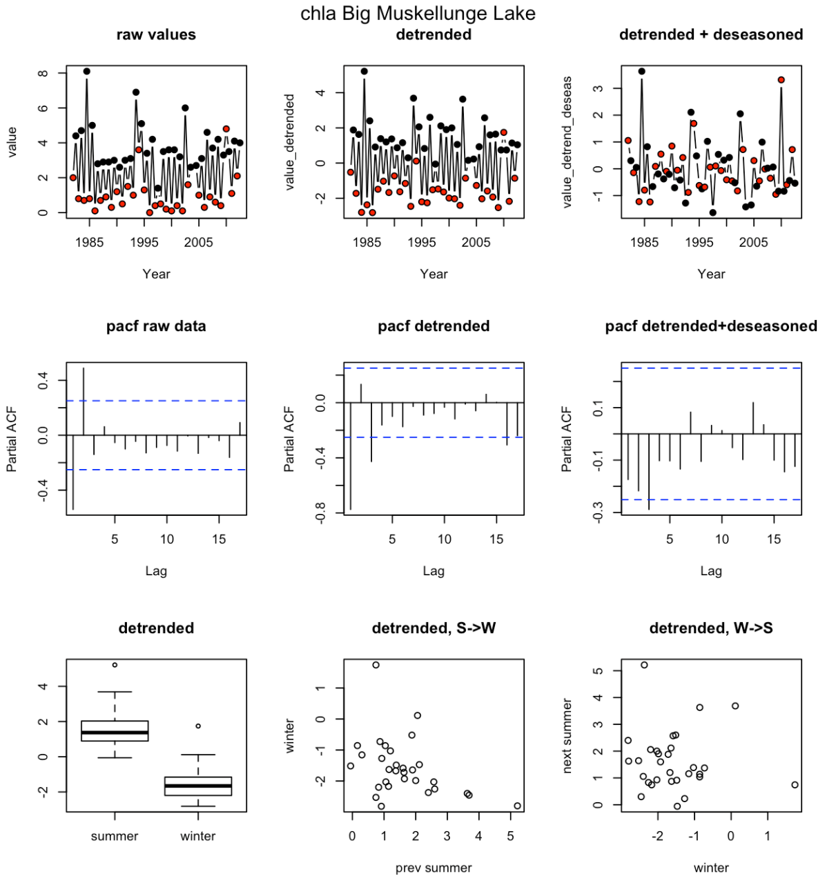
Figure S4. Example time series for chl a in Big Muskellunge Lake, WI (USA) including raw data, moving-average detrended data, winter-summer differences, autocorrelation structure, and winter-summer correlation plots. In top row, winter values are red. The detrended time series were used to examine winter-summer differences within lakes, and winter-summer correlations within lakes. Summary statistics for this time series, and all others that we examined, are in Table S5.
