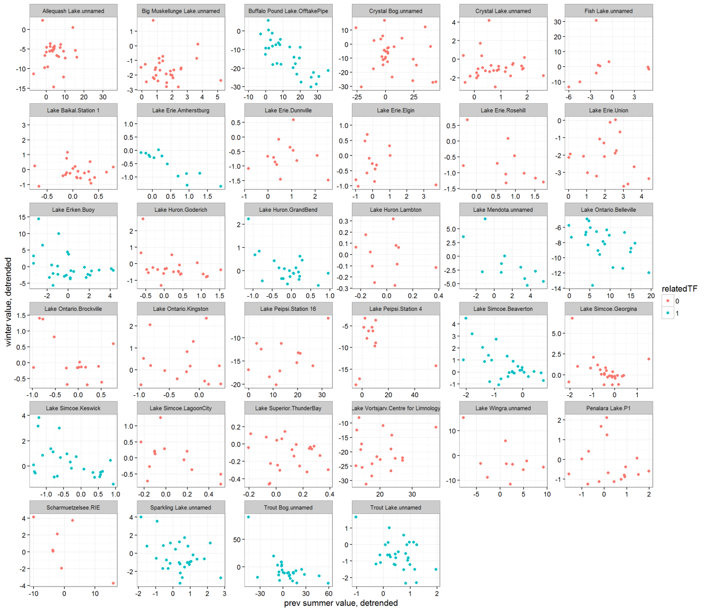
Figure S5. Example correlations between winter and the previous summer (SW) for chl a (moving average detrended) at stations that had longer-term time series. Blue dots indicate time series where winter and summer were related according to AICc selection, meaning that inclusion of a winter~summer slope was an improvement over the intercept only model ( \Delta AICc \geq 2 ).
