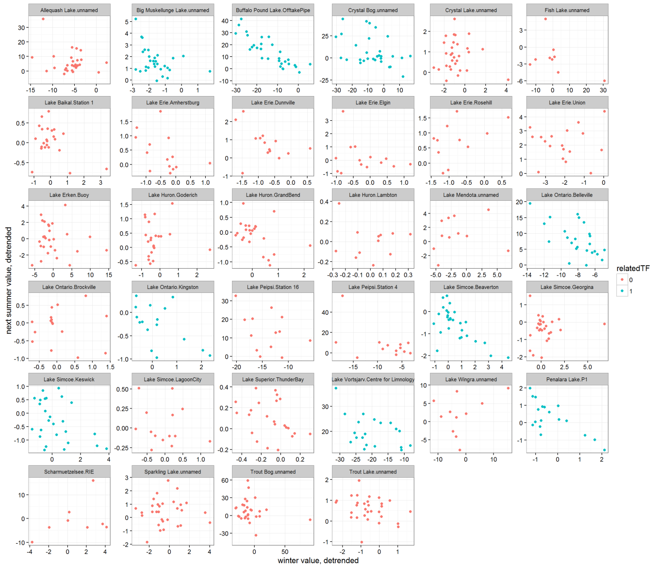
Figure S6. Example correlations between winter and the following summer (WS) for chl a (moving average detrended) at stations that had longer-term time series. Blue dots indicate time series where winter and summer were related according to AICc selection, meaning that inclusion of a summer~winter slope was an improvement over the intercept only model ( \Delta AICc \geq 2 ).
