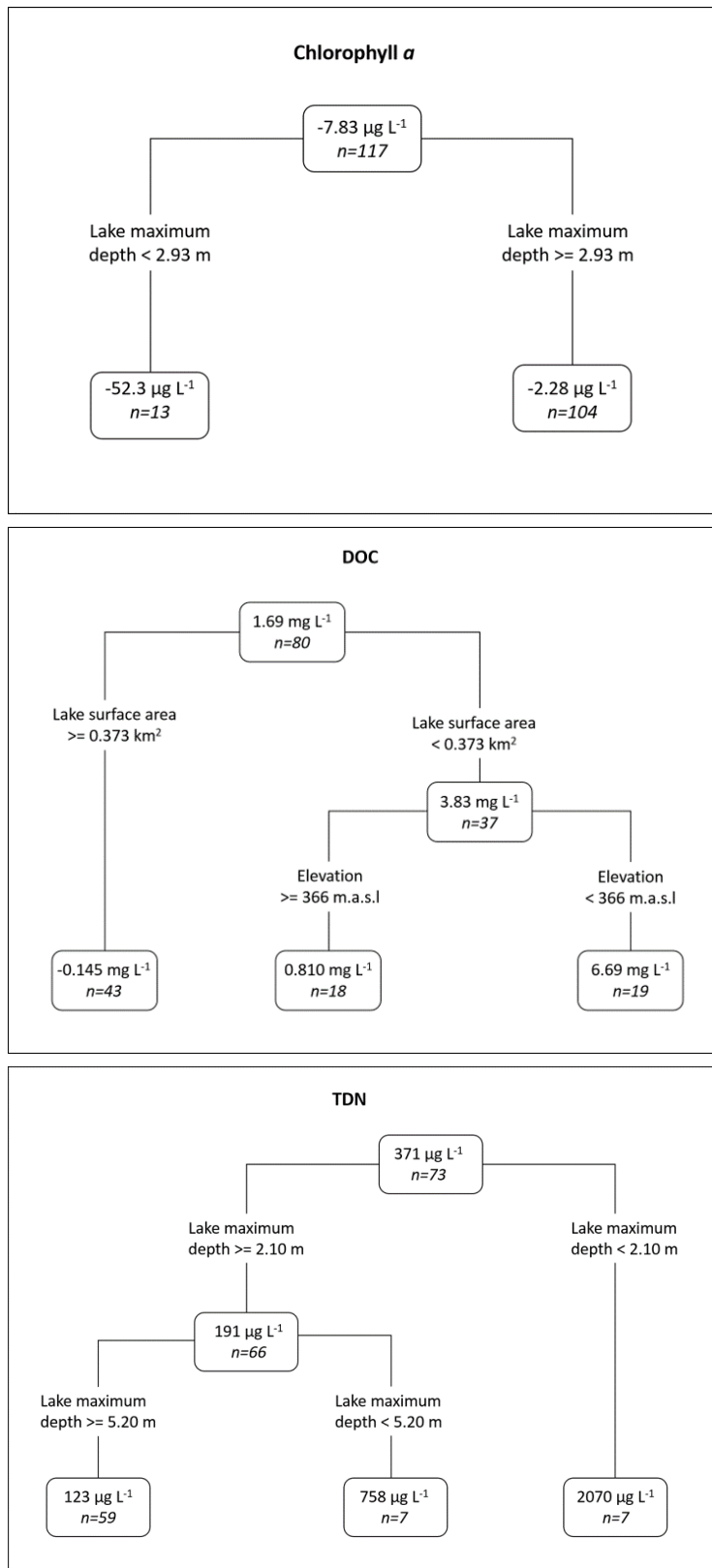
Figure S7. Regression tree results for chl a ( R^2=0.330 ), DOC ( R^2=0.538 ), and TDN ( R^2=0.722 ), showing differences between winter and summer (winter minus summer) for multiple lake types. Candidate covariates included lake surface area, maximum lake depth, elevation, and latitude (absolute).
