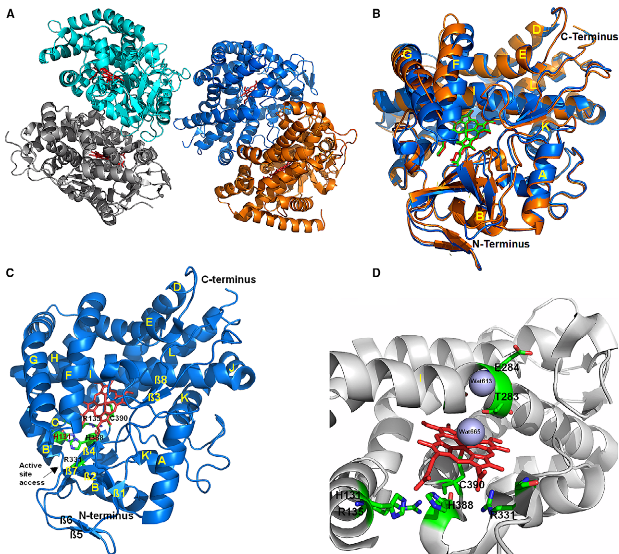
Fig. 1. Crystal structure of CYP260A1. A. The four molecules, chain A (cyan), chain B (orange), chain C (blue), and chain D (gray) were found in the asymmetric unit of the substrate-free crystal structure of CYP260A1. B. The superimposed structure of the open conformation of chain B (orange) and the close conformation of chain C (blue) is shown. C. The 12 \alpha -helices (A-helix to L-helix) and 8 \beta -strands ( \beta 1– \beta 8) in the chain C of CYP260A1 is shown. D. The active site residues of CYP260A1 with the two coordinated water molecules (W613 and W665) (light blue spheres) are shown.
