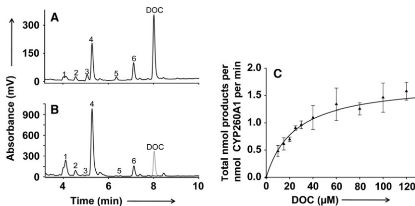
Fig. 2. LC-MS chromatogram of the in vitro (A) and an E. coli based whole-cell conversion (B) of DOC by CYP260A1. The activity was reconstituted with the heterologous redox partners Adx and AdR. The ratio of CYP260A1 : Adx : AdR was 1 : 10 : 3. The numbers indicated in the chromatogram represent the product peaks for the conversion of DOC. The major product corresponding to peak 4 was identified as 1\alpha -hydroxylated-11-DOC. C. Kinetic study of DOC conversion. The error bar in the figures represents the standard deviation of 3–5 independent measurements.
