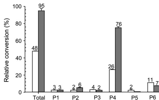
Fig. 4. Comparison of the steady-state in vitro conversion of DOC by wild-type CYP260A1 (blank bar) and S326N (gray bar). The products obtained upon the conversion of DOC by the P450s are shown as the product peaks P1-P6. The error bar in the figures represents the standard deviation of five independent measurements. The activity was reconstituted with the heterologous redox partners Adx and AdR. The ratio of CYP260A1 : Adx : AdR was 1 : 20 : 3. The major product corresponding to peak 4 was identified as 1 \alpha -hydroxylated-DOC.
