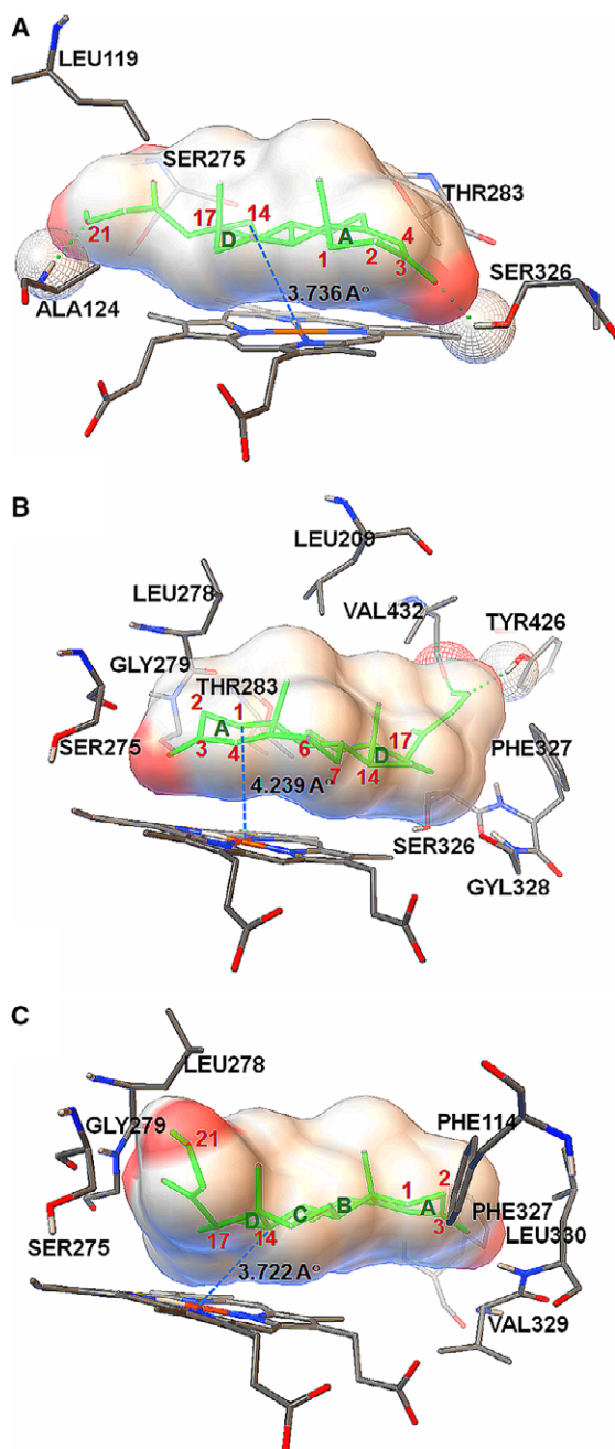
Fig. 3. Docking conformations of DOC into the crystal structure of CYP260A1. The docking poses II (A), III (B), and IV (C) are shown. The default program of Autodock version 4.2 was used. The ligand steroid is shown as green stick, surrounded by a molecular surface. The surface is colored with atomic colors in regions that contact the receptor, and gray in regions that are not in contact. The carbon surface is shown in red. The hydrogen bonds (in a wireframe-sphere) are shown in green dotted lines. The most possible hydroxylating C-atoms from the heme-center (blue dashed line) to the DOC are shown. The steroidal rings are represented by A to D, and the most feasible hydroxylating positions identified by P450s are numbered.
