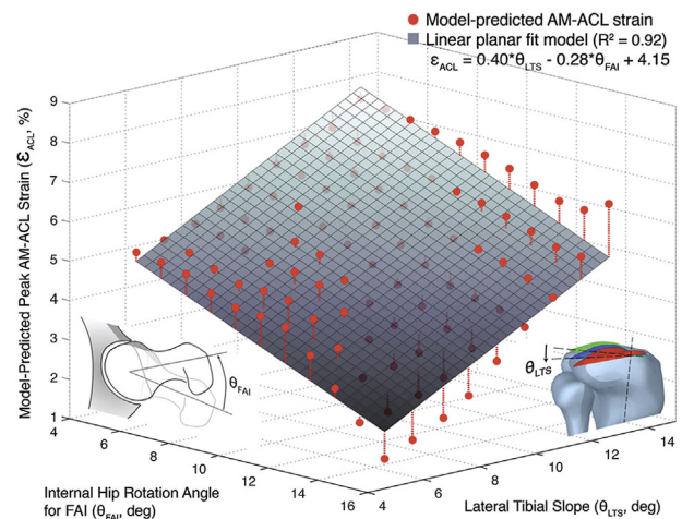
Figure 13. In silico model predictions for peak anteromedial bundle–anterior cruciate ligament (AM-ACL) strain during a simulated jump landing: As the available range of hip internal rotation is reduced, the peak AM-ACL strain in the knee increases. The linear planar fit model (shown as the gray plane) demonstrates how peak AM-ACL strain is predicted to be a function of both available axial hip range of motion and lateral tibial slope. Reproduced from Bedi et al. 25
