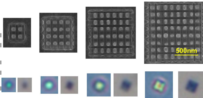
Figure 4 The SEM images with different pixel size and their corresponding photo images taken by digital imaging microscopy. The pixel size from left to right: 2×2 array, 4×4 array, 6×6 array, 8×8 array. The photo images of each group were taken in transmission and reflection respectively, from left to right.
