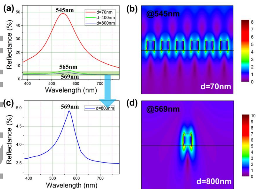
Figure 3 (a) The reflectance curves of the structure for the reflective green filter with three different inter-patch distances d=70\text{nm} , 400\text{nm} , 800\text{nm} . (b) The electric field distribution of the patch array structure with the inter-patch distance d=70\text{nm} for the peak reflectance wavelength \lambda=545\text{nm} . (c) The magnified reflectance curve of the patch array structure with the inter-patch distance d=800\text{nm} . (d) The electric field distribution of the patch array structure with the inter-patch distance d=800\text{nm} for the peak reflectance wavelength \lambda=569\text{nm} .
