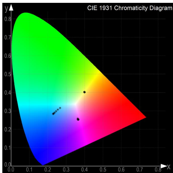
Figure S1 The CIE 1931 chromaticity coordinates of three transmissive primary color filters composed of ultrathin metallic nanocuboid array for the unpolarized light at the incidence angles of 0^\circ , 10^\circ , 20^\circ , 30^\circ , 40^\circ , 50^\circ , 60^\circ .
