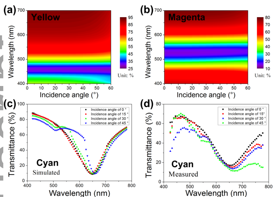
Figure 2 (a) Simulated transmittance of the transmissive yellow filter of the nanocuboid pattern as a function of wavelength and the angle of incidence for average polarization. (b) Simulated transmittance of the transmissive magenta filter of the nanocuboid pattern as a function of wavelength and the angle of incidence for average polarization. (c) Simulated transmittance curves of the transmissive cyan filter of the nanodisk pattern at different incidence angles for average polarization. (d) Measured transmittance curves of the transmissive cyan filter at different incidence angles for average polarization.
