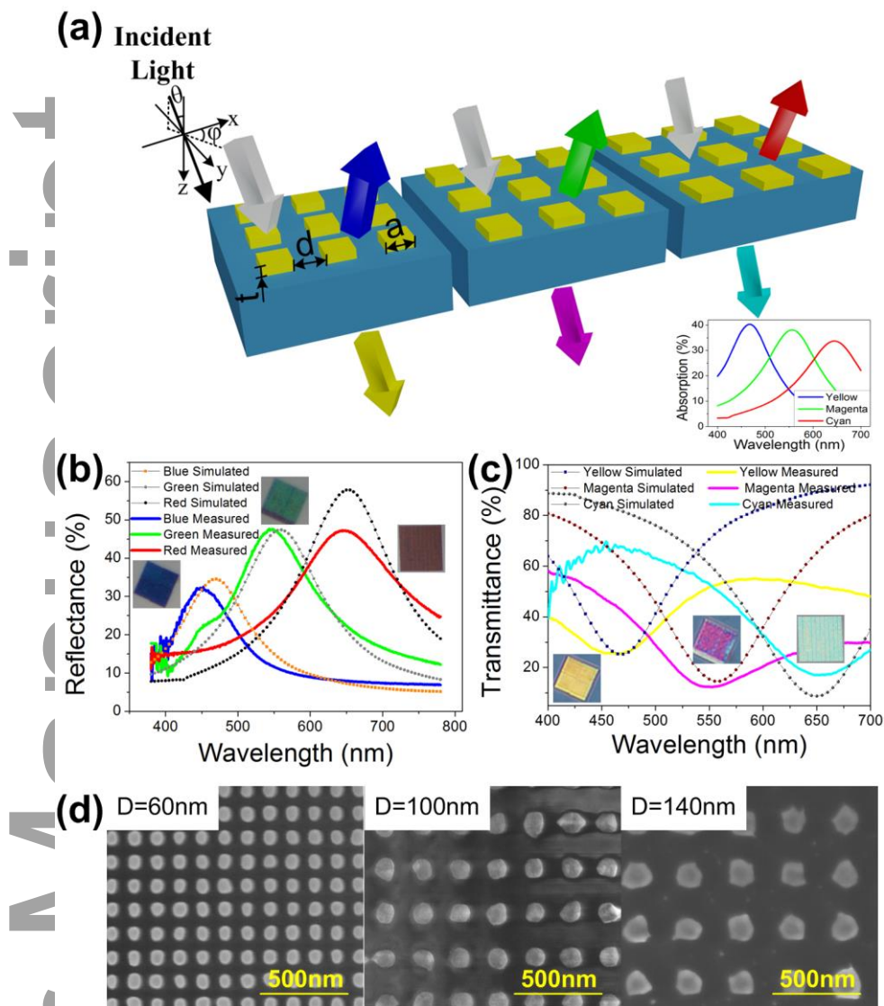
Figure 1 (a) The schematic geometry of the angle robust reflection/transmission plasmonic filters using ultrathin metal patch array structure. The calculated absorption of the proposed filters is shown in the inset. (b) The simulated and measured reflectance curves of the reflective RGB filters of
