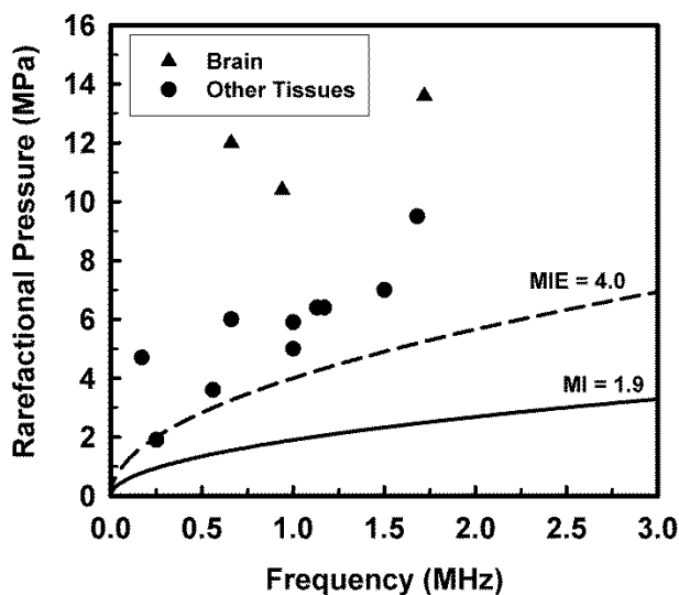
Figure 3. Best estimates of in situ rarefactional pressure shown in Table 1. Triangles and circles indicate values for brain and all other tissues, respectively. Curves delineate pressures calculated for the maximum value of the MI in the FDA’s guidance for track 3 devices (solid curve, labeled MI = 1.9) and an effective mechanical index of 4.0 (dashed curve, labeled MIE = 4.0).
