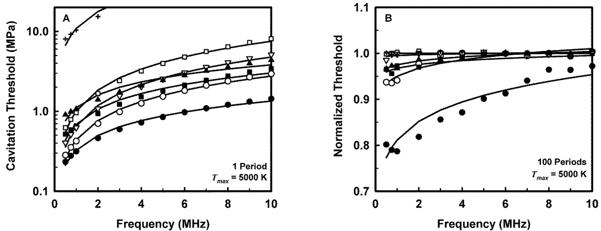
Figure 1. Theoretical thresholds for inertial cavitation of optimally sized air bubbles in materials with various viscoelastic properties for a threshold criterion of T_{max} = 5000 K. A , Thresholds calculated assuming pressure durations of 1 acoustic period. B , Normalized (by data from 1 acoustic period in A ) thresholds for inertial cavitation in each material at a pulse length of 100 acoustic periods. Curves are the best fits of P_t = Bf_c^n to the numerical data for water ( \bullet ) blood ( \circ ), heart ( \square ), kidney ( \blacksquare ), liver ( \nabla ), skeletal muscle ( \blacktriangle ), and skin ( + ). The average value for n (the power of frequency) for the combined curves was 0.75. 15
