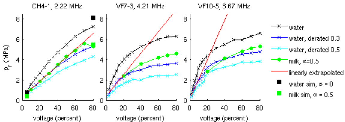
Figure 2. Peak rarefactional pressure ( p_r ) values measured in water (X) and derated by: 0.3 \text{ dB cm}^{-1} \text{ MHz}^{-1} (X), and 0.5 \text{ dB cm}^{-1} \text{ MHz}^{-1} (X); p_r derated water measurements linearly extrapolated from small signal values (—, see appendix A); p_r estimated using a grid of source pressure measurements in water and modeling nonlinear propagation using the 3D KZK model with numerical solution methods described previously 44 (CH4-1 only) assuming propagation through water (■) and milk (■); as well as in situ p_r measurements made in an evaporated milk solution (●, measured attenuation = 0.5 \text{ dB cm}^{-1} \text{ MHz}^{-1} ). Note that derating water values by 0.3 \text{ dB cm}^{-1} \text{ MHz}^{-1} provides reasonable agreement with the milk measurements (to within 20% for all transducers); however, derating water values by the actual measured attenuation of the milk ( 0.5 \text{ dB cm}^{-1} \text{ MHz}^{-1} ) leads to considerable underestimation of the milk measurements. Additionally, the linear extrapolation approach considerably overestimates the milk measurements for the higher frequency transducers, whereas the source pressure + nonlinear simulation approach (black squares and green squares, left plot) is in good agreement with the milk measurements. Each array transducer was focused with an F/2 lateral focal configuration concurrent with its fixed elevation focus.
